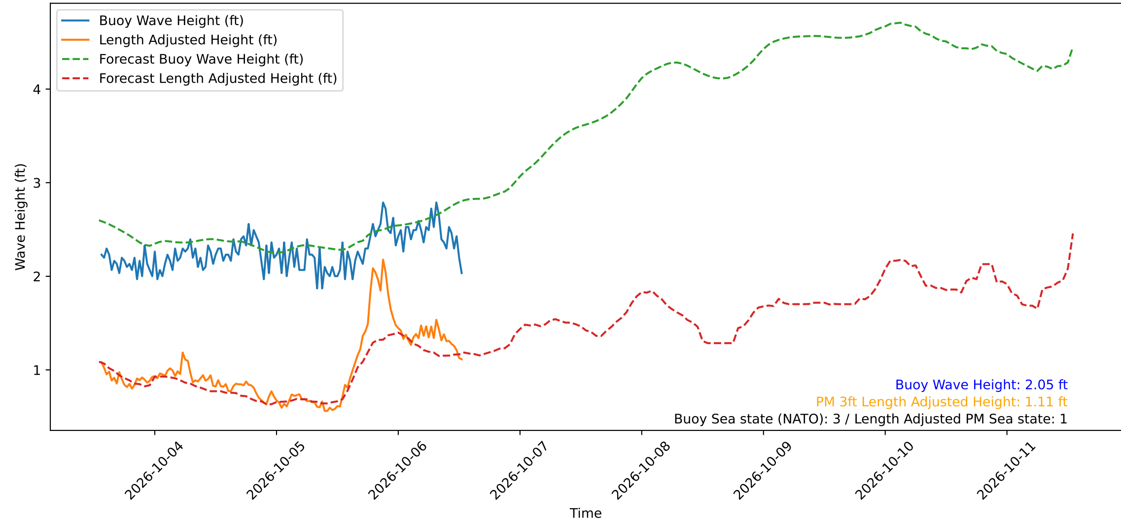
Wave Heights over Time for Oceanside Harbor at 2026-10-06 13:20:29
