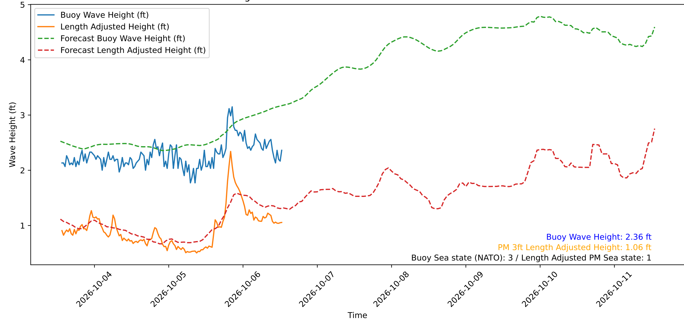
Wave Heights over Time for Green Beach at 2026-10-06 13:21:15
