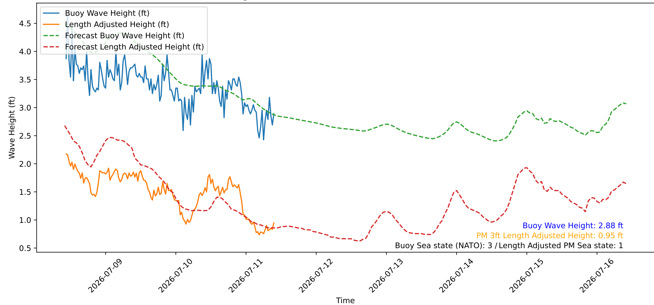
Wave Heights over Time for Red Beach at 2026-07-11 10:10:45
