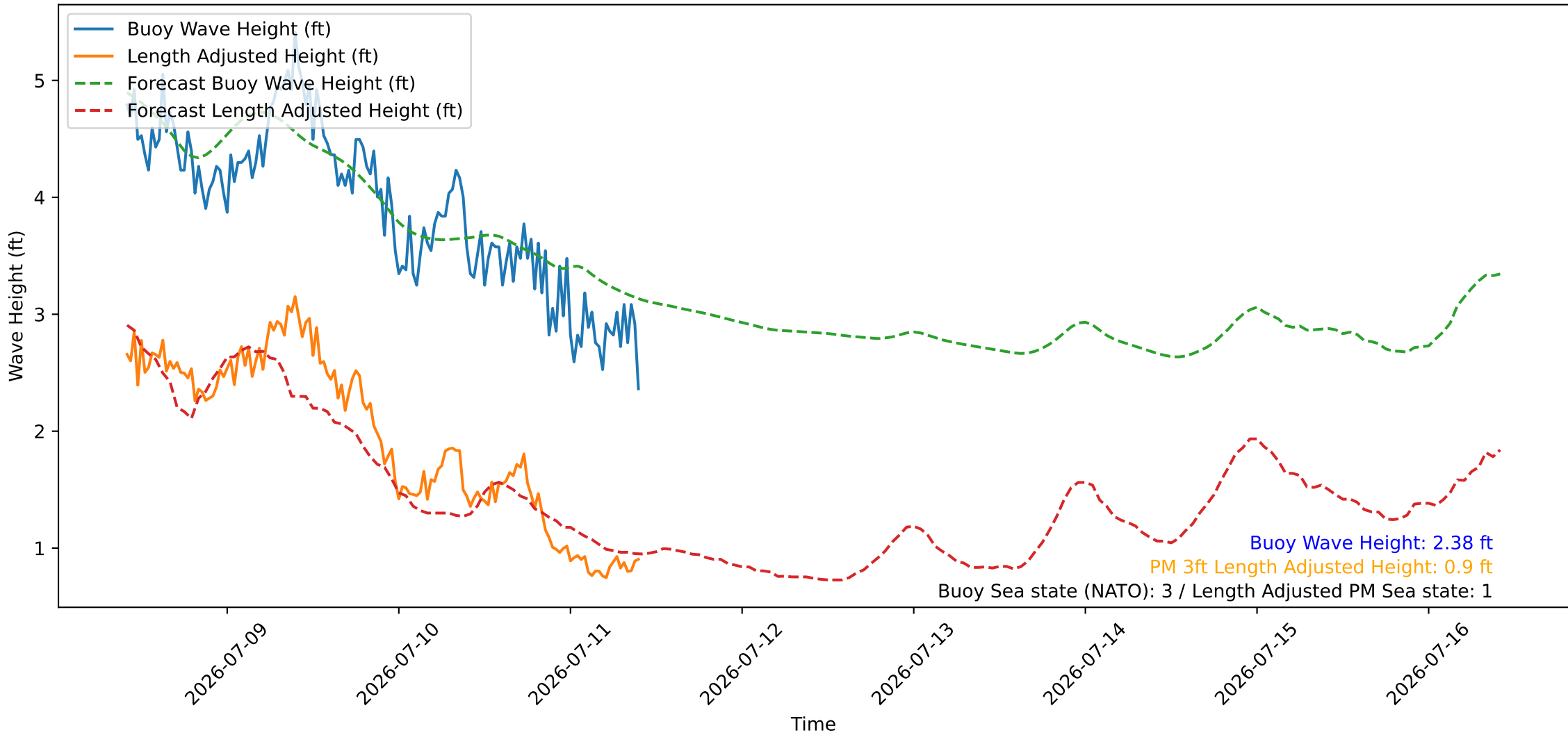
Wave Heights over Time for Oceanside Harbor at 2026-07-11 10:10:26
