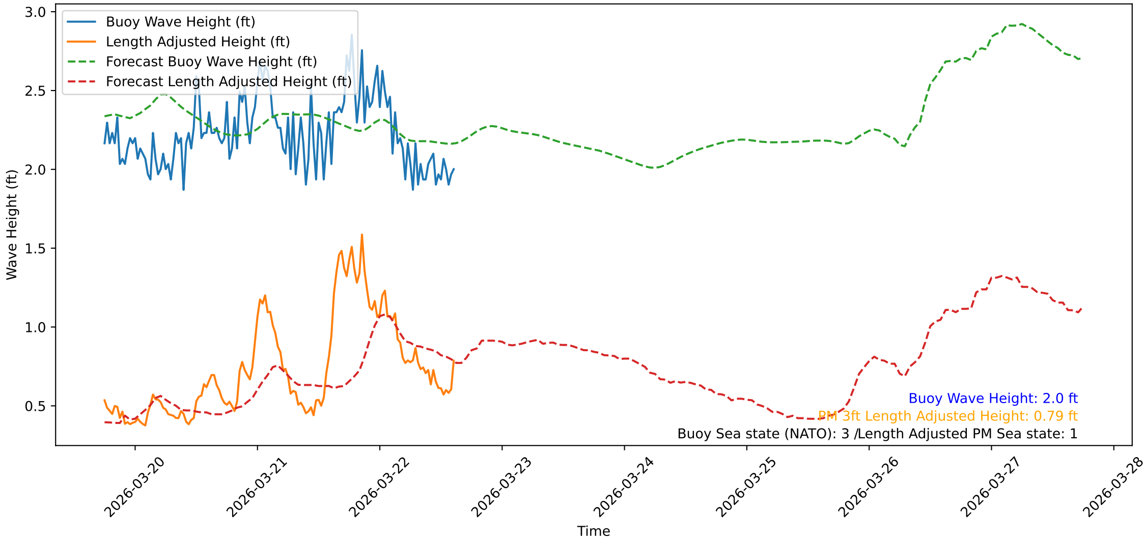
Wave Heights over Time for Red Beach at 2026-03-22 17:40:47
