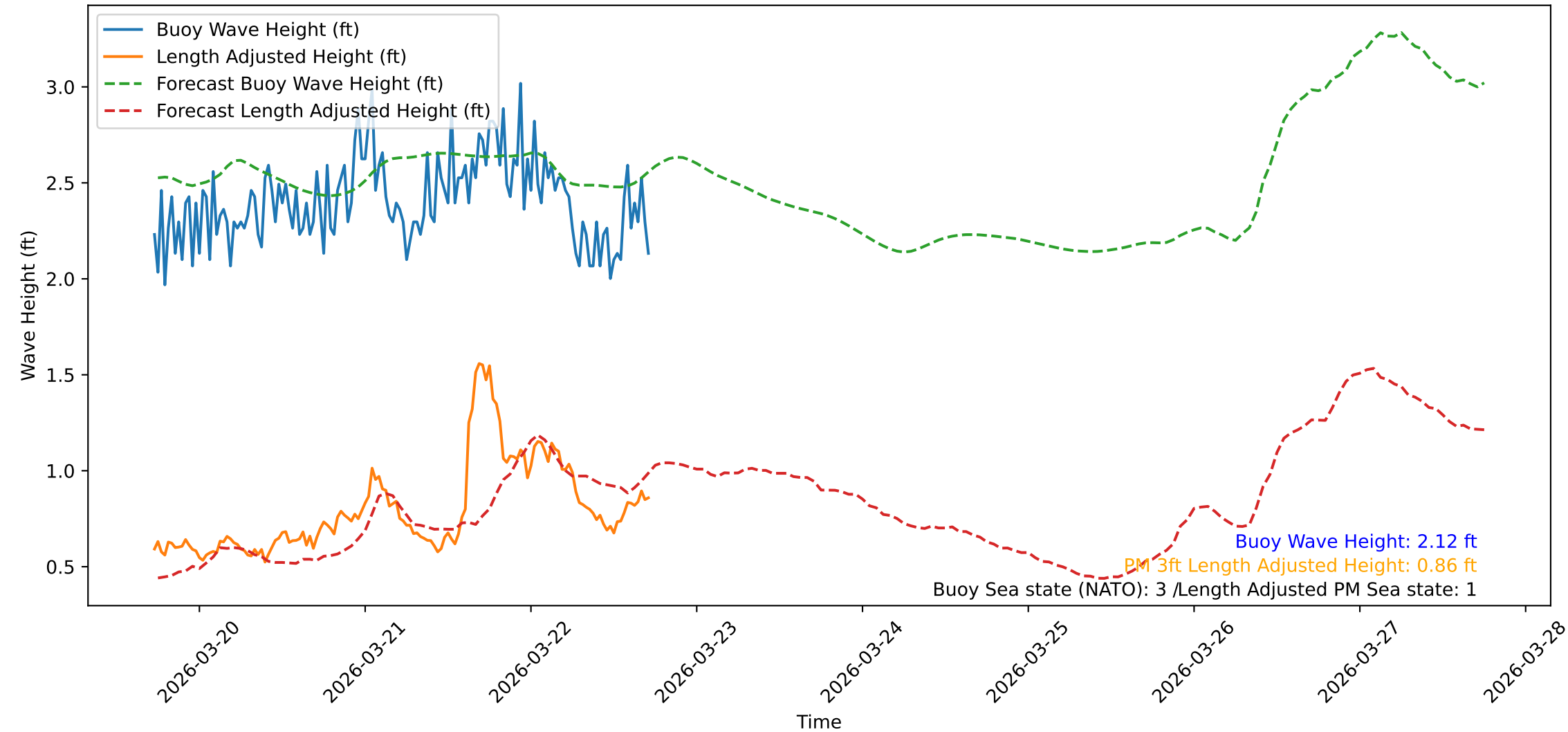
Wave Heights over Time for Oceanside Harbor at 2026-03-22 17:40:32
