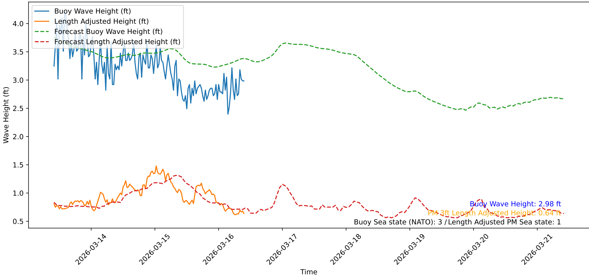
Wave Heights over Time for Oceanside Harbor at 2026-03-16 10:10:42
