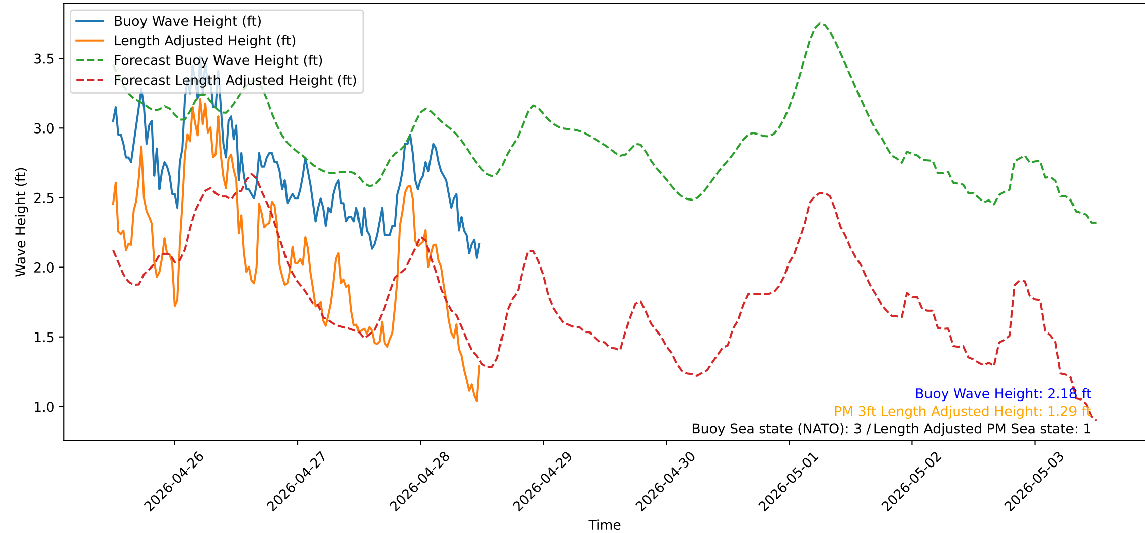
Wave Heights over Time for Green Beach at 2026-04-28 12:11:27
