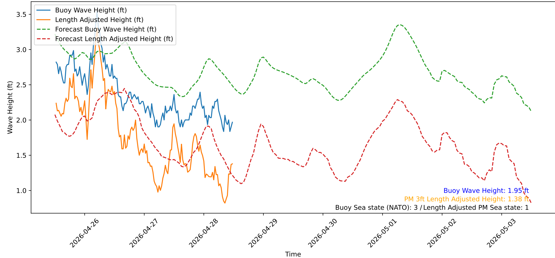
Wave Heights over Time for Red Beach at 2026-04-28 12:10:50
