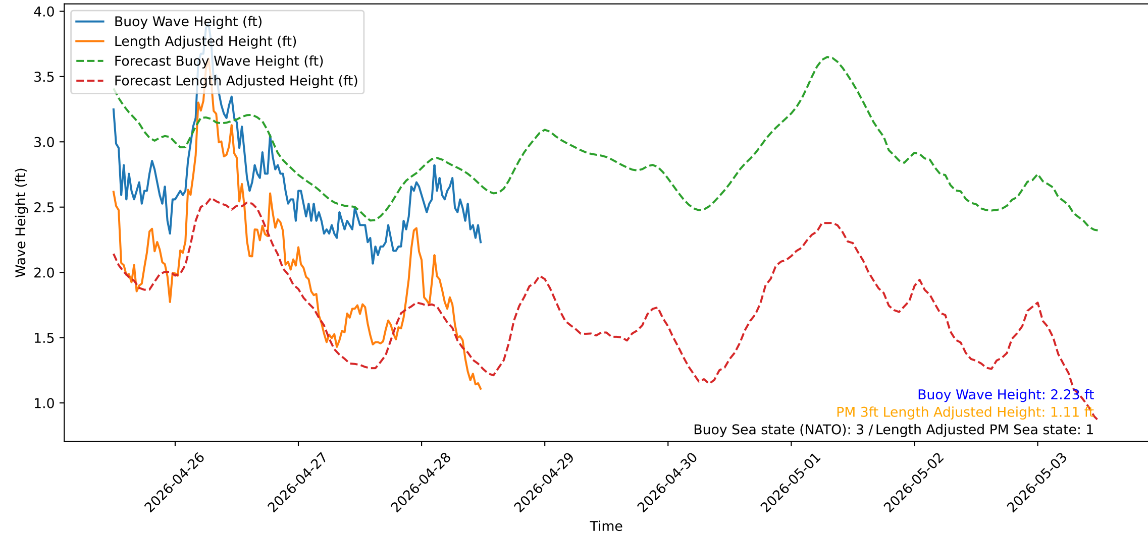
Wave Heights over Time for Oceanside Harbor at 2026-04-28 12:10:31
