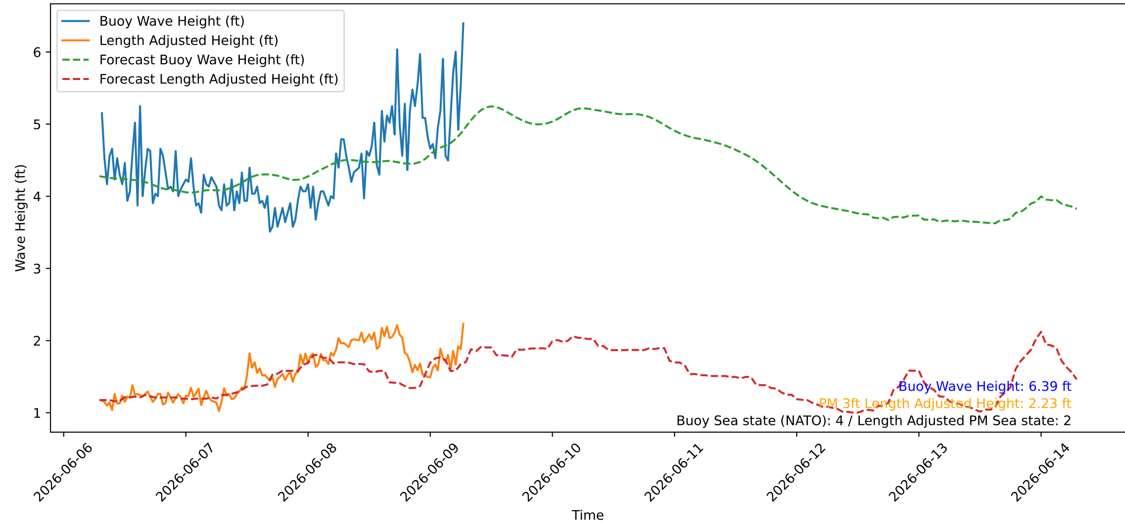
Wave Heights over Time for Oceanside Harbor at 2026-06-09 07:20:26
