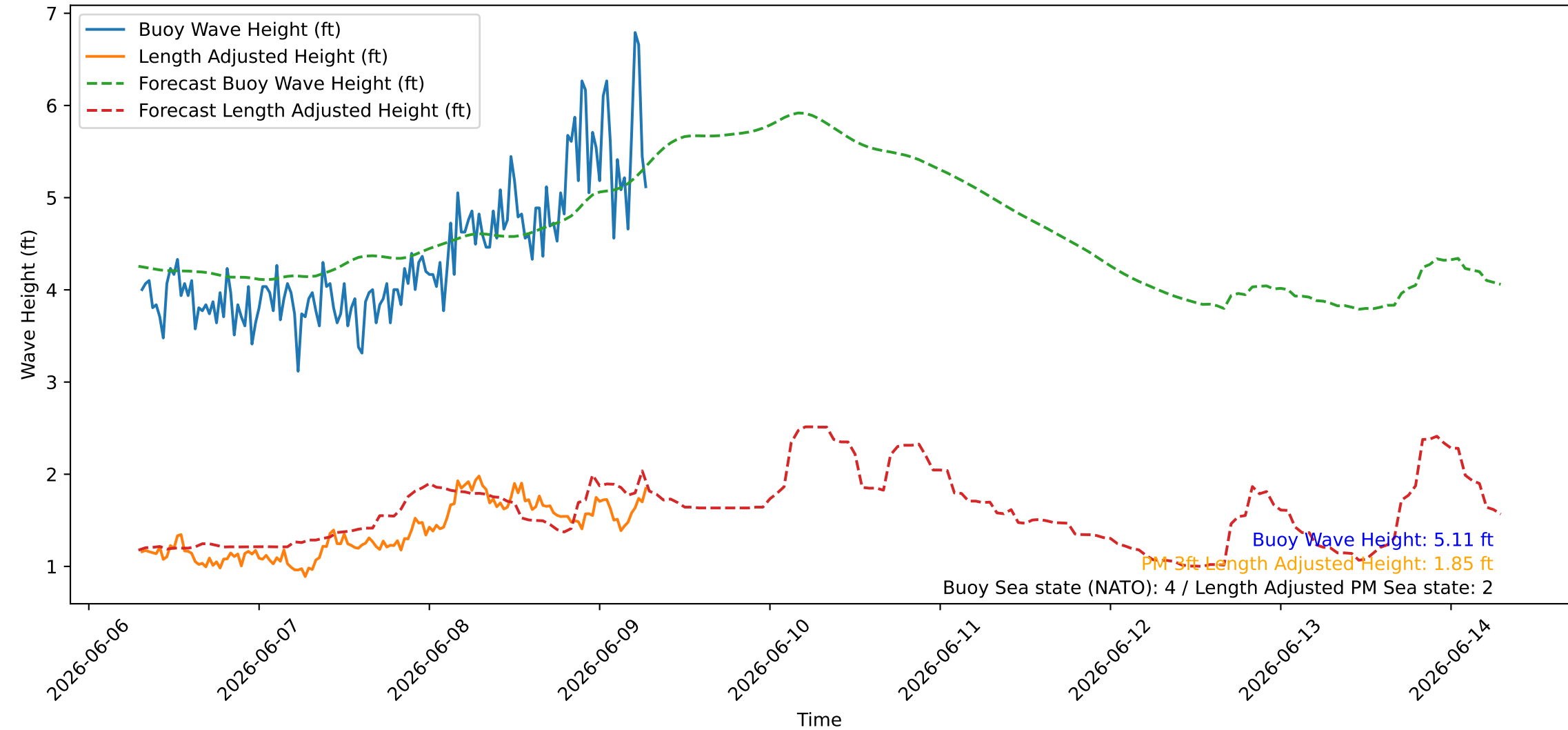
Wave Heights over Time for Green Beach at 2026-06-09 07:21:09
