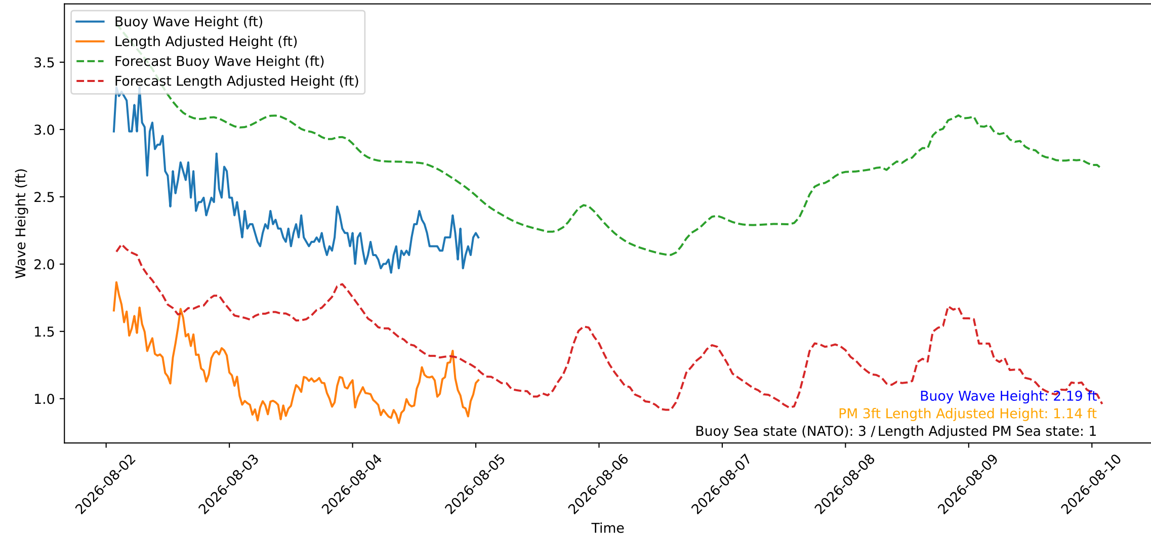
Wave Heights over Time for Green Beach at 2026-08-05 01:31:09
