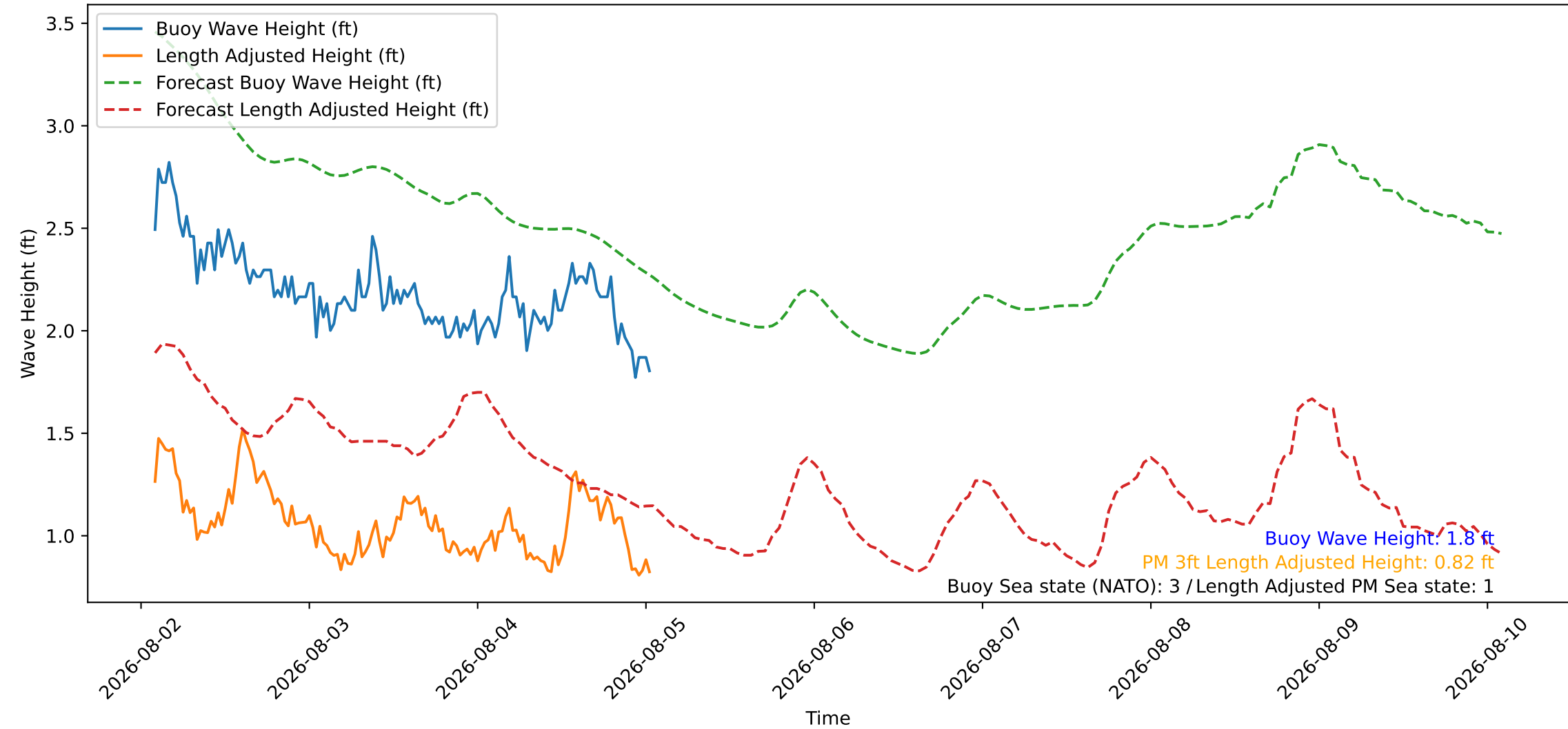
Wave Heights over Time for Red Beach at 2026-08-05 01:30:45
