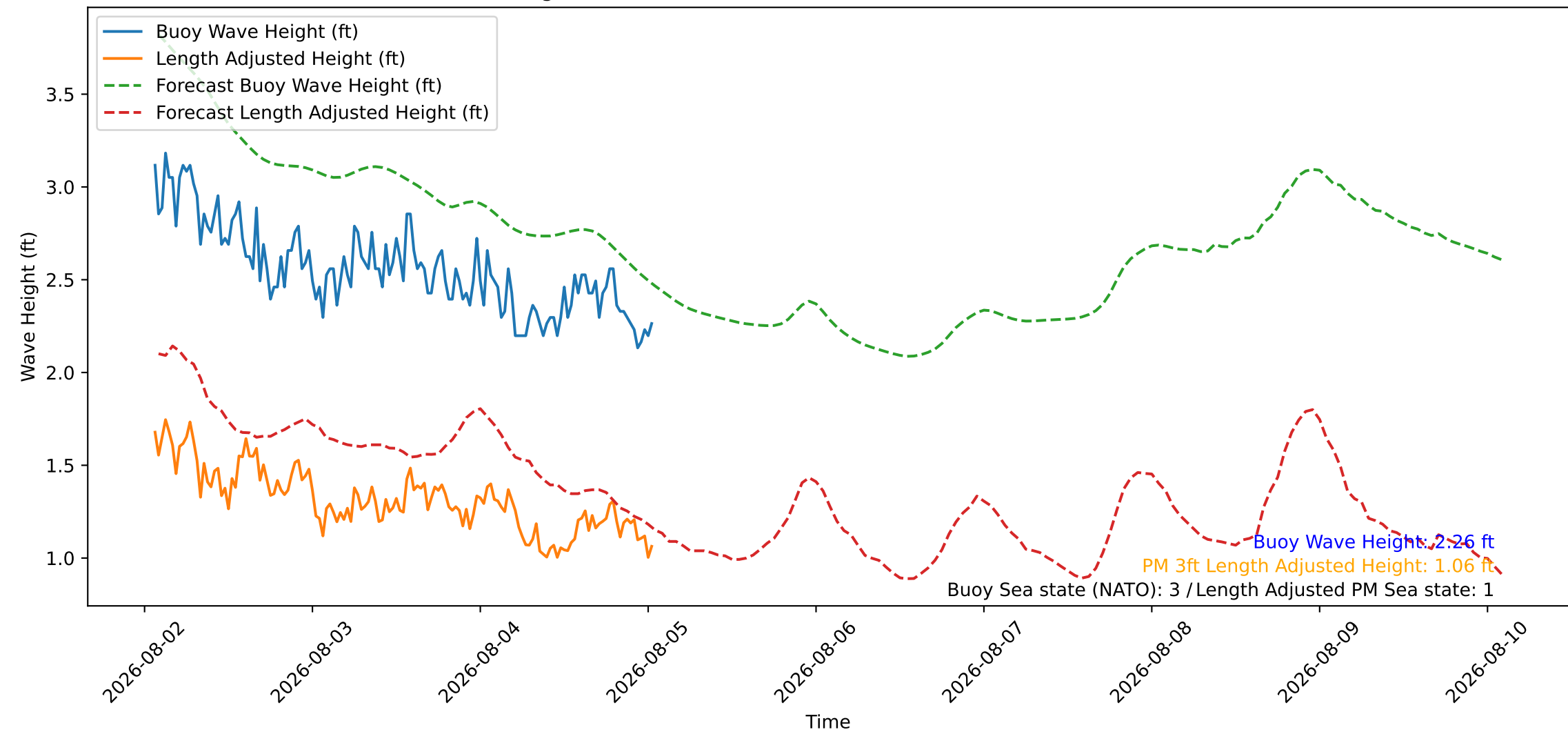
Wave Heights over Time for Oceanside Harbor at 2026-08-05 01:30:26
