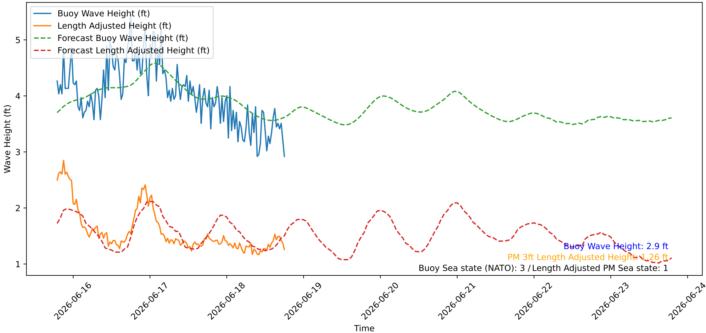
Wave Heights over Time for Oceanside Harbor at 2026-06-18 19:00:27
