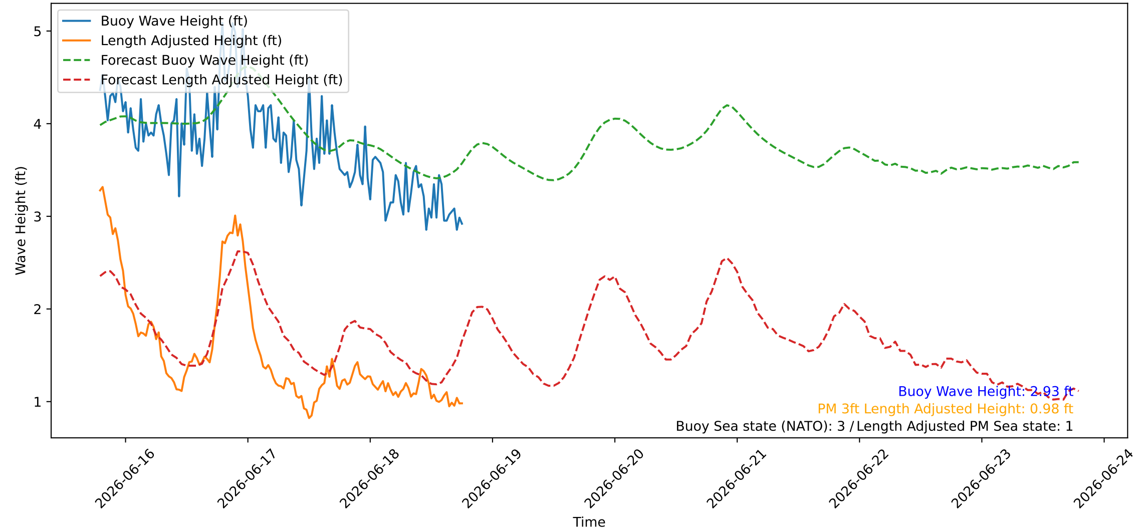
Wave Heights over Time for Green Beach at 2026-06-18 19:01:08
