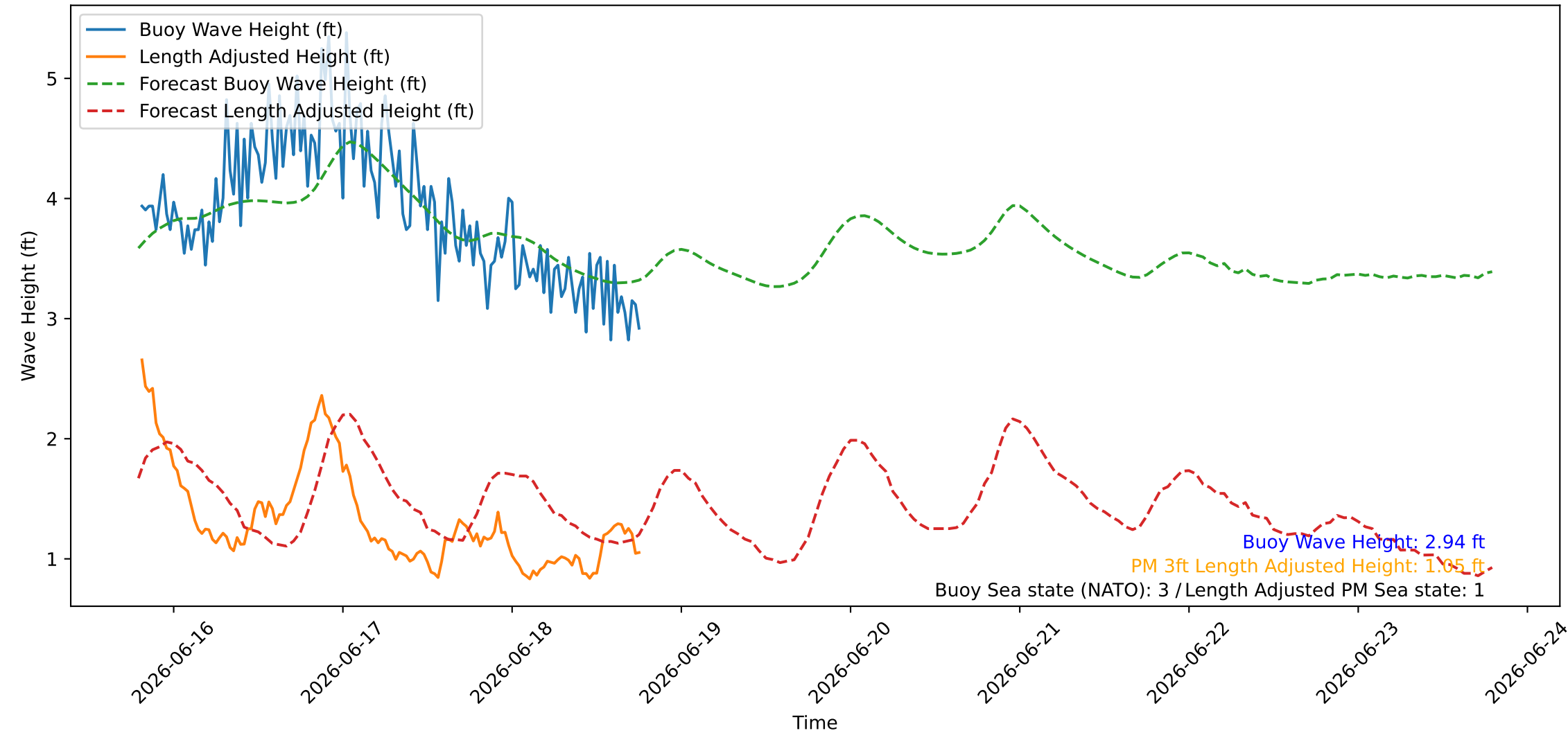
Wave Heights over Time for Red Beach at 2026-06-18 19:00:46
