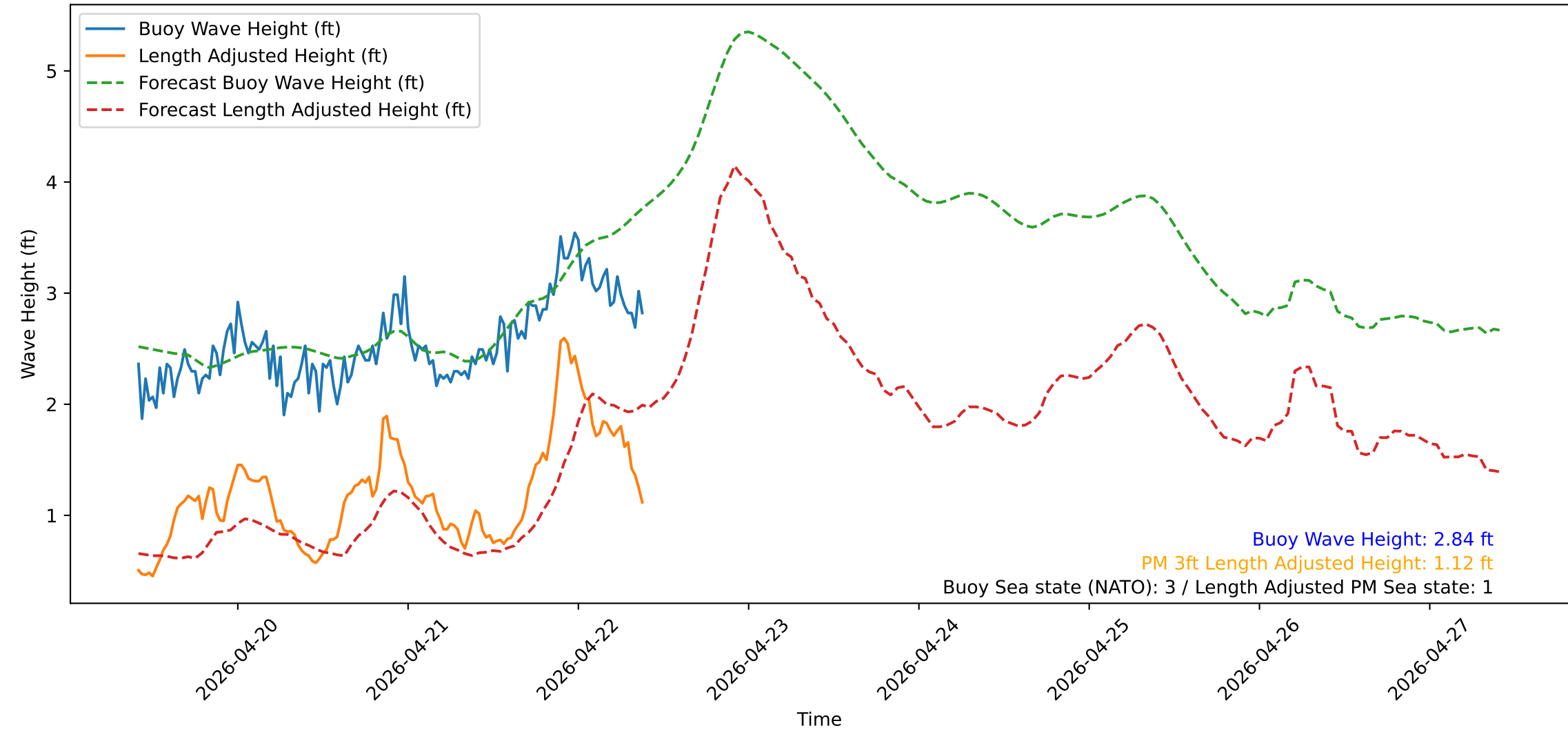
Wave Heights over Time for Green Beach at 2026-04-22 10:01:12
