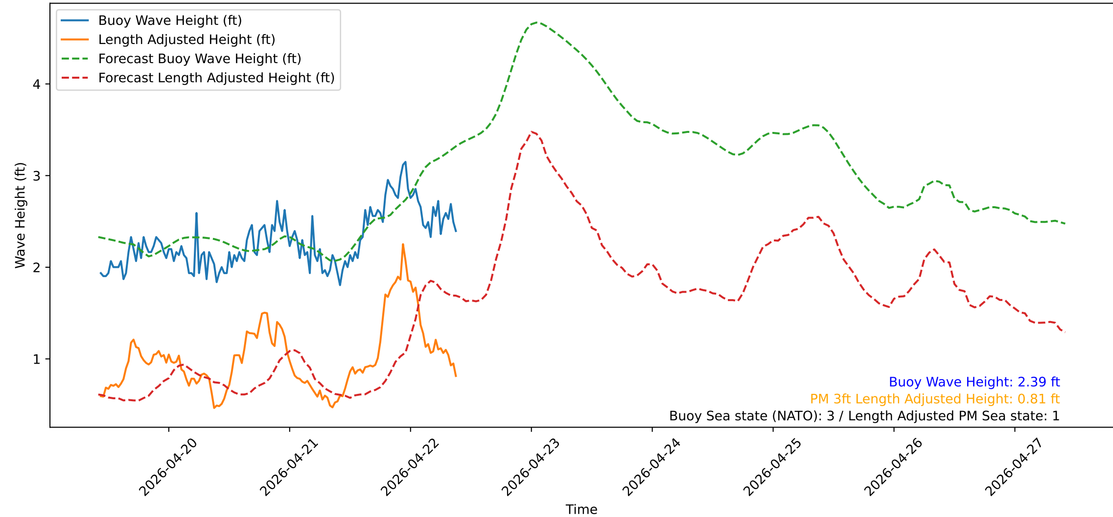
Wave Heights over Time for Red Beach at 2026-04-22 10:00:50
