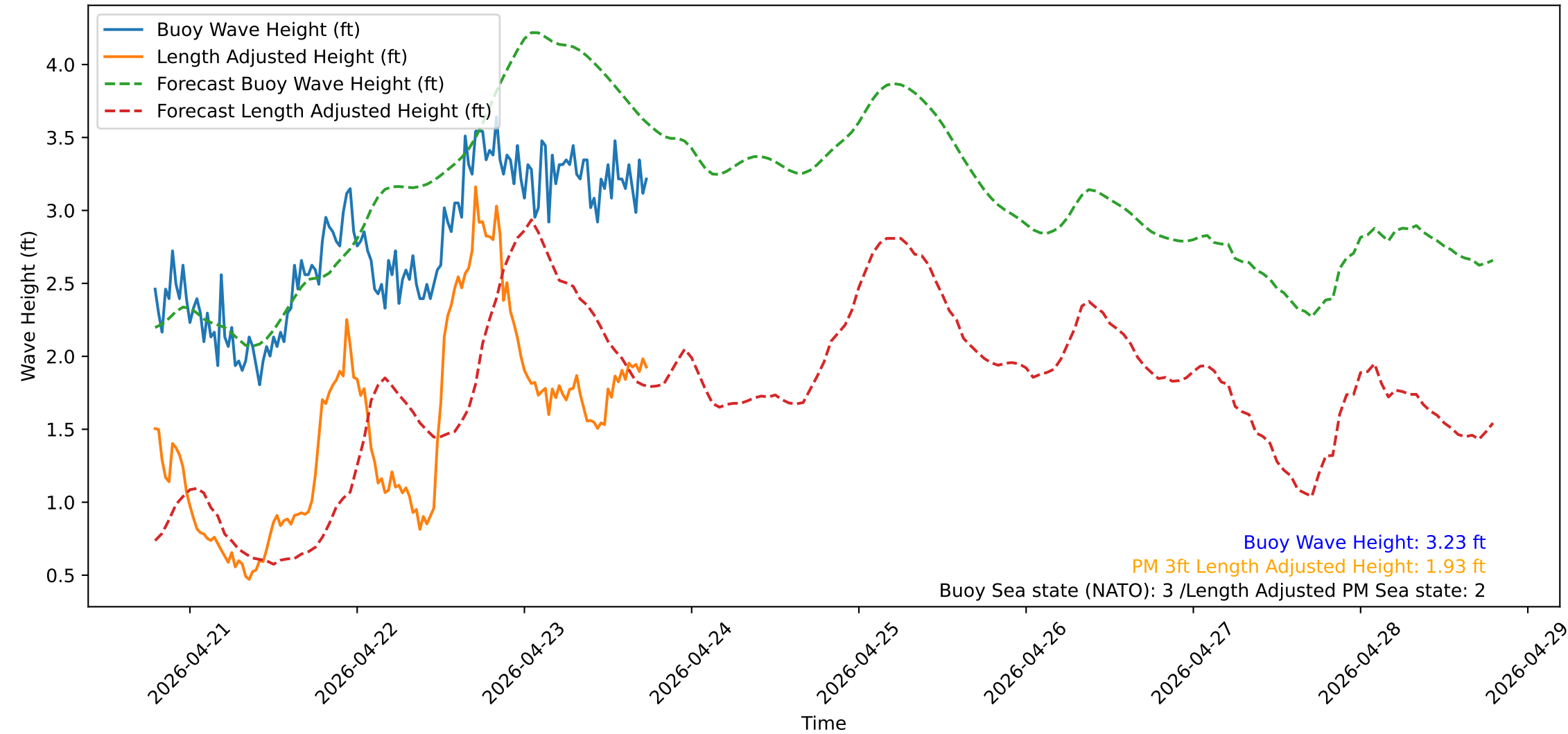
Wave Heights over Time for Red Beach at 2026-04-23 18:30:51
