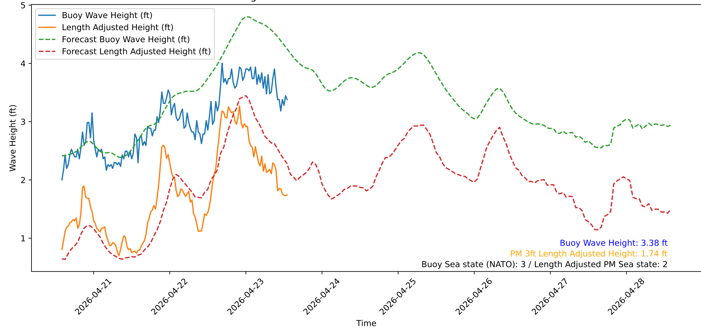
Wave Heights over Time for Green Beach at 2026-04-23 13:51:13
