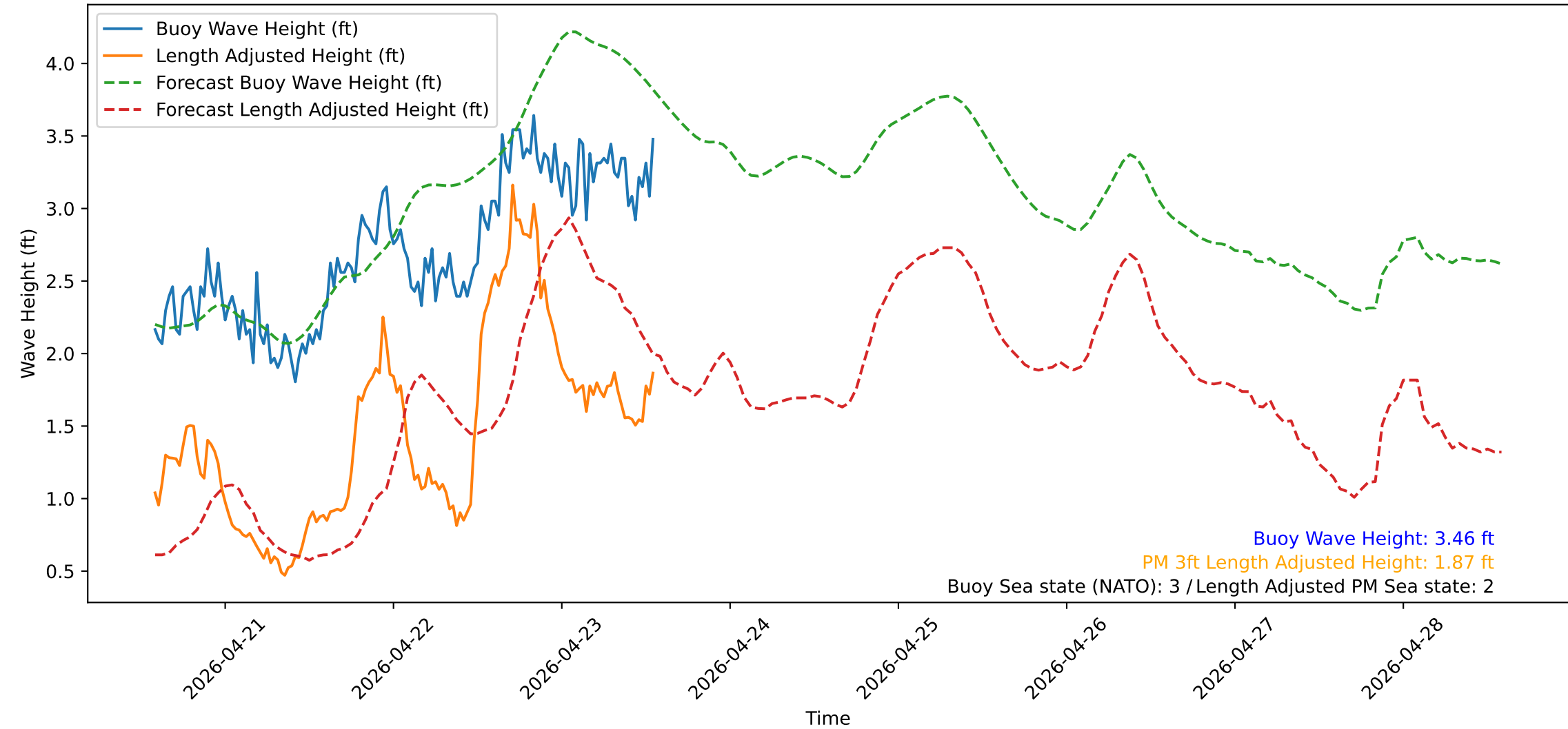
Wave Heights over Time for Red Beach at 2026-04-23 13:50:51
