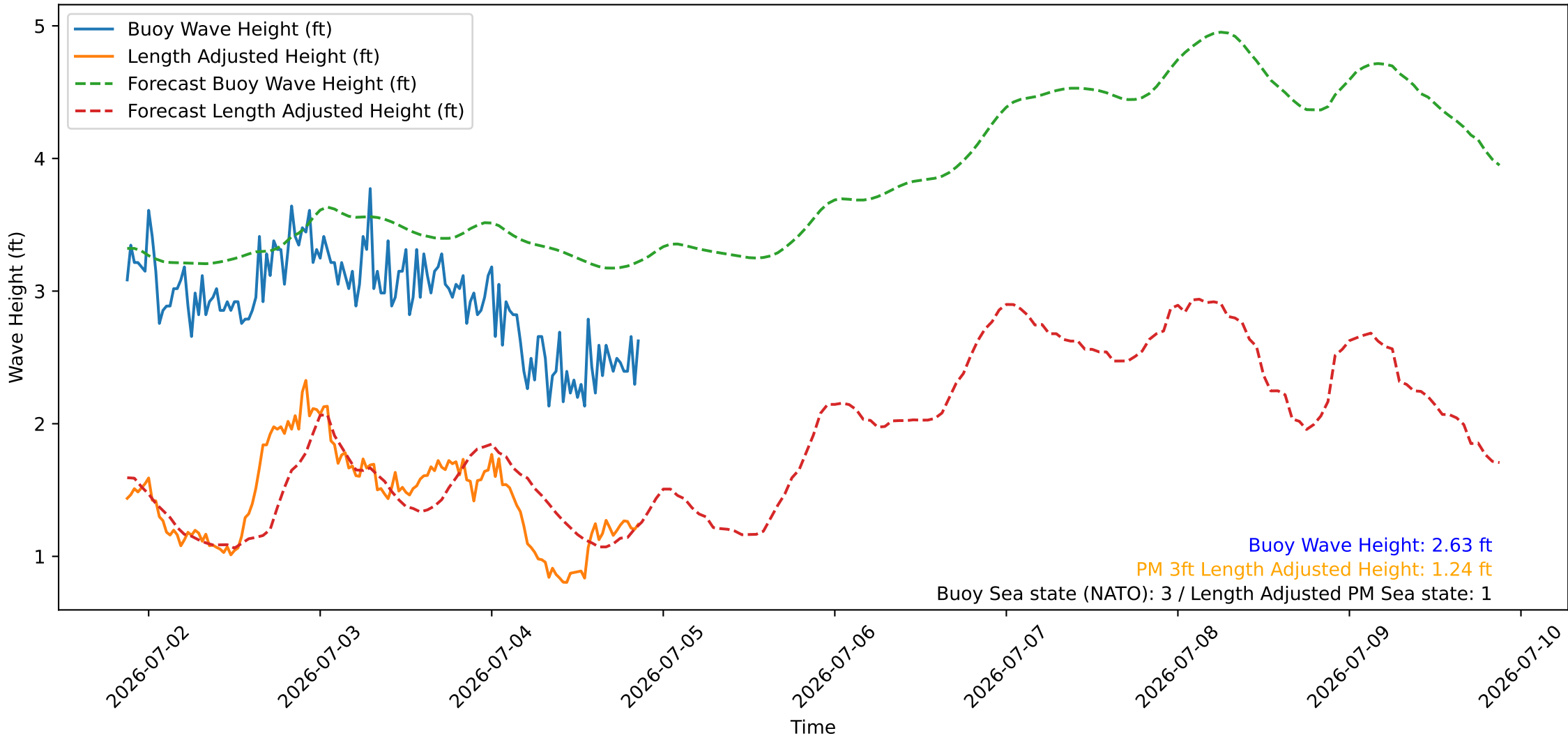
Wave Heights over Time for Oceanside Harbor at 2026-07-04 21:10:27
