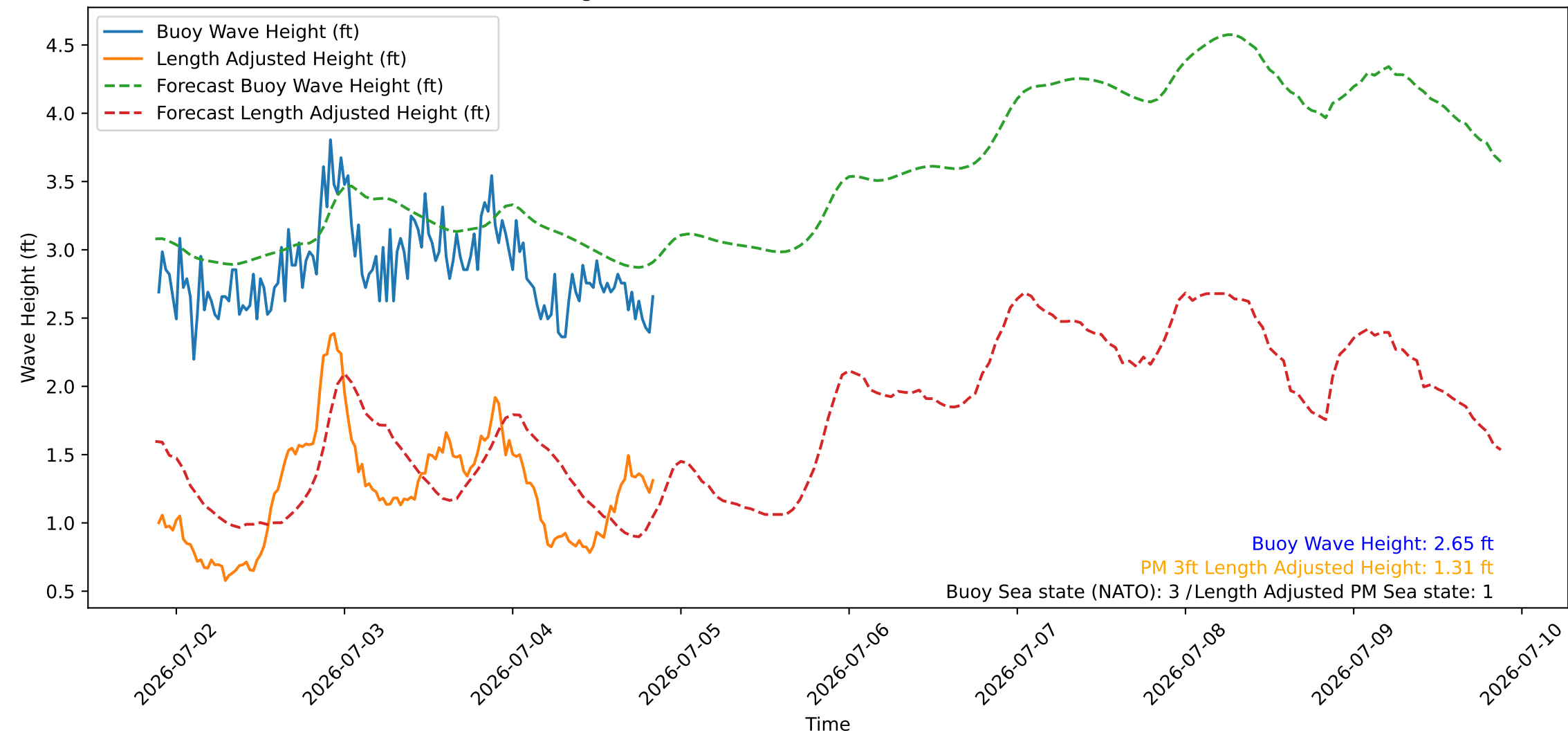
Wave Heights over Time for Red Beach at 2026-07-04 21:10:46
