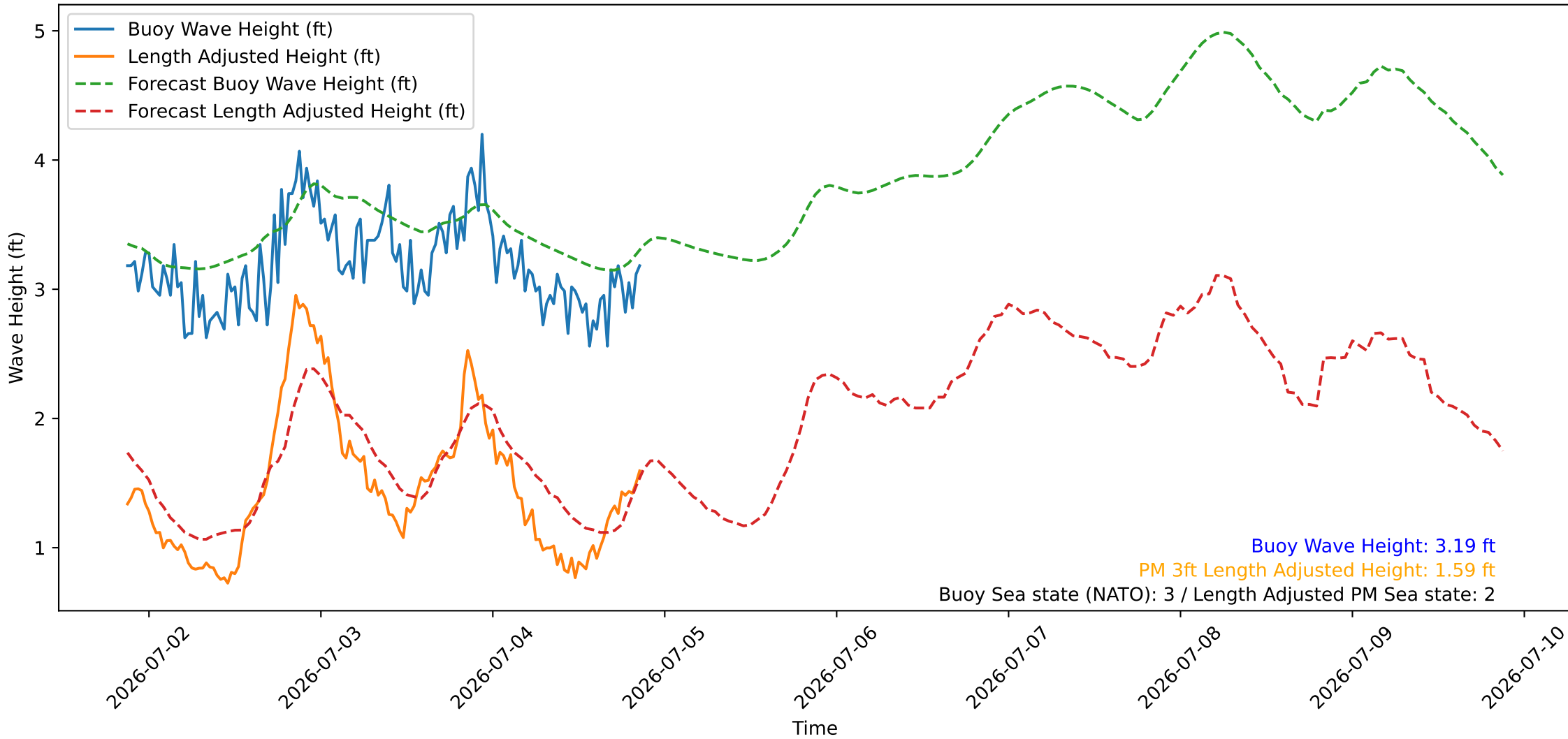
Wave Heights over Time for Green Beach at 2026-07-04 21:11:08
