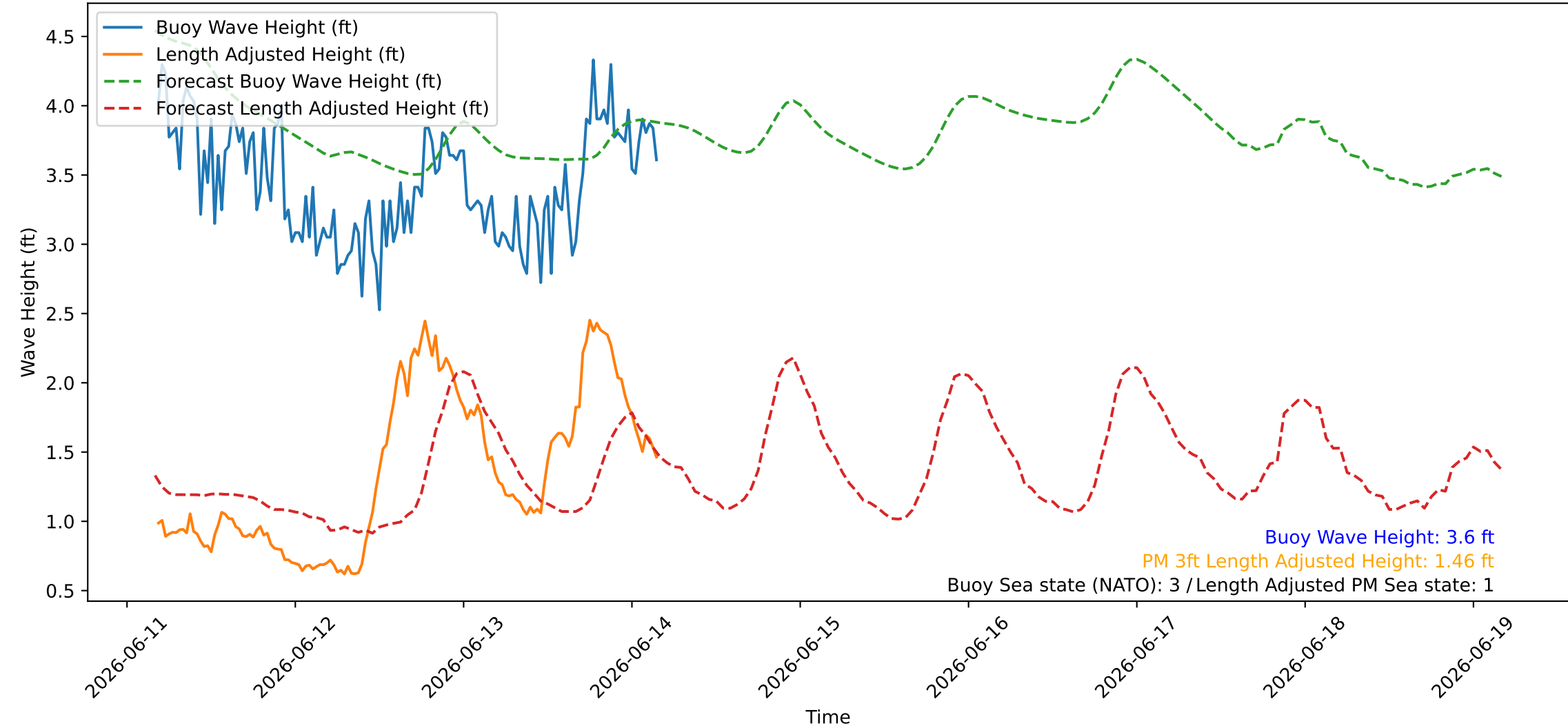
Wave Heights over Time for Red Beach at 2026-06-14 04:10:46
