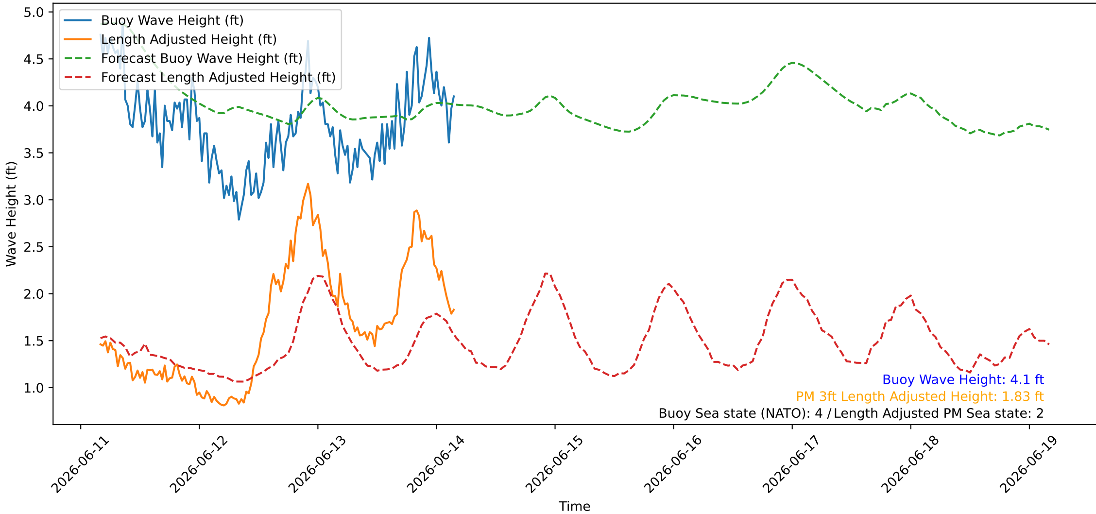
Wave Heights over Time for Oceanside Harbor at 2026-06-14 04:10:26
