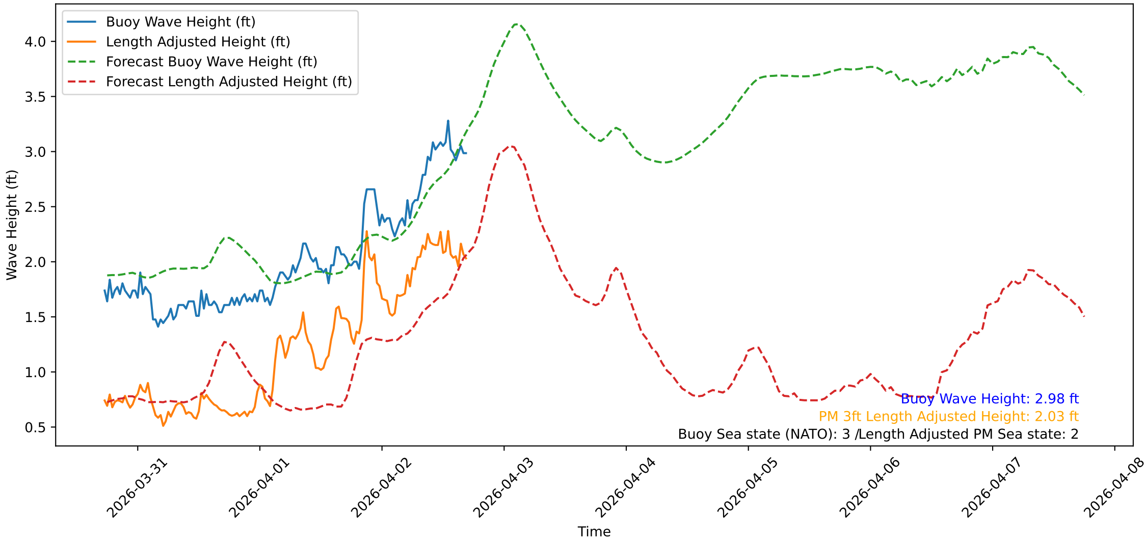
Wave Heights over Time for Green Beach at 2026-04-02 17:31:10
