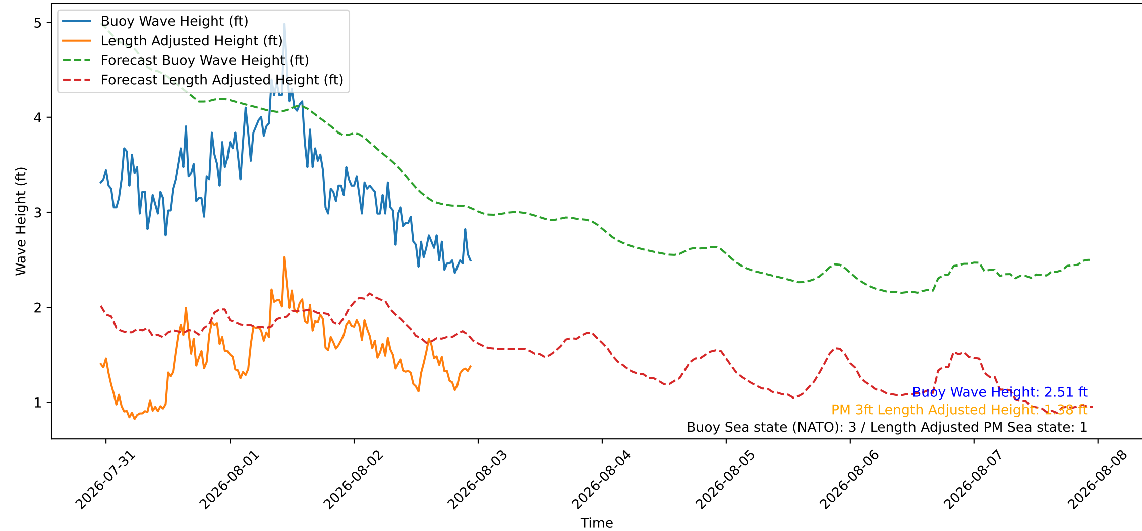
Wave Heights over Time for Green Beach at 2026-08-02 23:11:08
