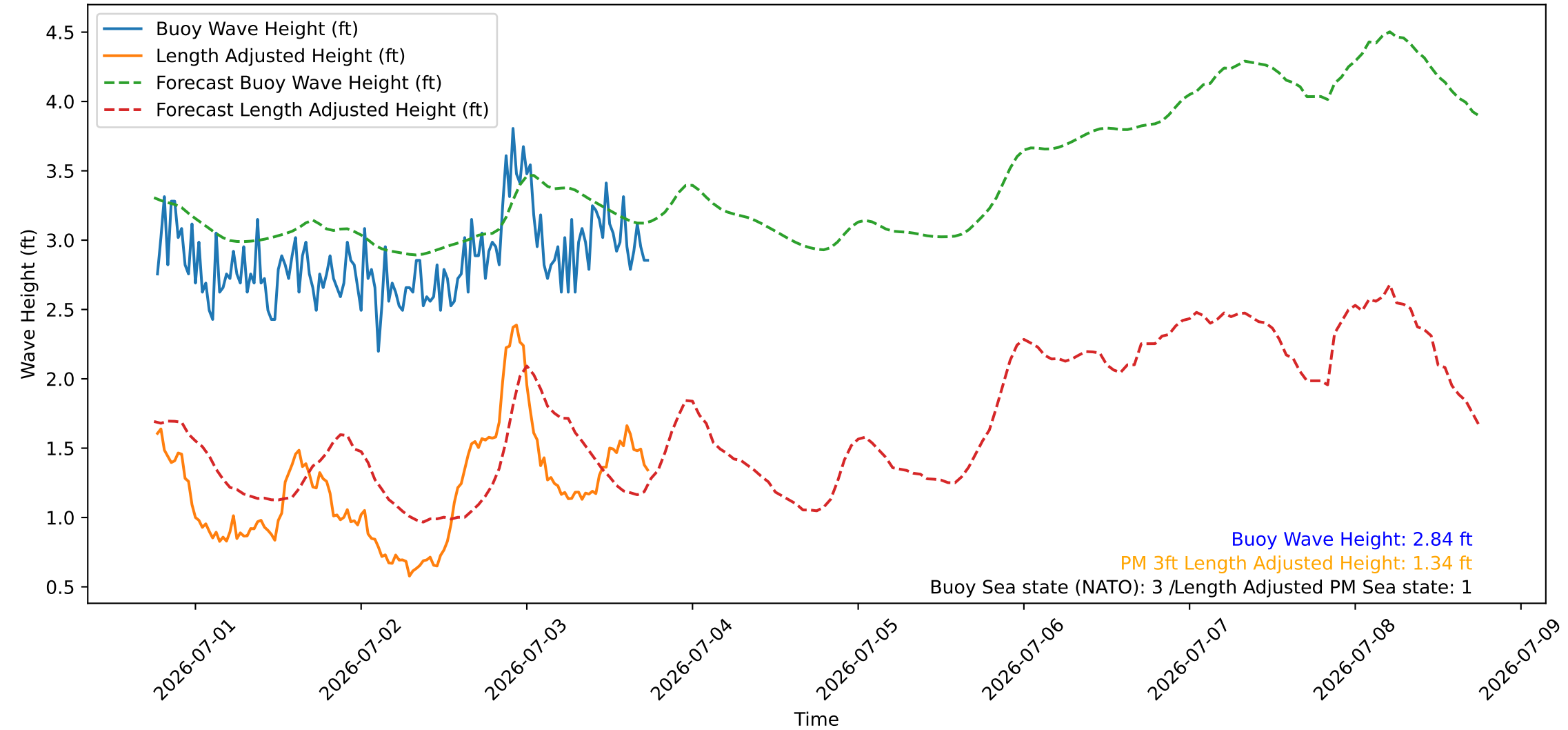
Wave Heights over Time for Red Beach at 2026-07-03 18:20:48
