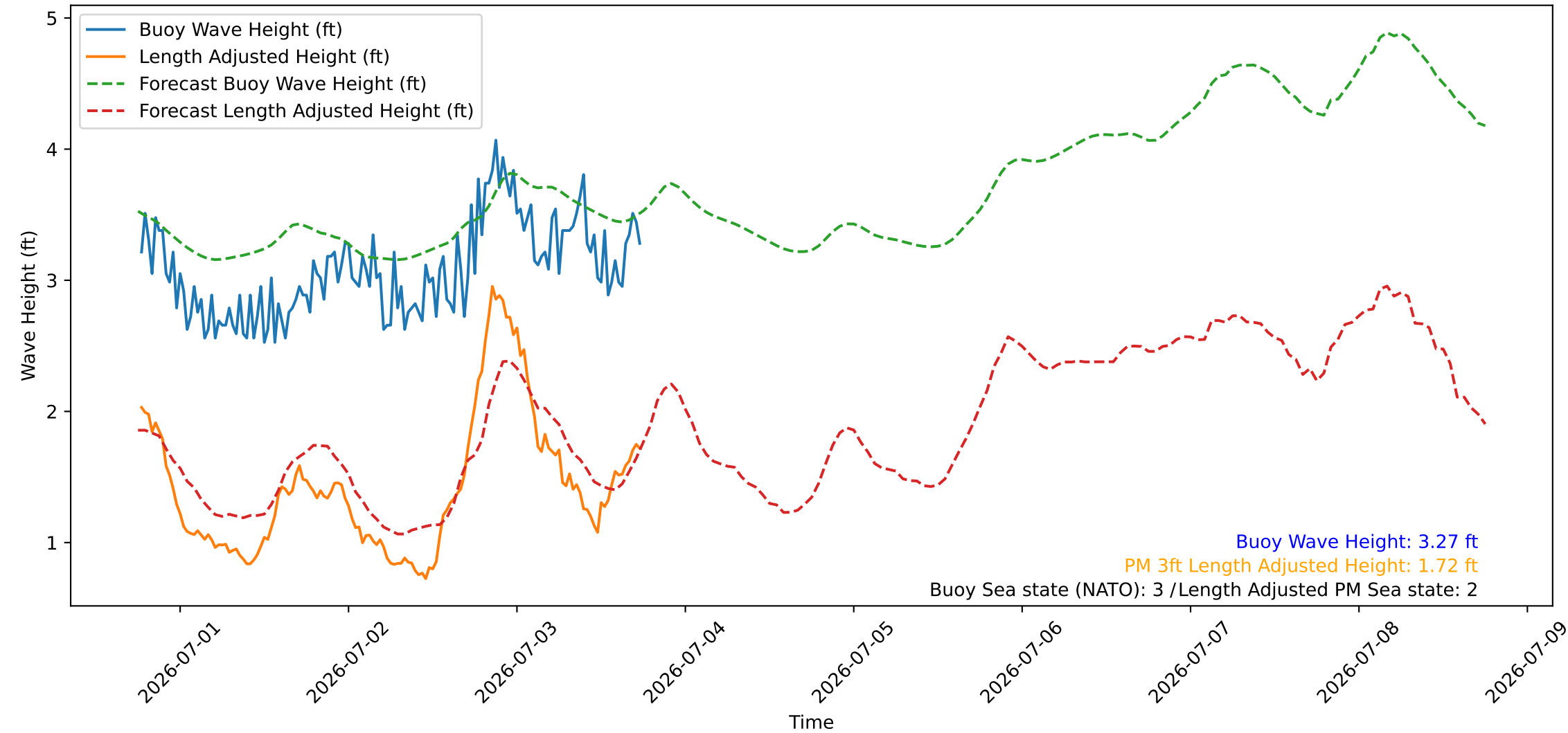
Wave Heights over Time for Green Beach at 2026-07-03 18:21:09
