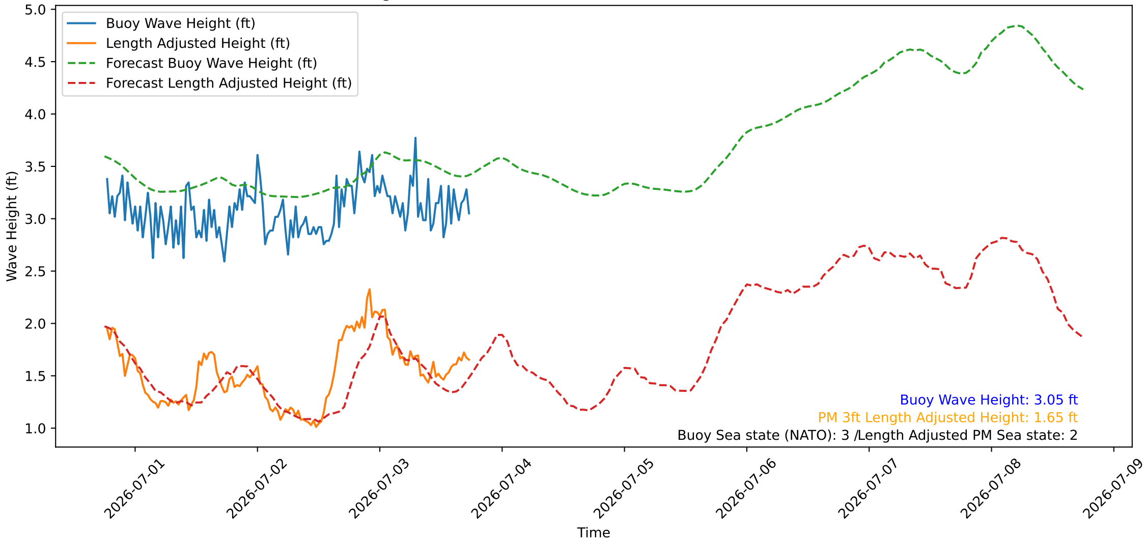
Wave Heights over Time for Oceanside Harbor at 2026-07-03 18:20:26
