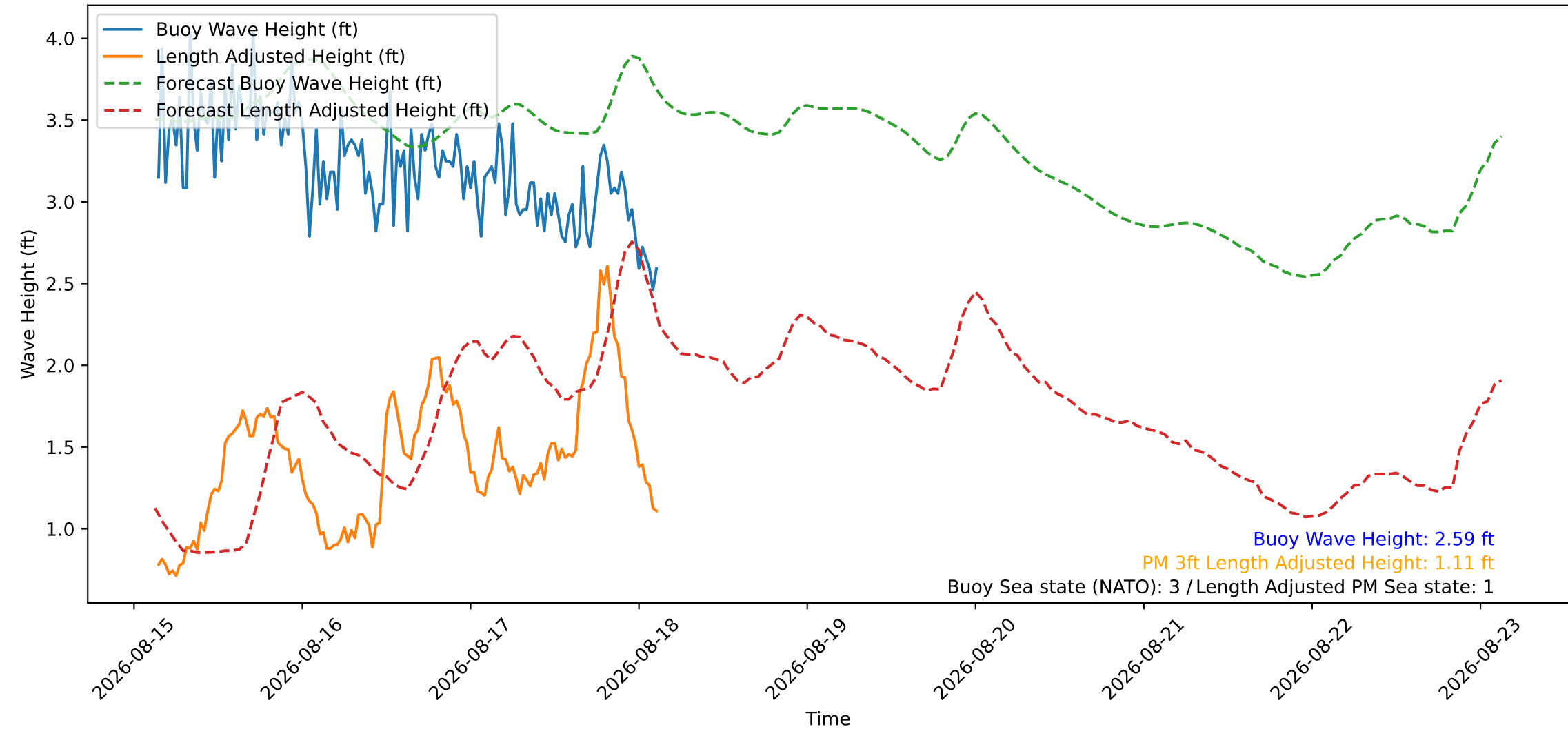
Wave Heights over Time for Red Beach at 2026-08-18 03:20:47
