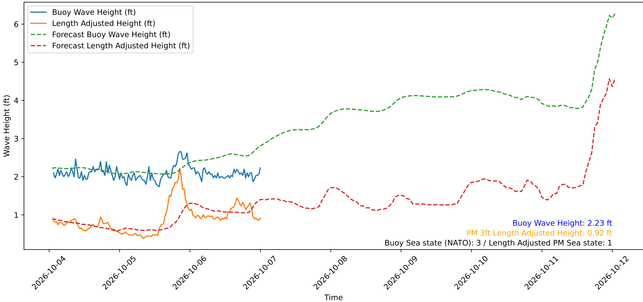
Wave Heights over Time for Red Beach at 2026-10-07 01:00:49
