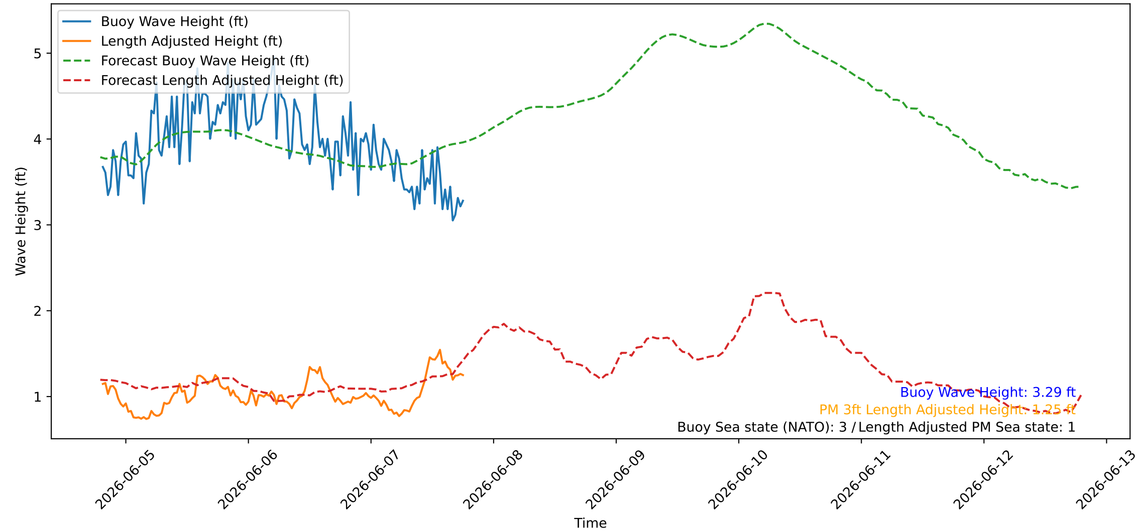
Wave Heights over Time for Red Beach at 2026-06-07 19:00:46
