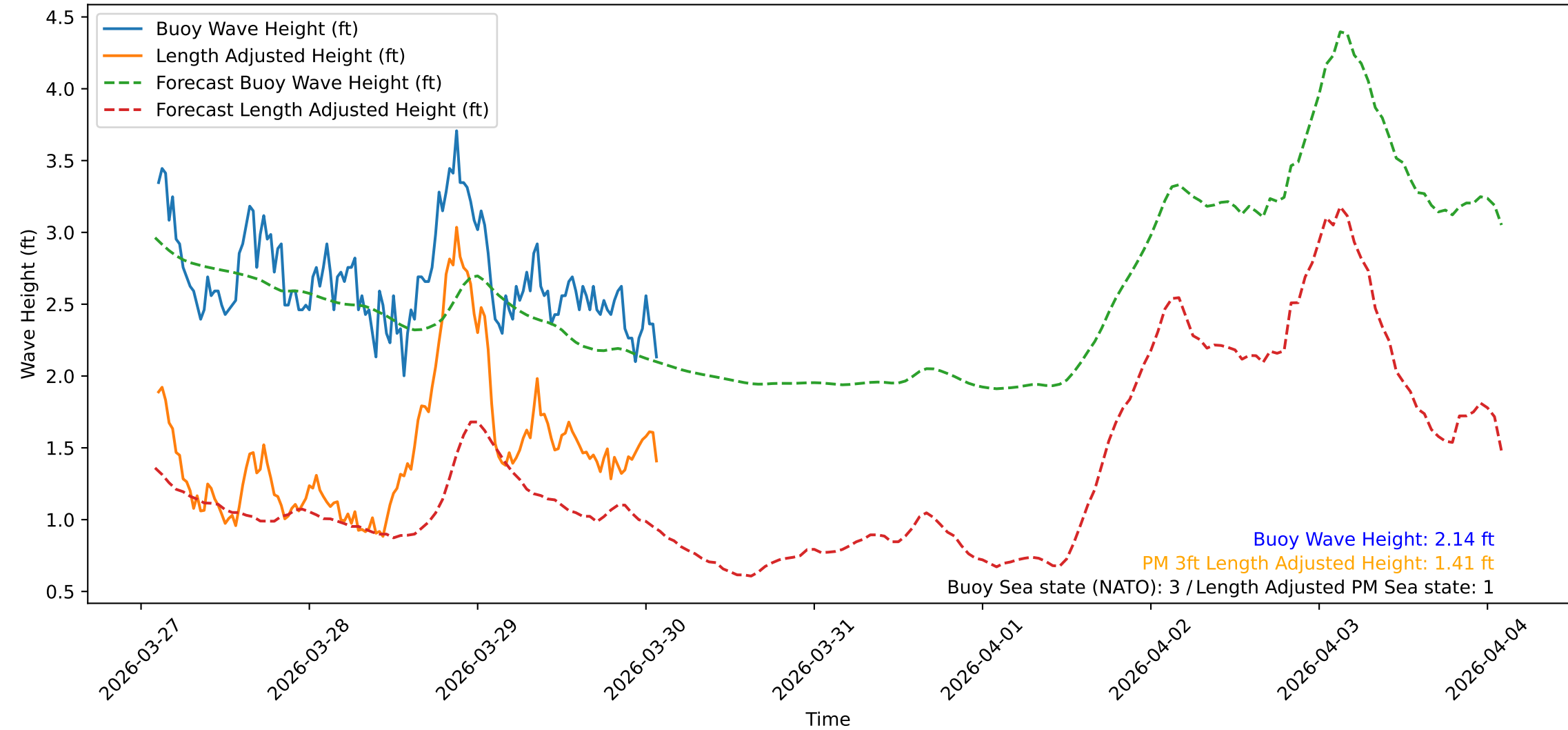
Wave Heights over Time for Green Beach at 2026-03-30 02:21:11
