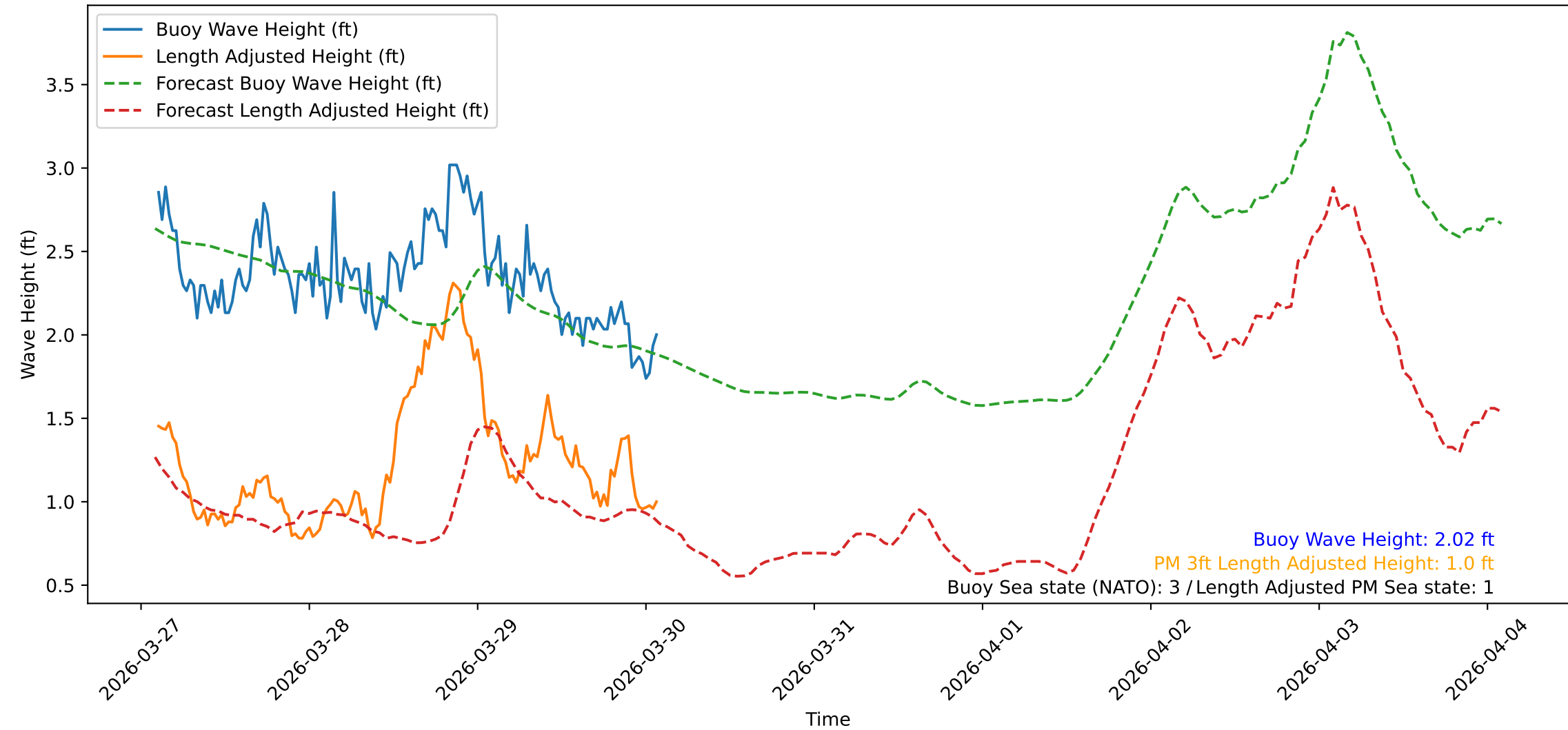
Wave Heights over Time for Red Beach at 2026-03-30 02:20:48
