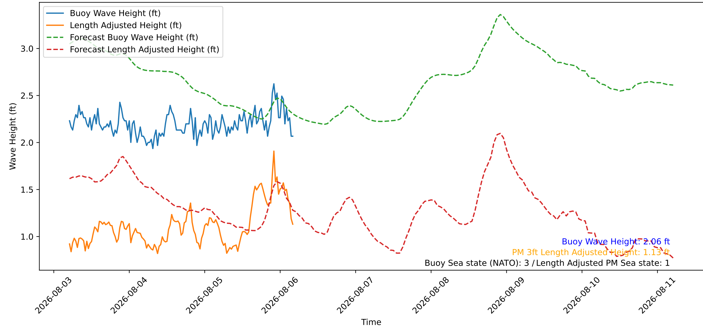
Wave Heights over Time for Green Beach at 2026-08-06 04:51:09
