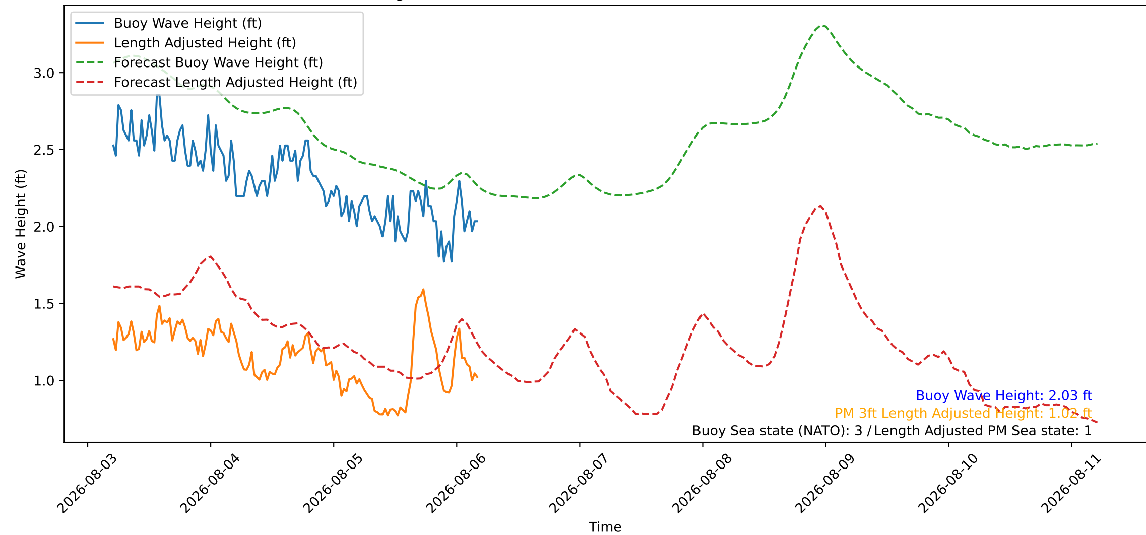
Wave Heights over Time for Oceanside Harbor at 2026-08-06 04:50:26
