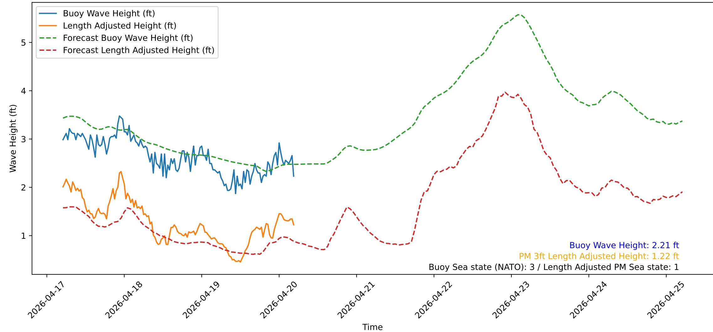
Wave Heights over Time for Green Beach at 2026-04-20 05:11:12
