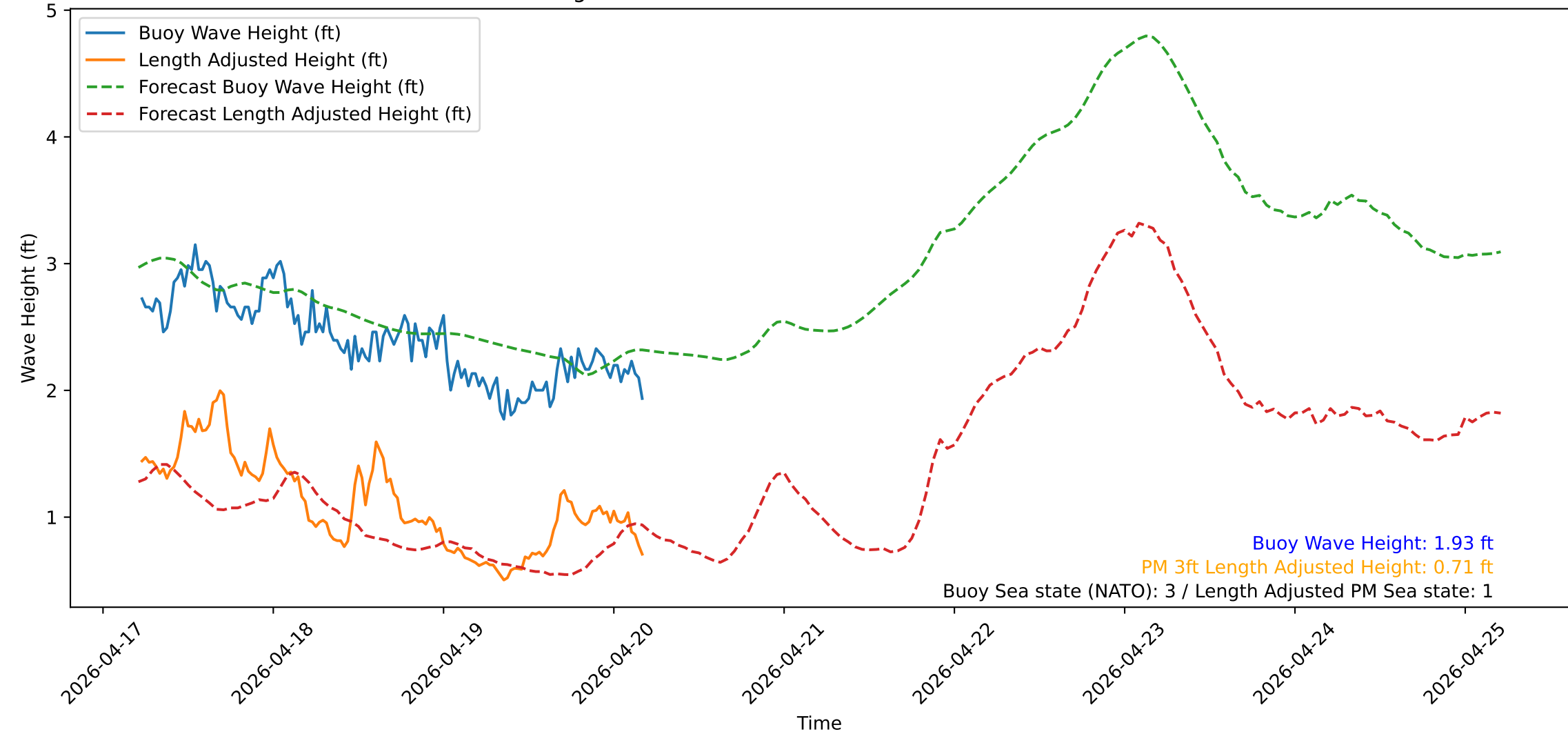
Wave Heights over Time for Red Beach at 2026-04-20 05:10:50
