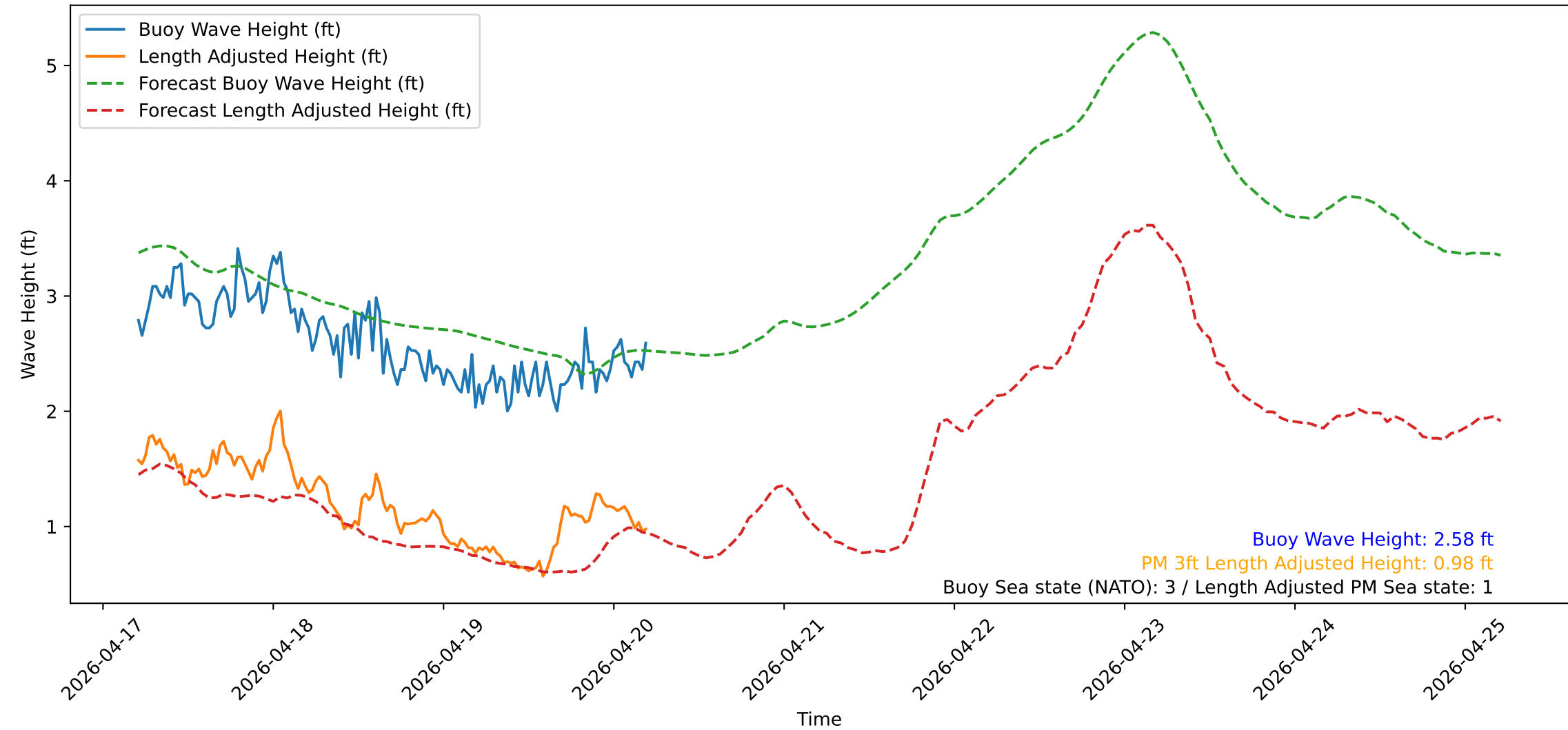
Wave Heights over Time for Oceanside Harbor at 2026-04-20 05:10:31
