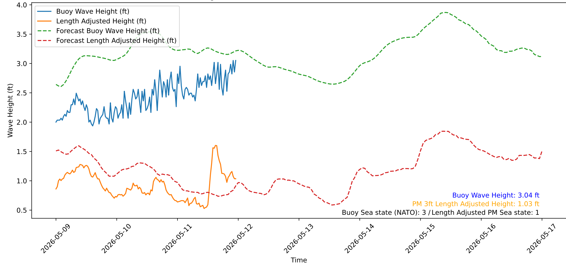
Wave Heights over Time for Red Beach at 2026-05-11 23:40:50
