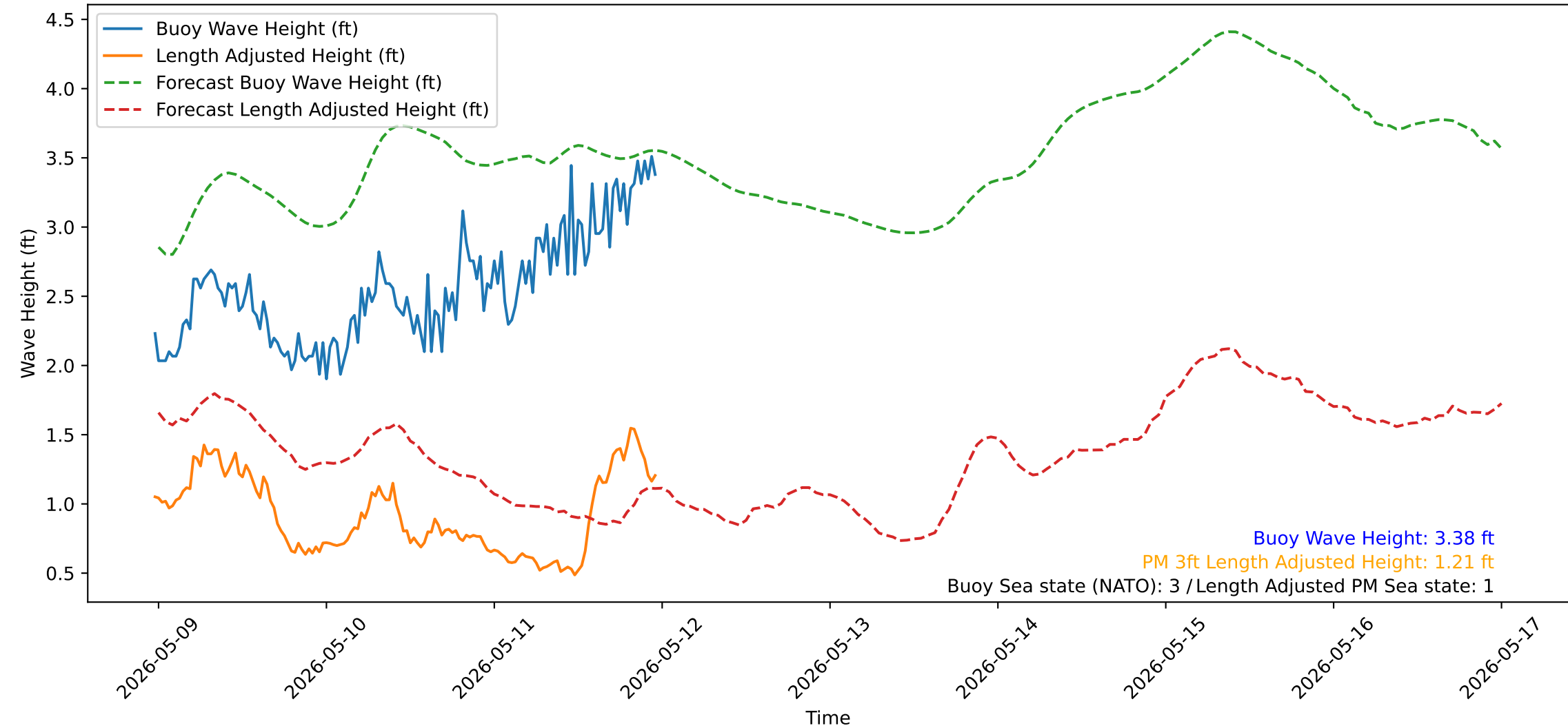
Wave Heights over Time for Green Beach at 2026-05-11 23:41:12
