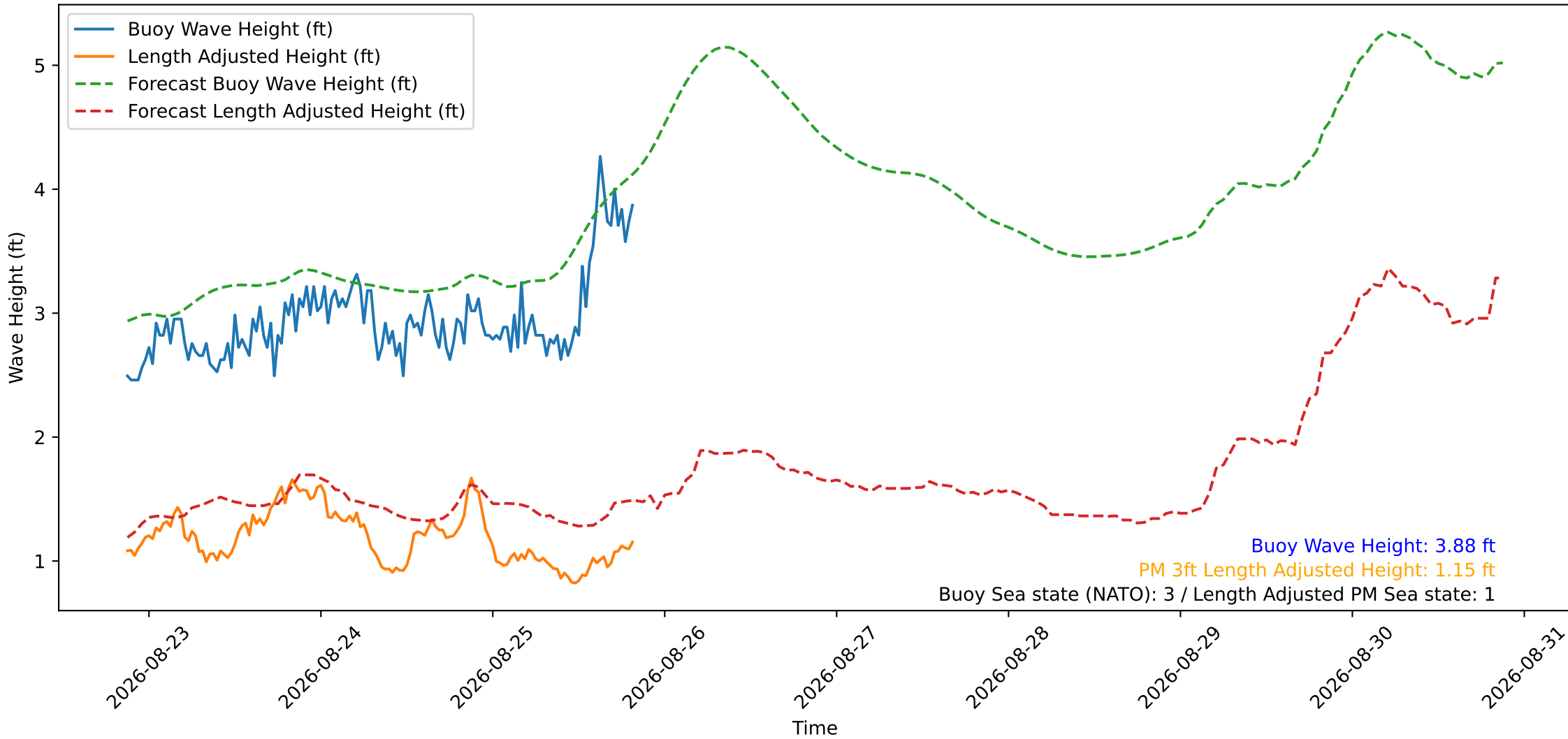
Wave Heights over Time for Green Beach at 2026-08-25 20:31:13
