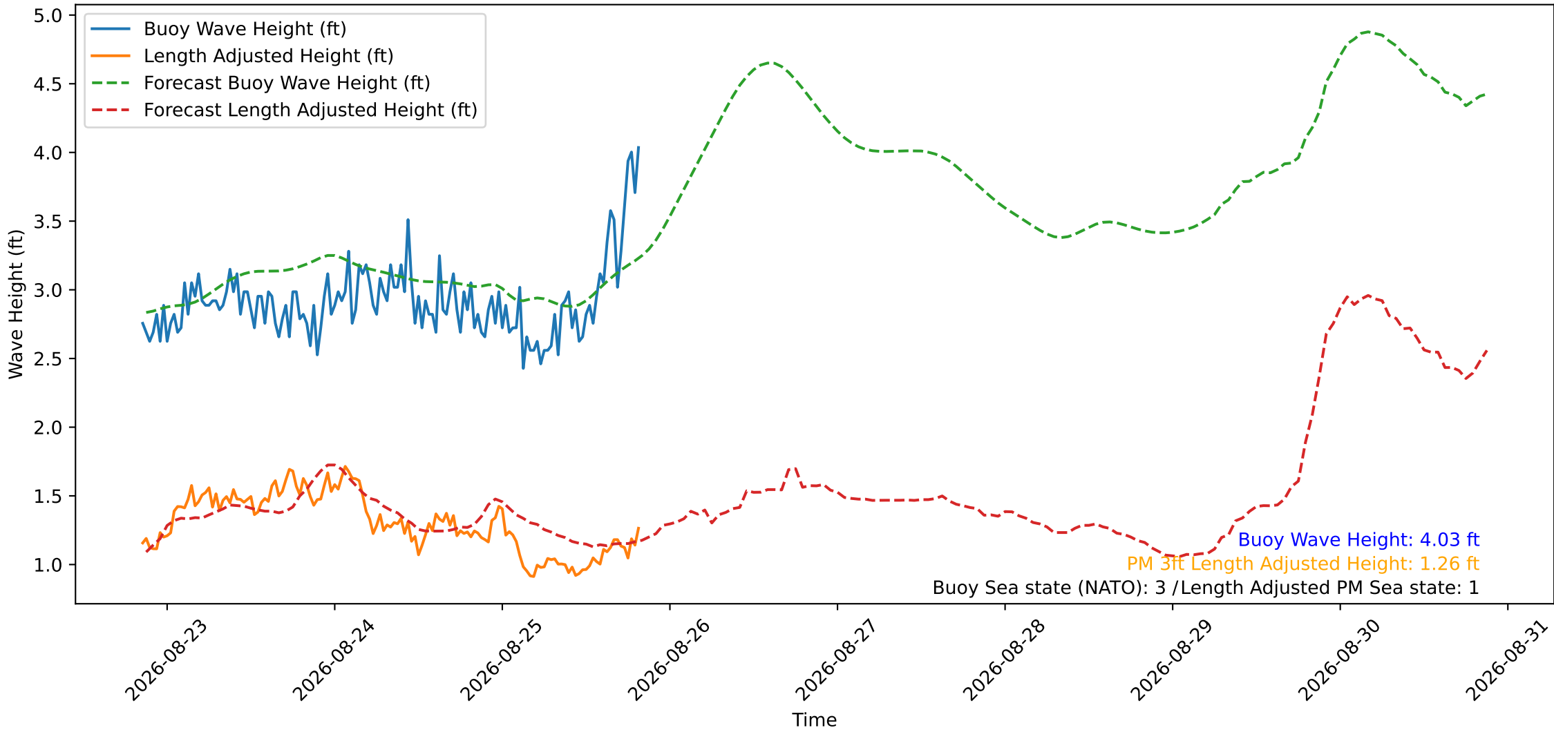
Wave Heights over Time for Oceanside Harbor at 2026-08-25 20:30:30
