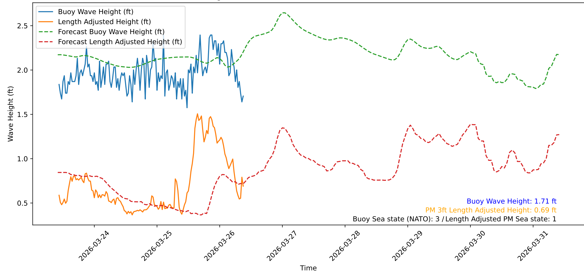
Wave Heights over Time for Red Beach at 2026-03-26 10:00:48
