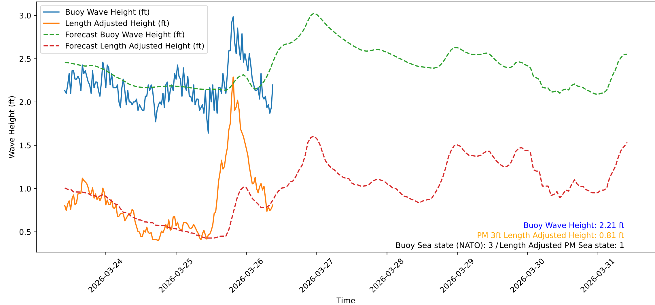
Wave Heights over Time for Green Beach at 2026-03-26 10:01:11
