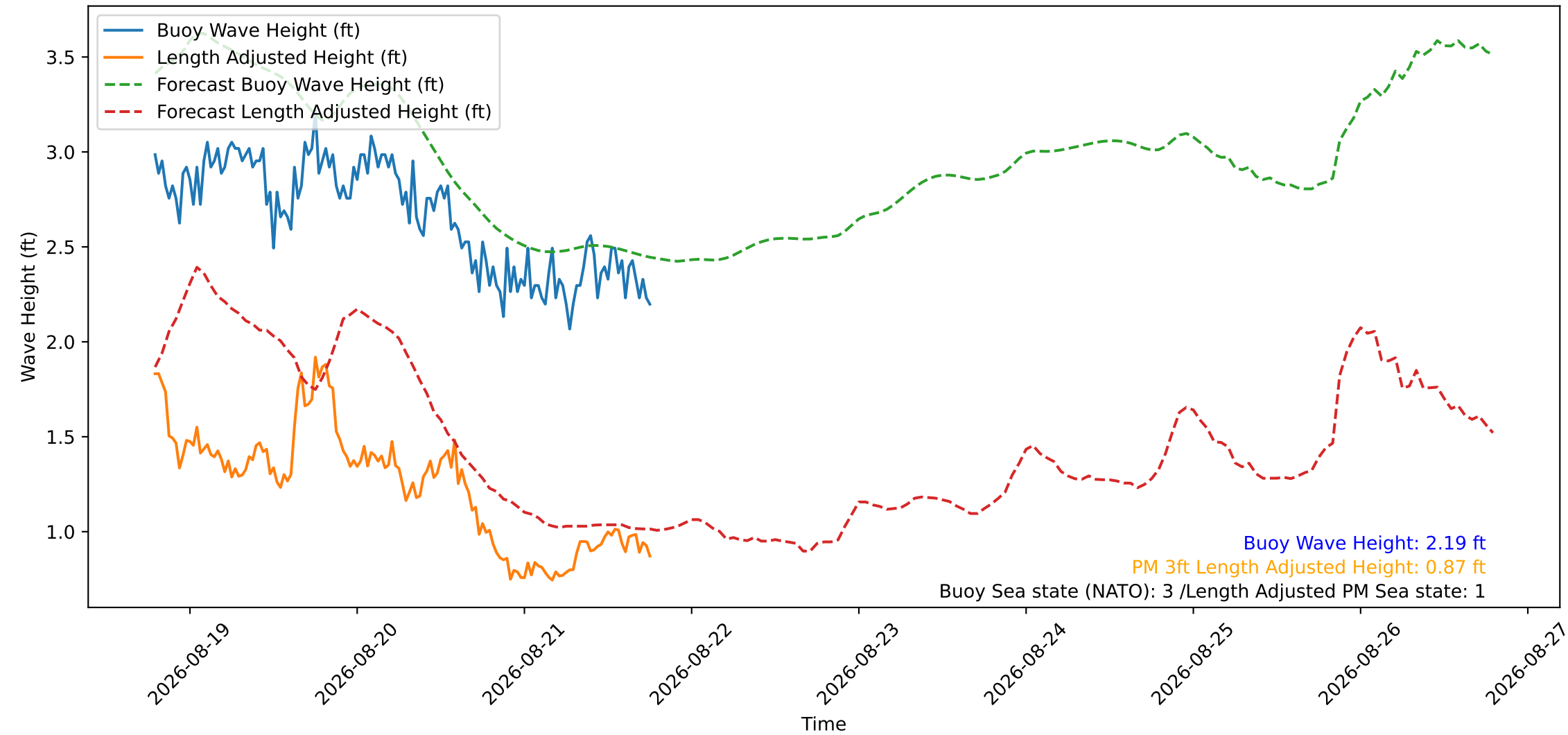
Wave Heights over Time for Red Beach at 2026-08-21 18:50:47
