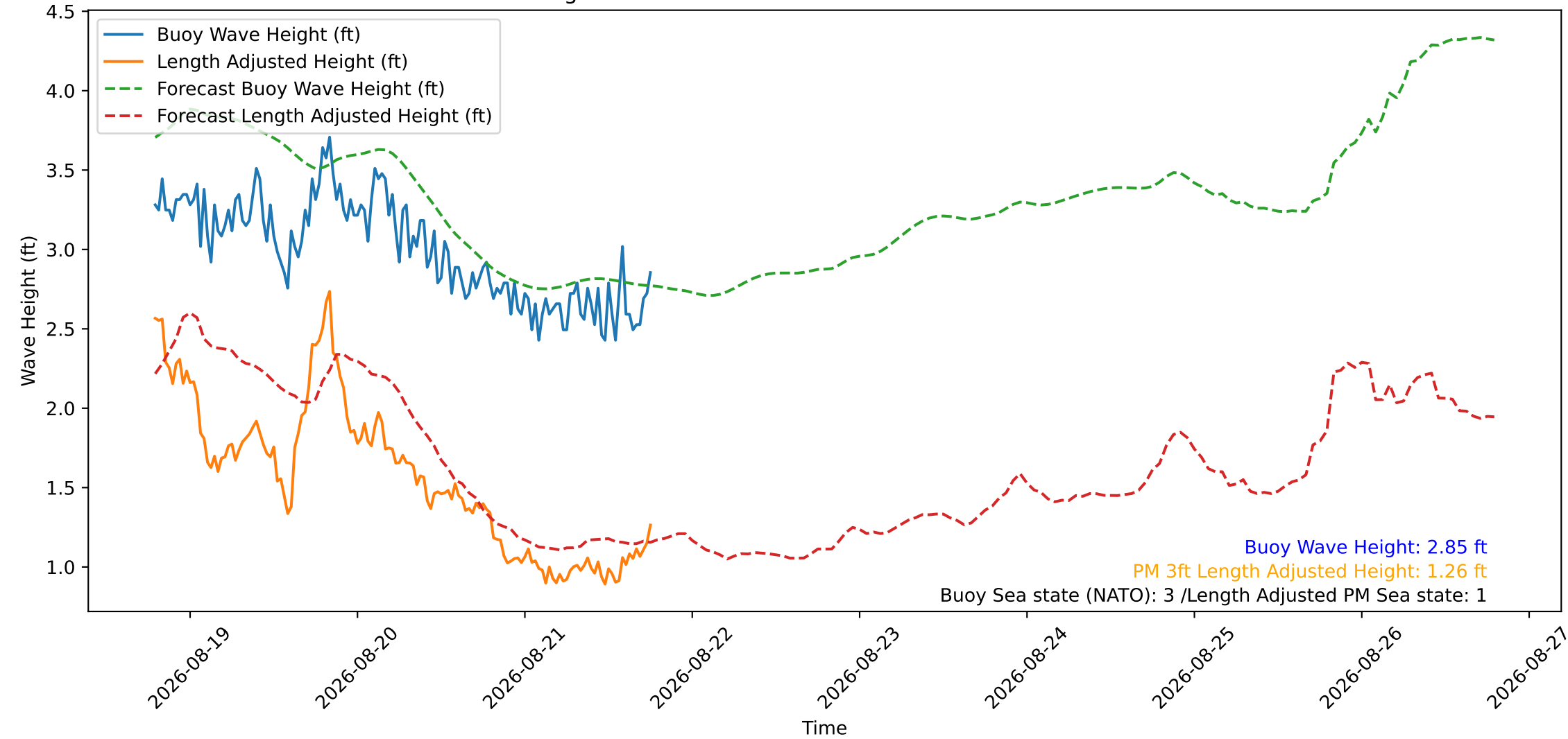
Wave Heights over Time for Green Beach at 2026-08-21 18:51:10
