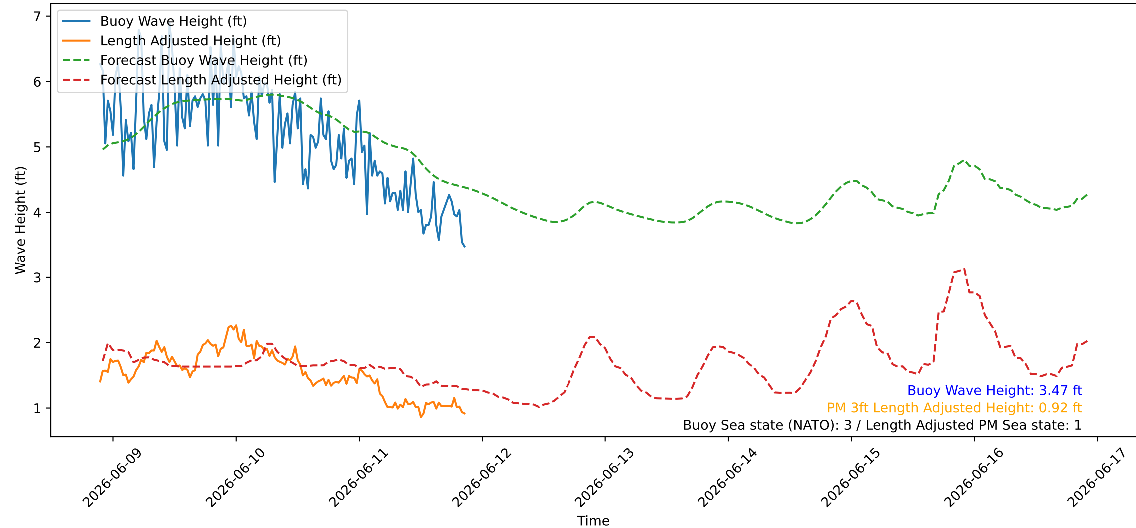
Wave Heights over Time for Green Beach at 2026-06-11 21:31:08
