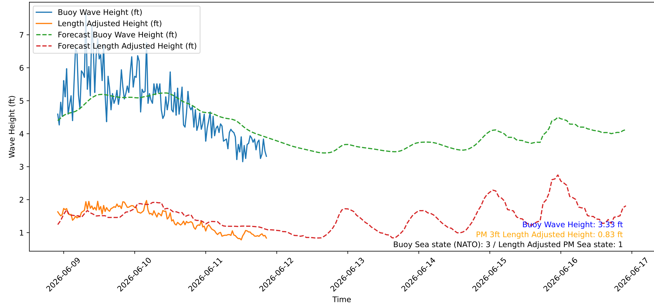
Wave Heights over Time for Red Beach at 2026-06-11 21:30:46
