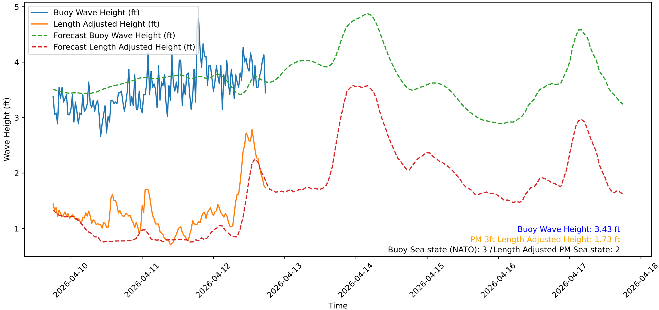
Wave Heights over Time for Oceanside Harbor at 2026-04-12 18:10:31
