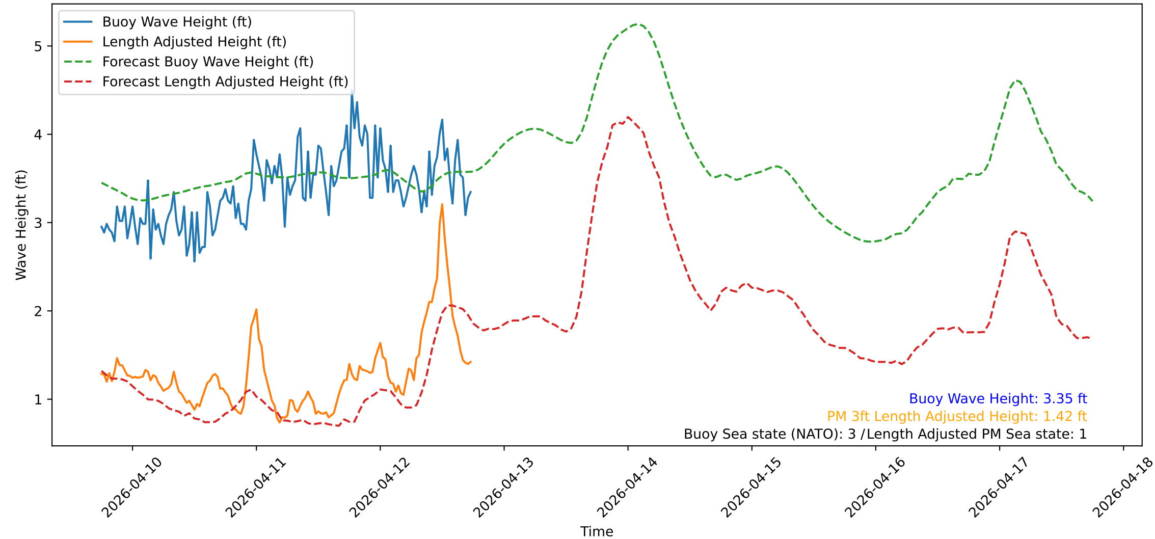
Wave Heights over Time for Green Beach at 2026-04-12 18:11:11
