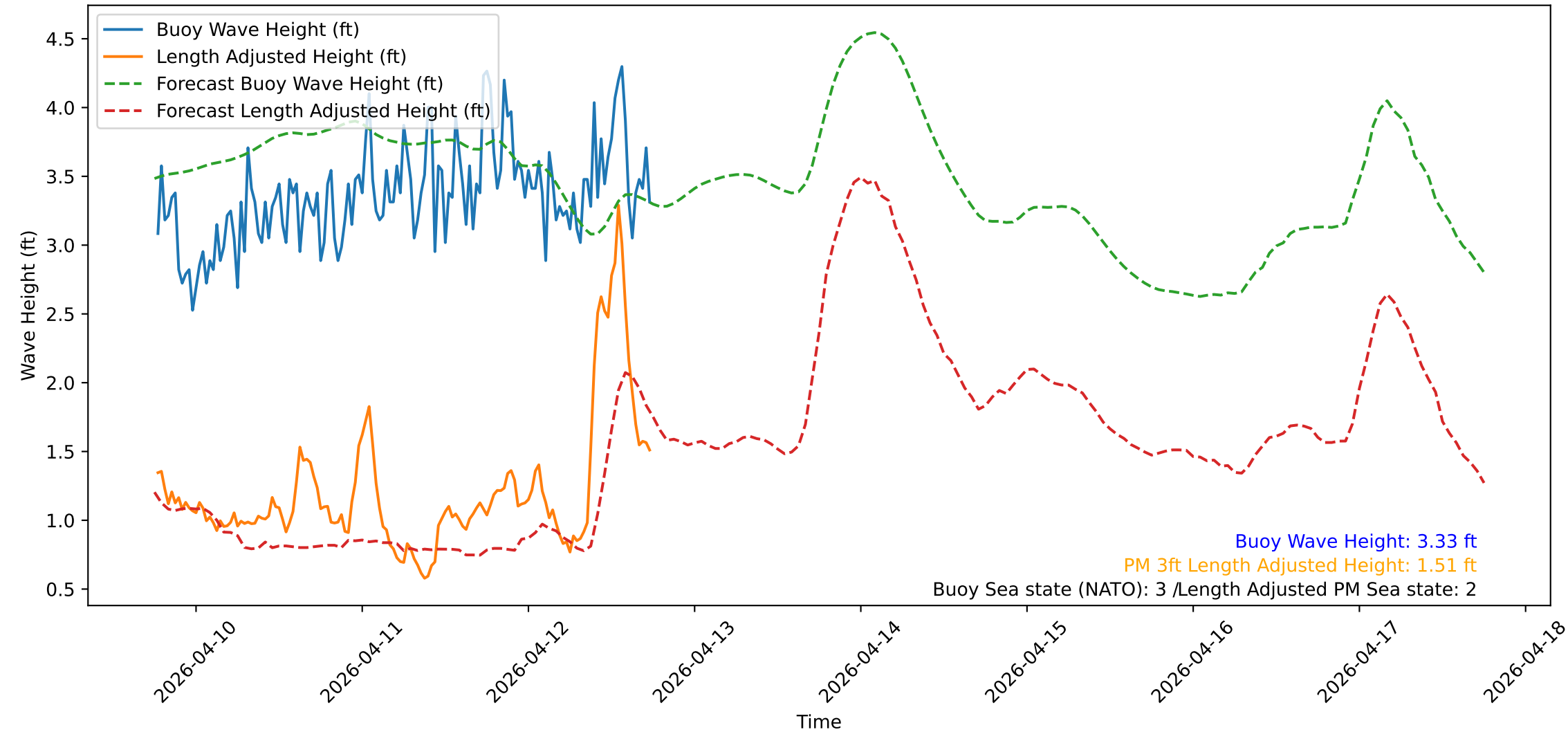
Wave Heights over Time for Red Beach at 2026-04-12 18:10:49
