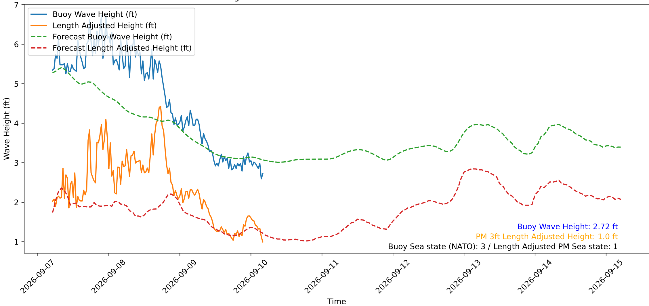
Wave Heights over Time for Red Beach at 2026-09-10 04:50:50
