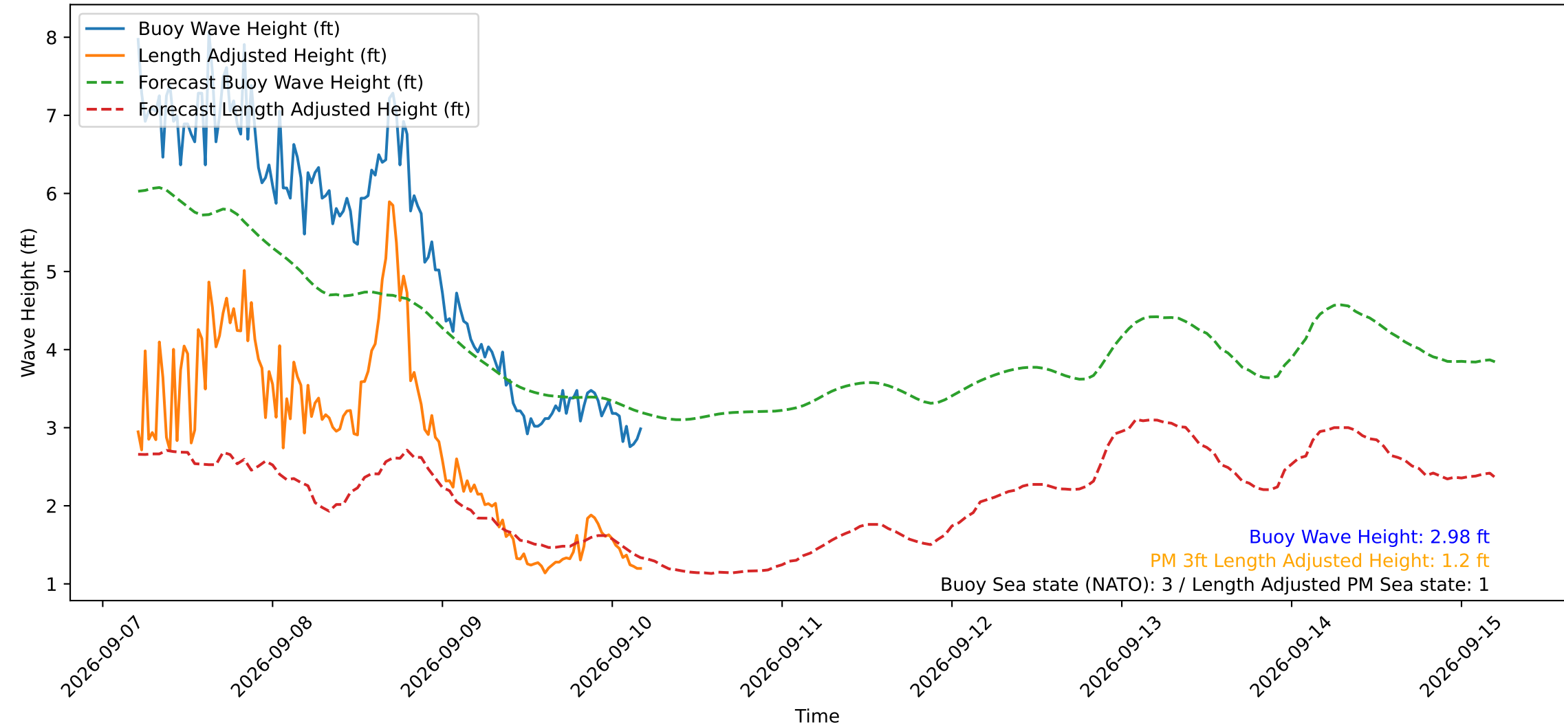
Wave Heights over Time for Green Beach at 2026-09-10 04:51:14
