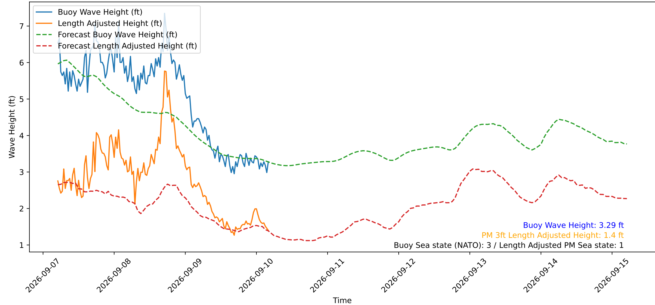
Wave Heights over Time for Oceanside Harbor at 2026-09-10 04:50:29
