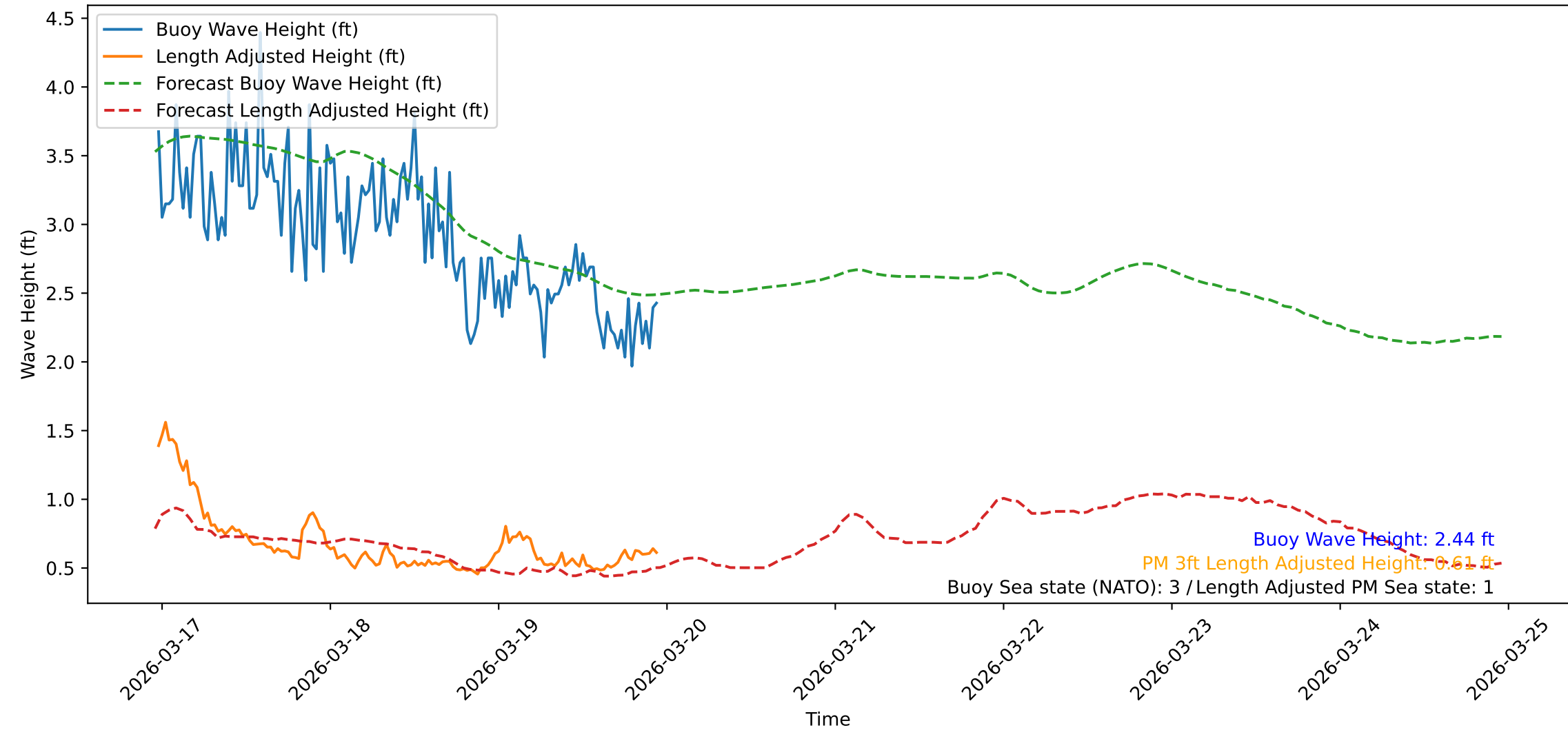
Wave Heights over Time for Oceanside Harbor at 2026-03-19 23:20:31
