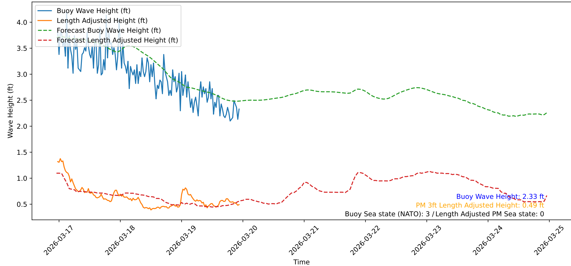
Wave Heights over Time for Green Beach at 2026-03-19 23:21:09
