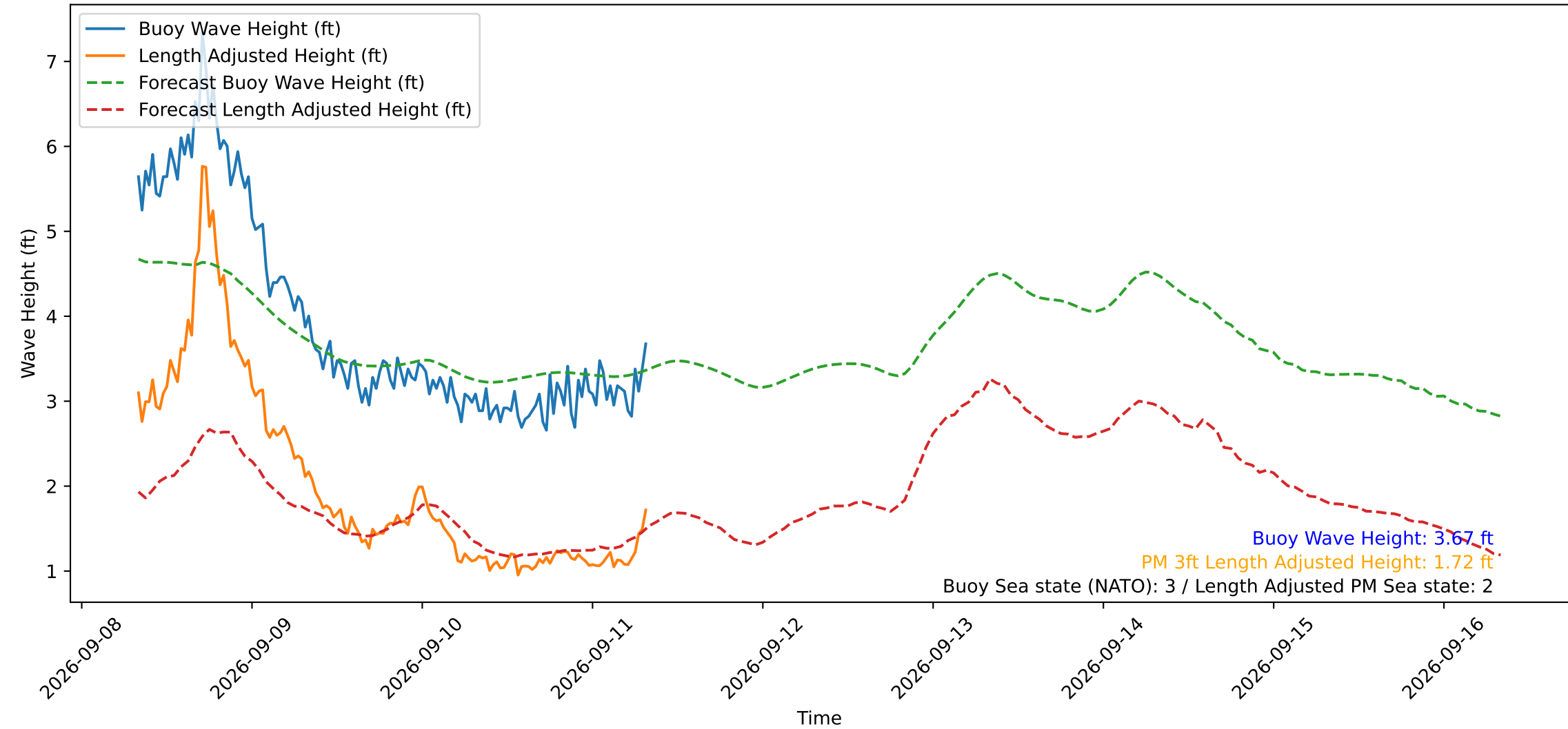
Wave Heights over Time for Oceanside Harbor at 2026-09-11 08:10:30
