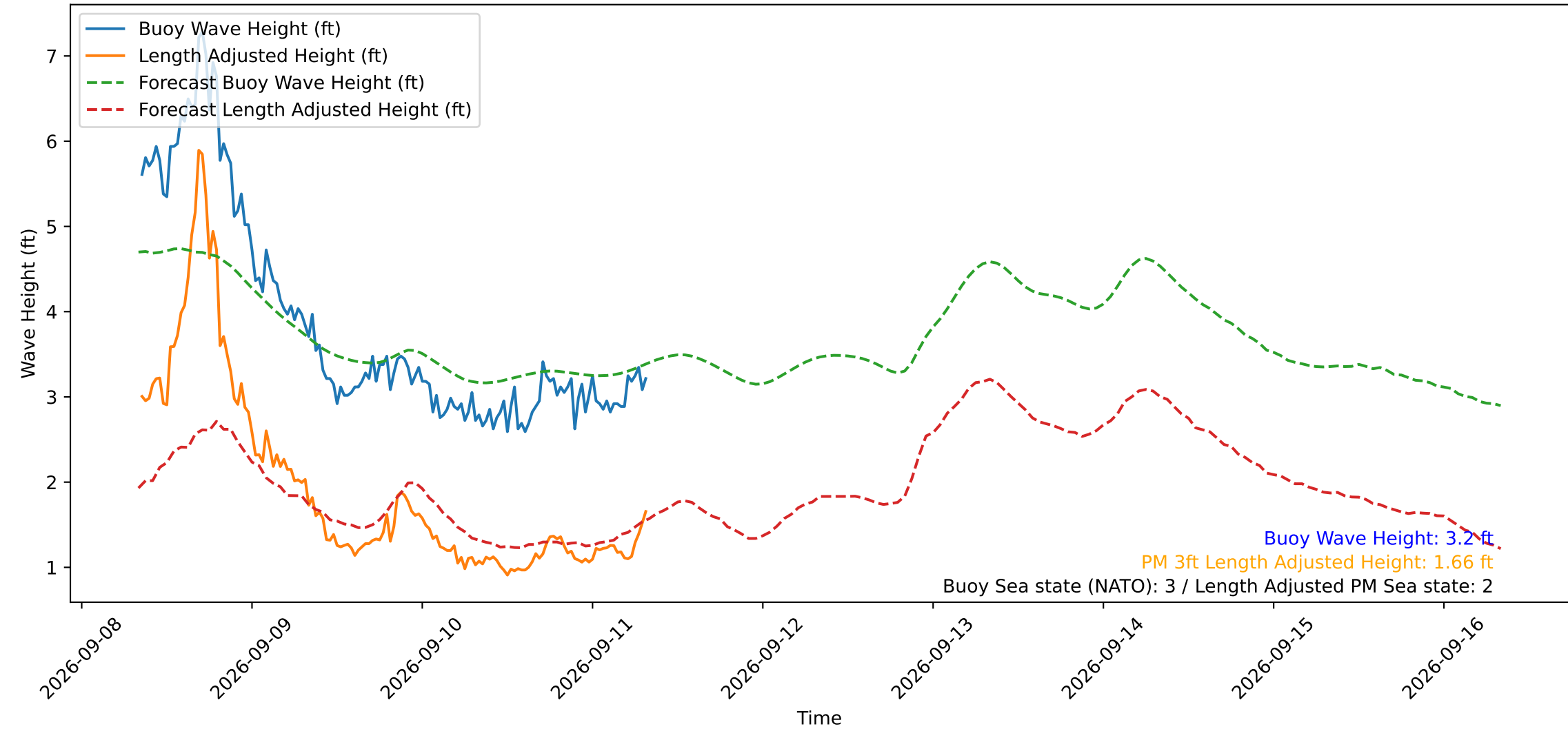
Wave Heights over Time for Green Beach at 2026-09-11 08:11:12
