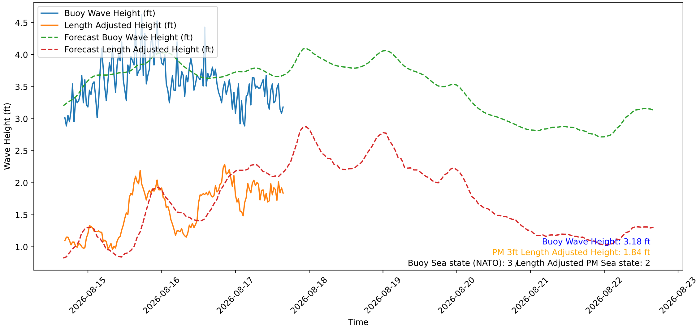
Wave Heights over Time for Oceanside Harbor at 2026-08-17 16:20:26
