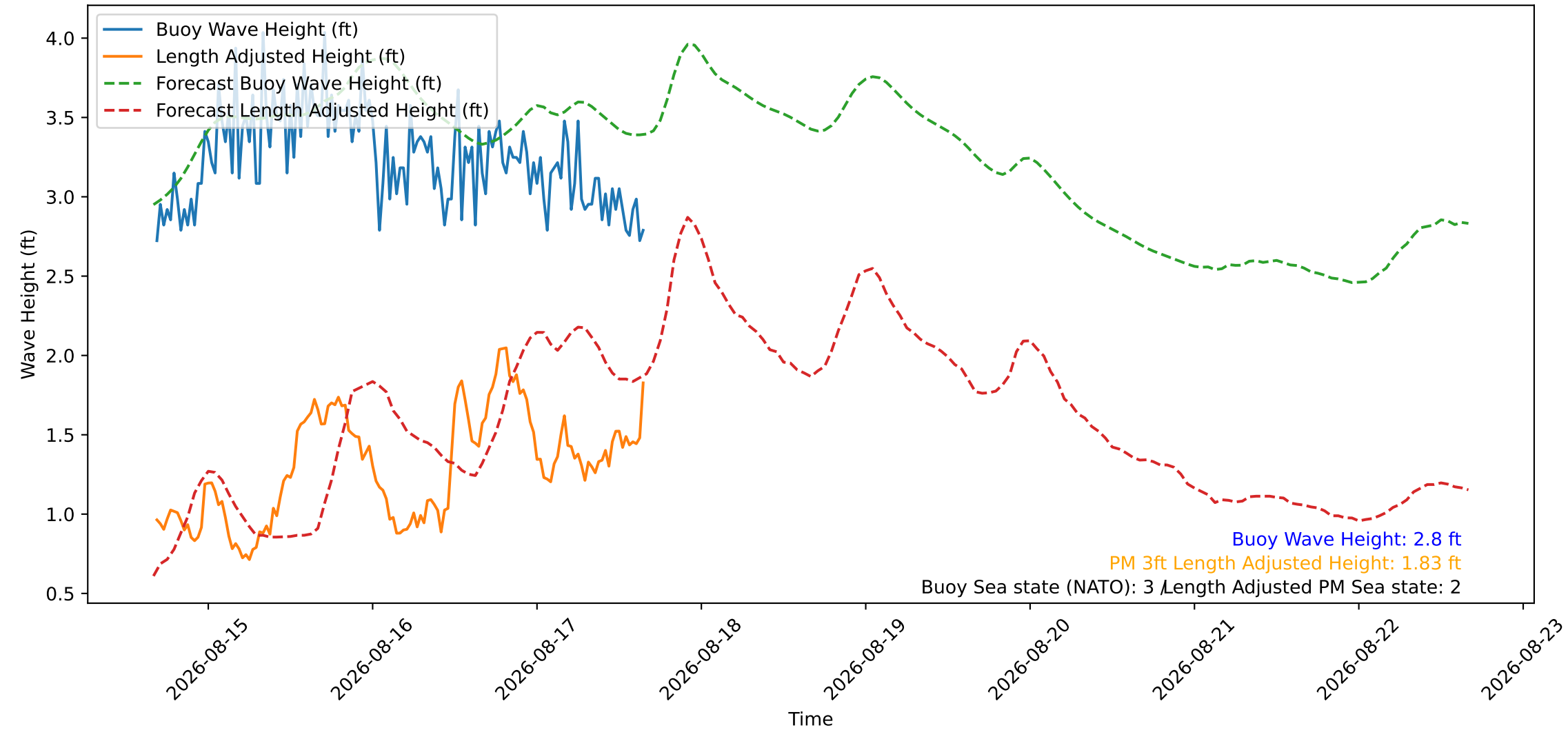
Wave Heights over Time for Red Beach at 2026-08-17 16:20:47
