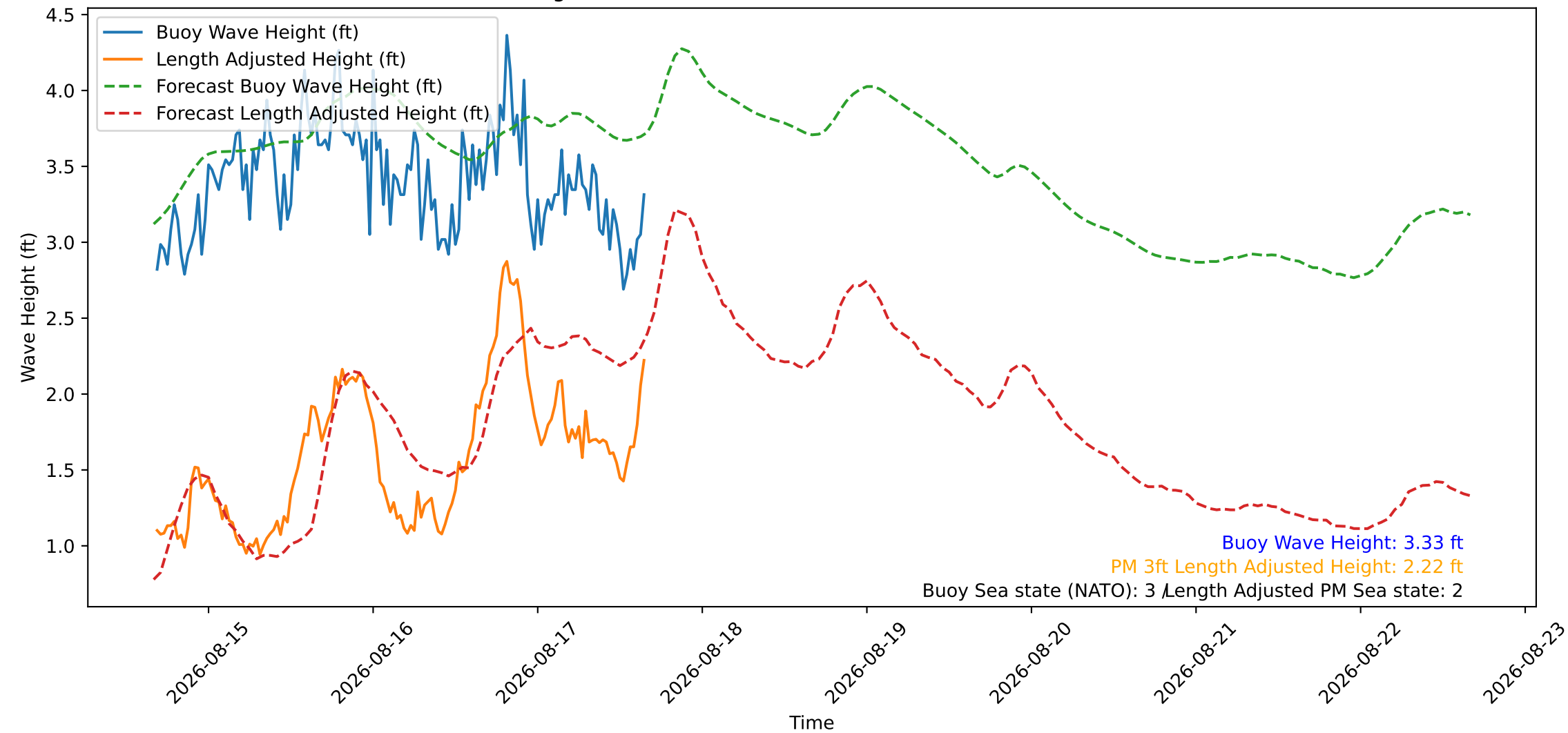
Wave Heights over Time for Green Beach at 2026-08-17 16:21:11
