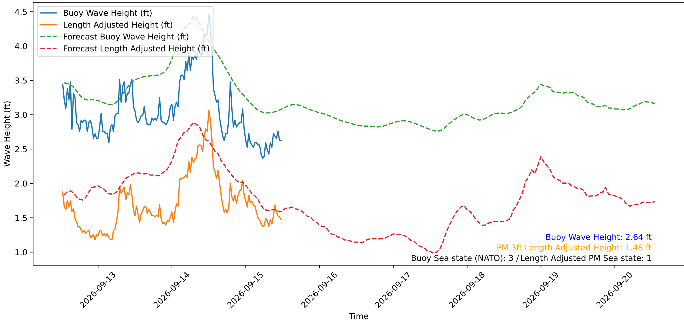
Wave Heights over Time for Oceanside Harbor at 2026-09-15 12:30:29
