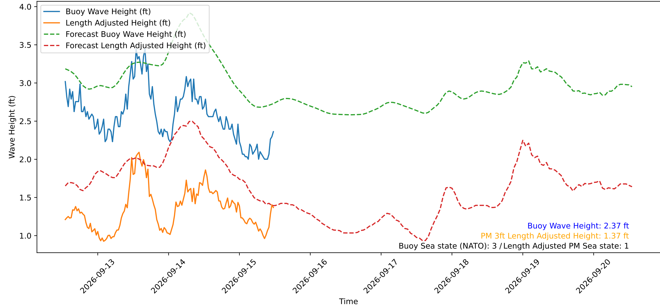
Wave Heights over Time for Red Beach at 2026-09-15 12:30:49
