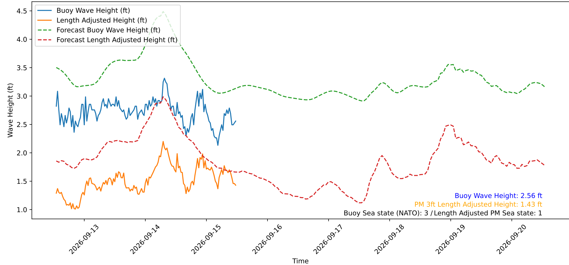
Wave Heights over Time for Green Beach at 2026-09-15 12:31:11
