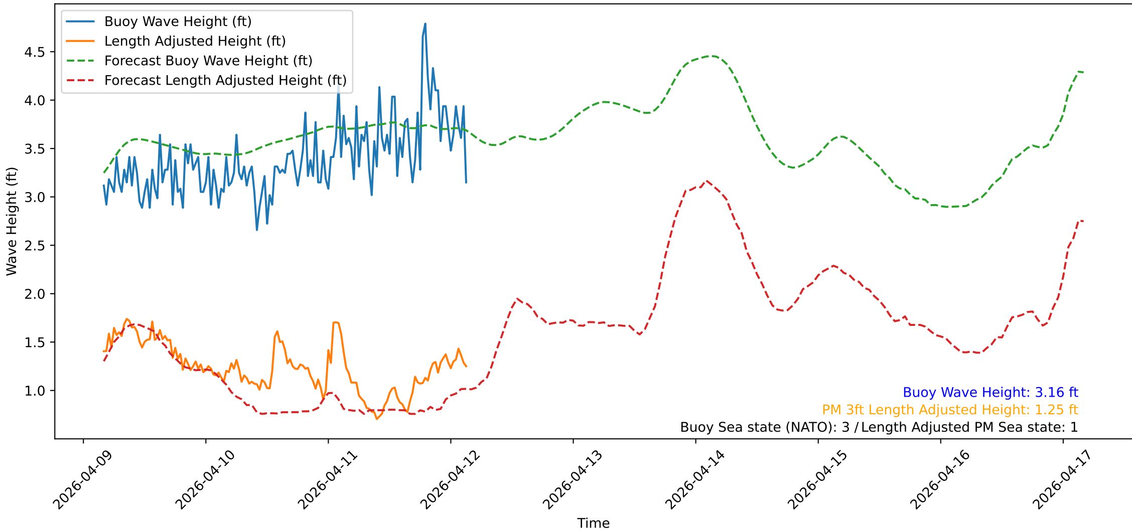
Wave Heights over Time for Oceanside Harbor at 2026-04-12 04:00:31
