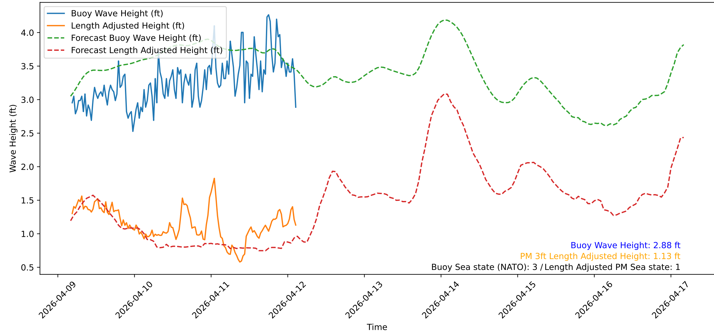
Wave Heights over Time for Red Beach at 2026-04-12 04:00:50
