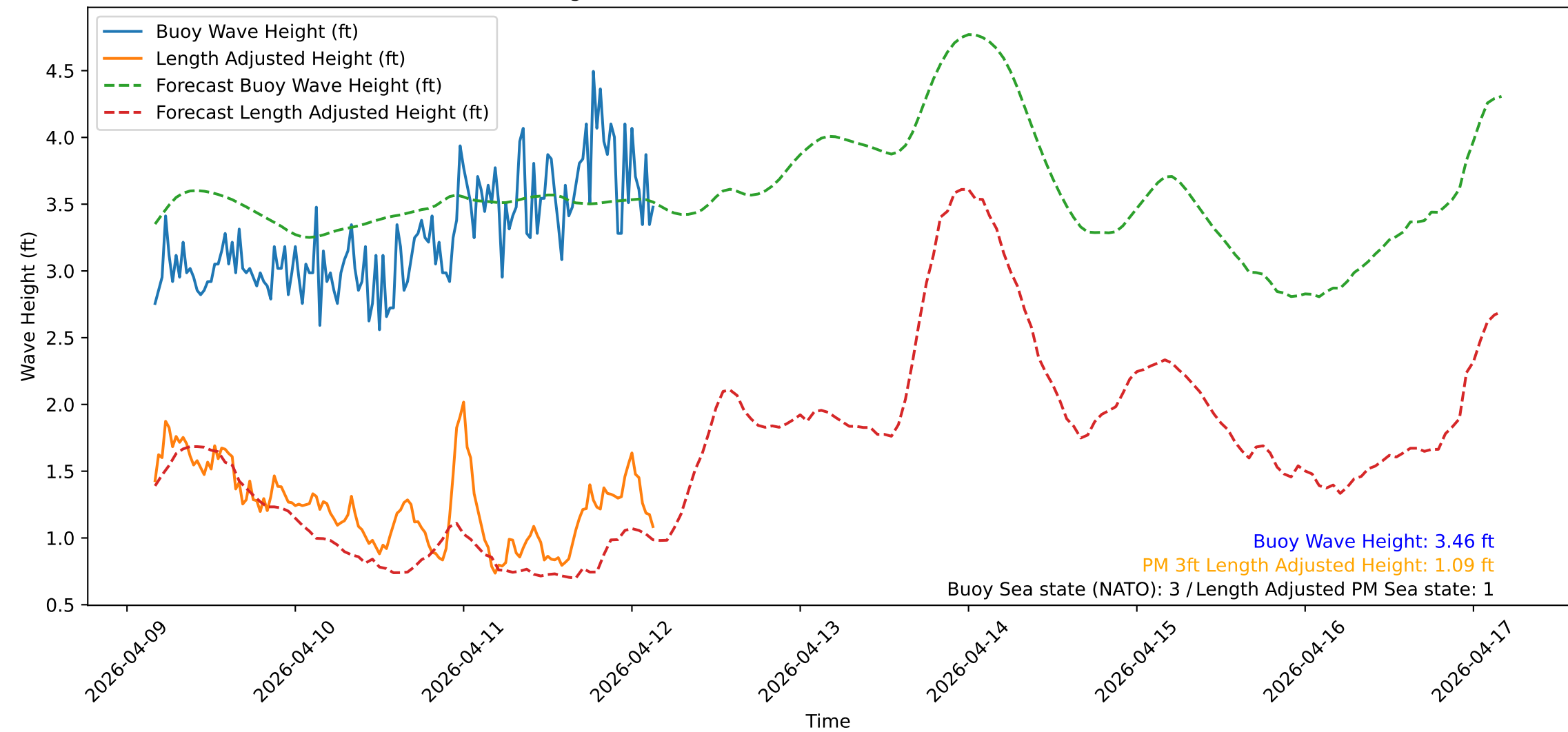
Wave Heights over Time for Green Beach at 2026-04-12 04:01:12
