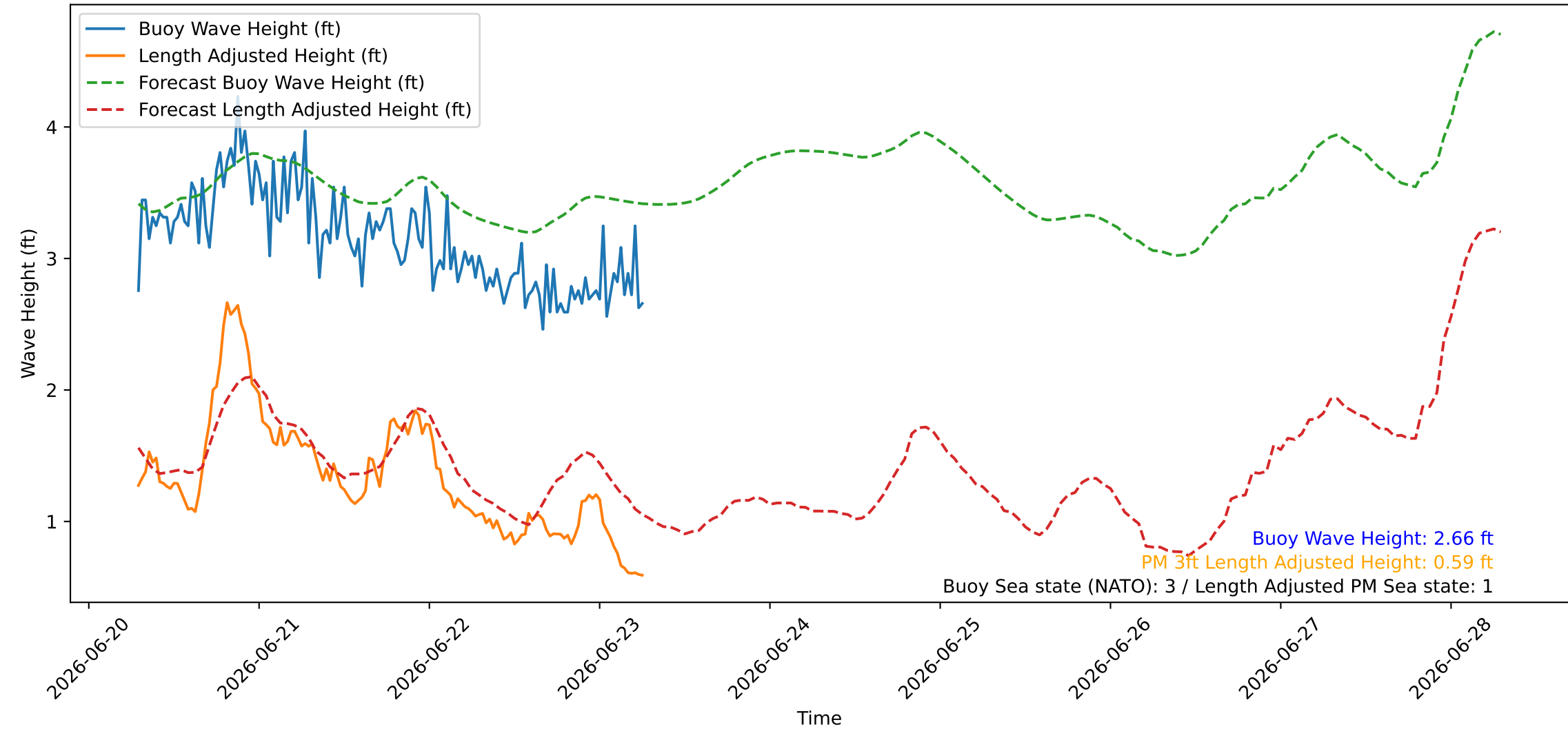
Wave Heights over Time for Green Beach at 2026-06-23 07:01:08
