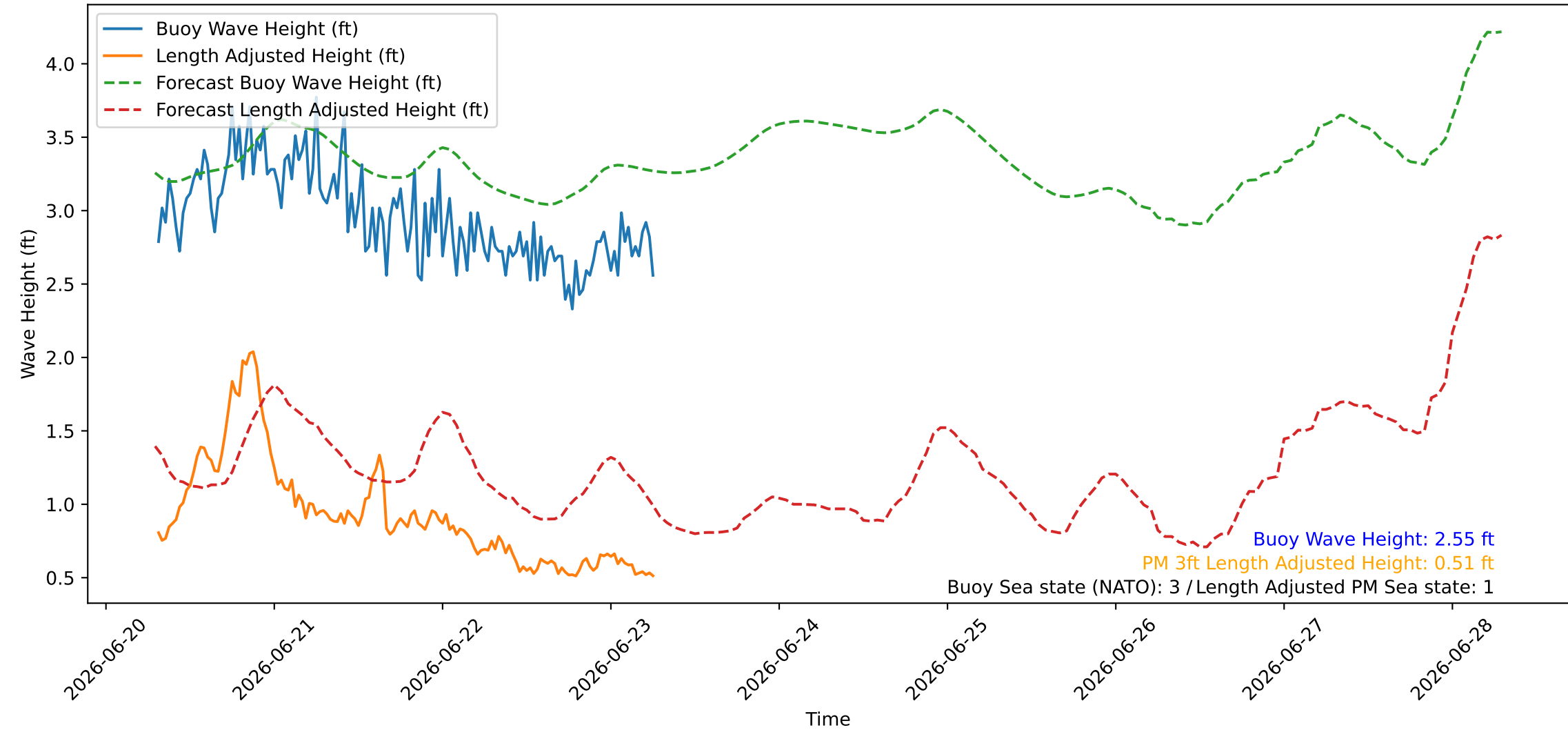
Wave Heights over Time for Red Beach at 2026-06-23 07:00:46
