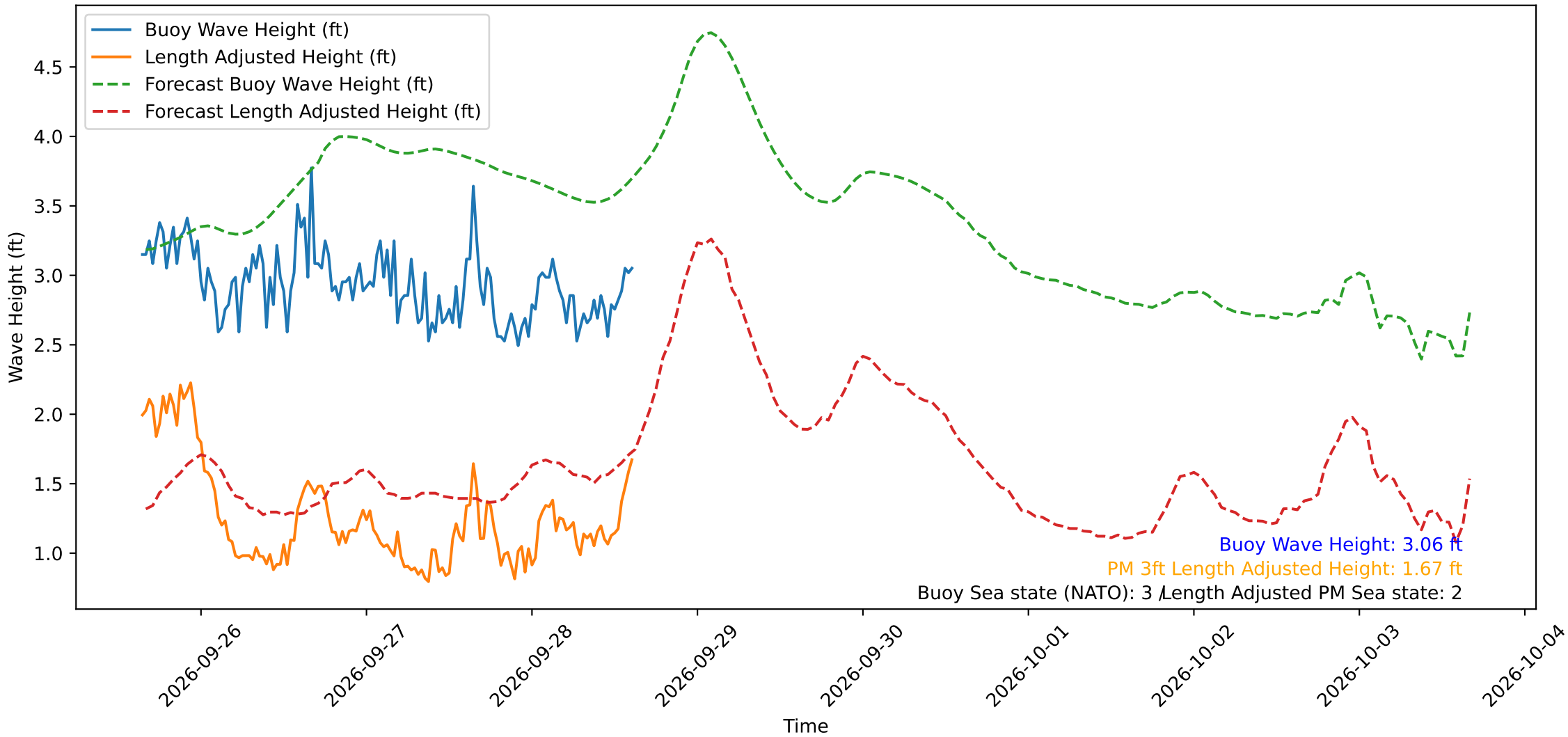
Wave Heights over Time for Oceanside Harbor at 2026-09-28 15:40:29
