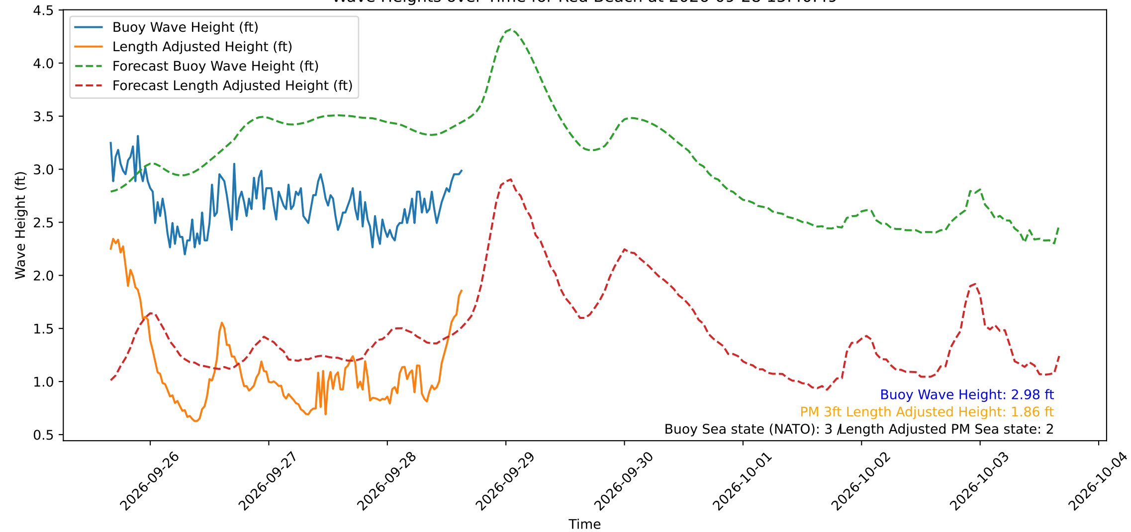
Wave Heights over Time for Red Beach at 2026-09-28 15:40:49
