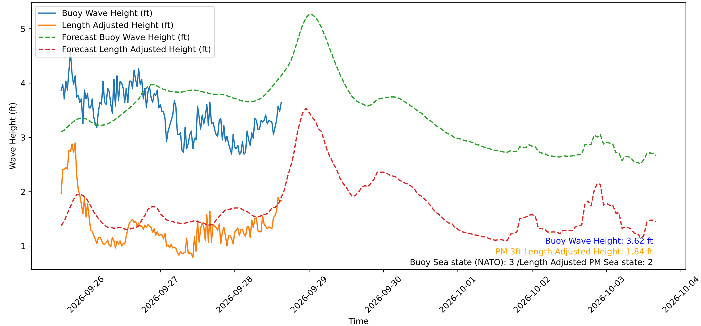
Wave Heights over Time for Green Beach at 2026-09-28 15:41:13
