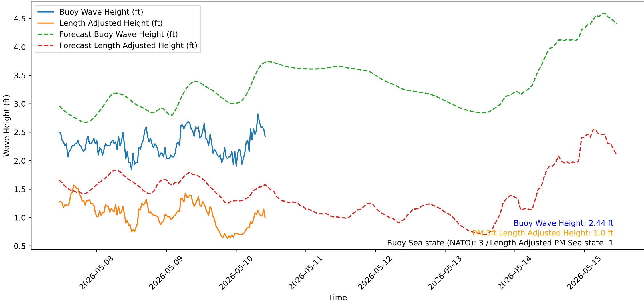
Wave Heights over Time for Green Beach at 2026-05-10 11:01:14
