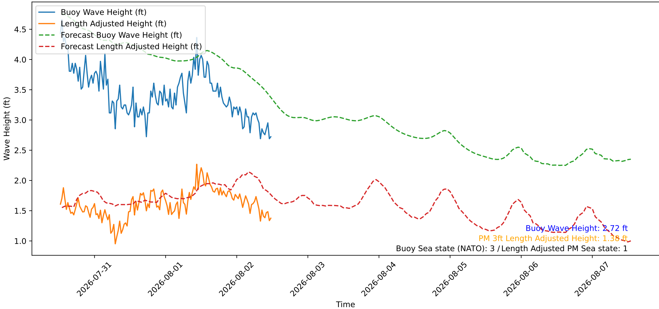
Wave Heights over Time for Oceanside Harbor at 2026-08-02 12:30:26
