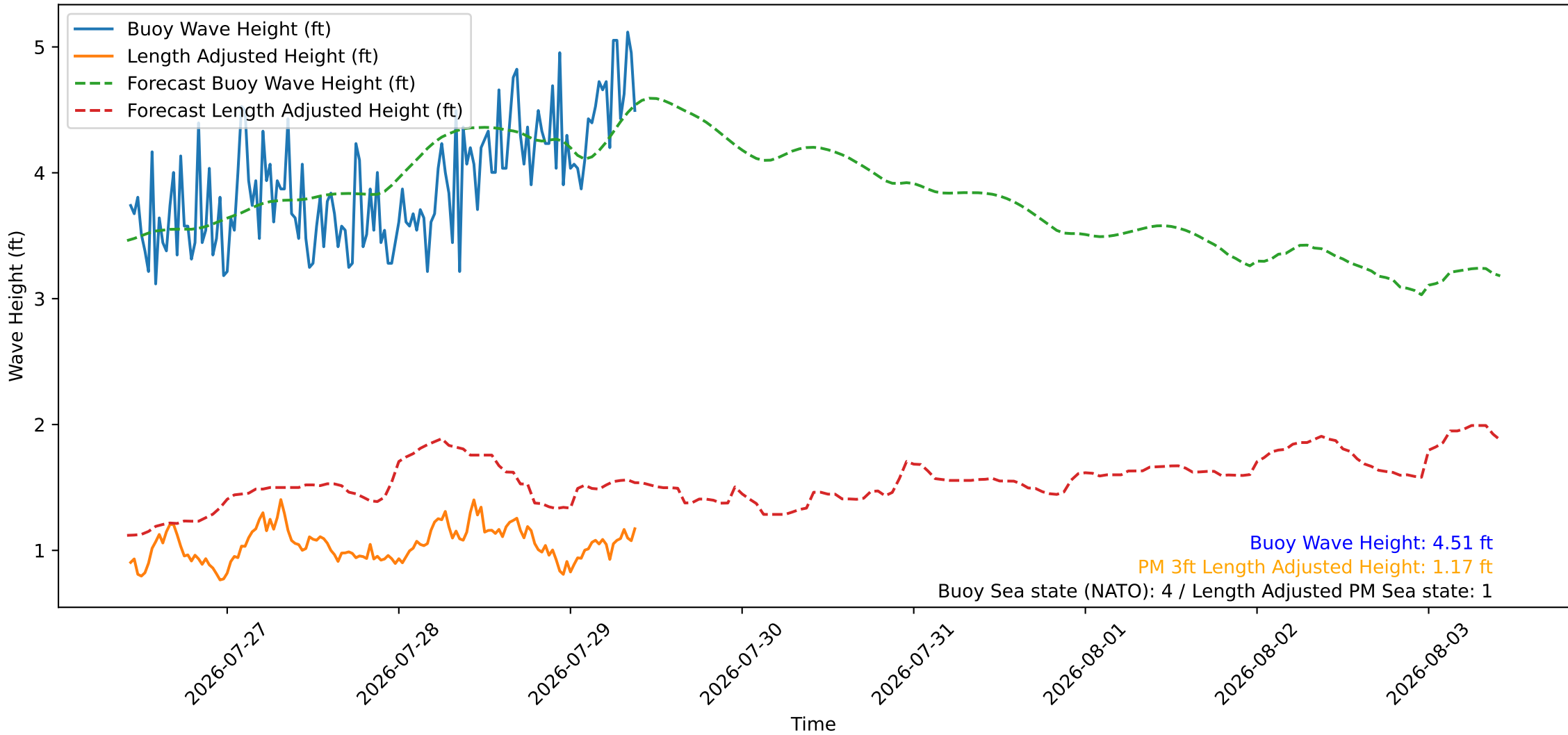
Wave Heights over Time for Red Beach at 2026-07-29 10:00:46
