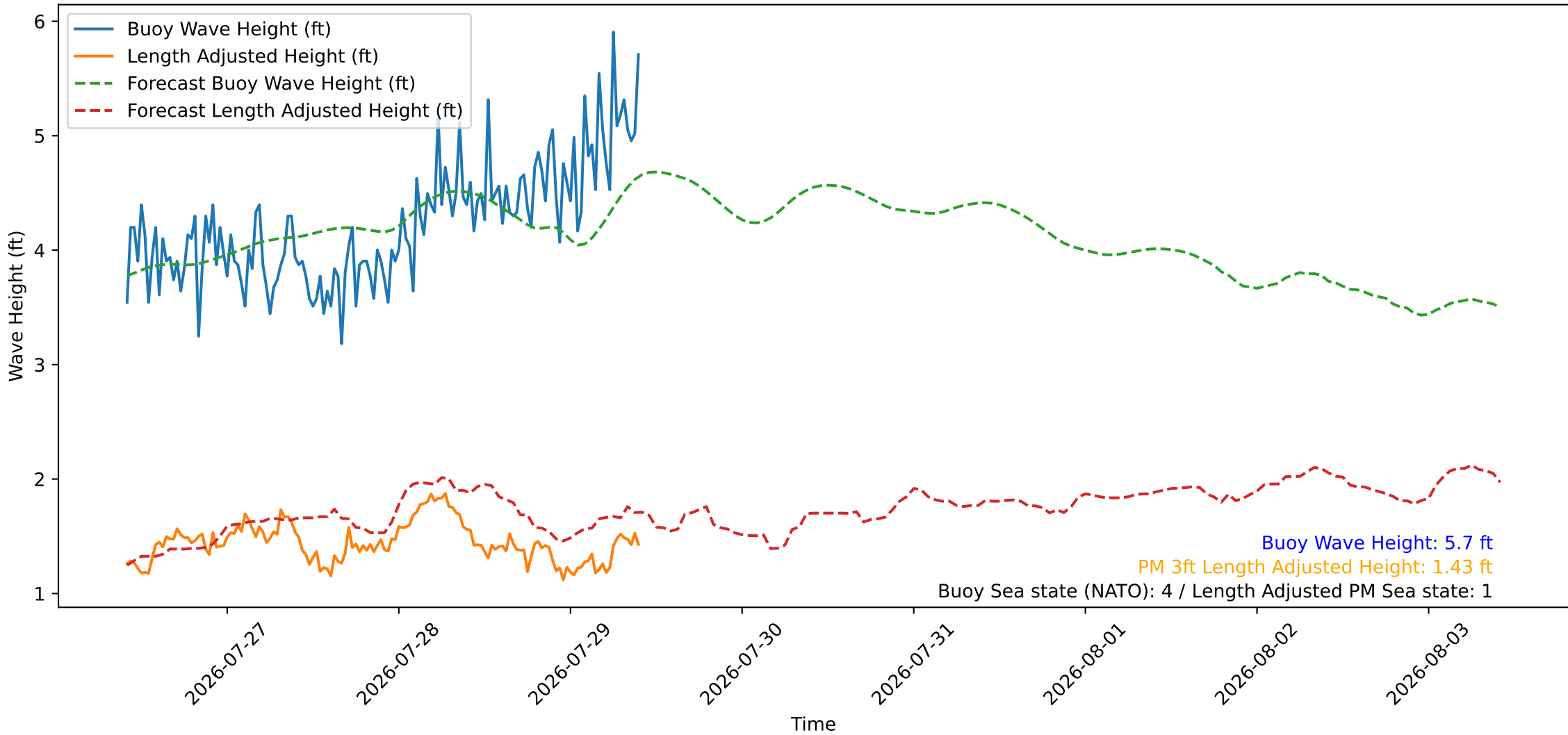
Wave Heights over Time for Oceanside Harbor at 2026-07-29 10:00:26
