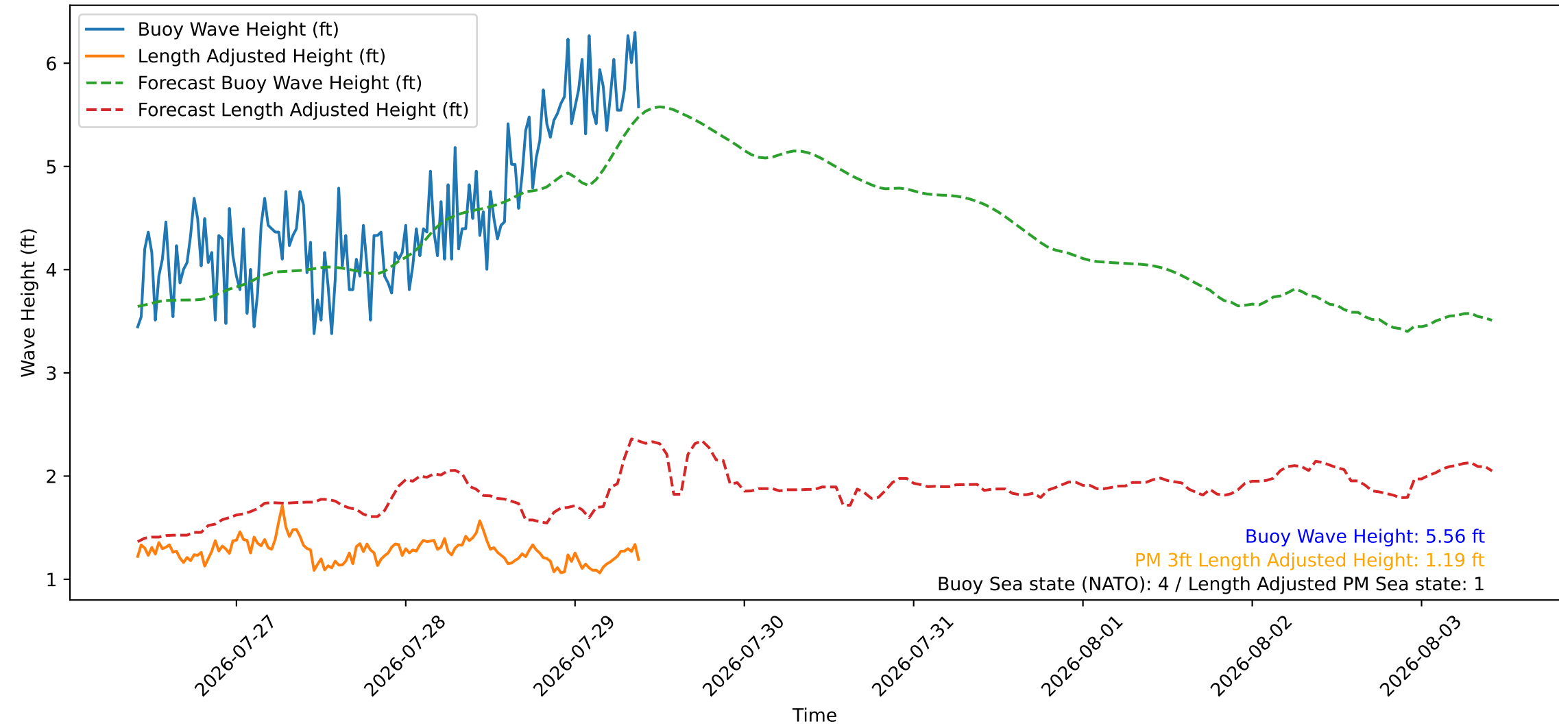
Wave Heights over Time for Green Beach at 2026-07-29 10:01:08
