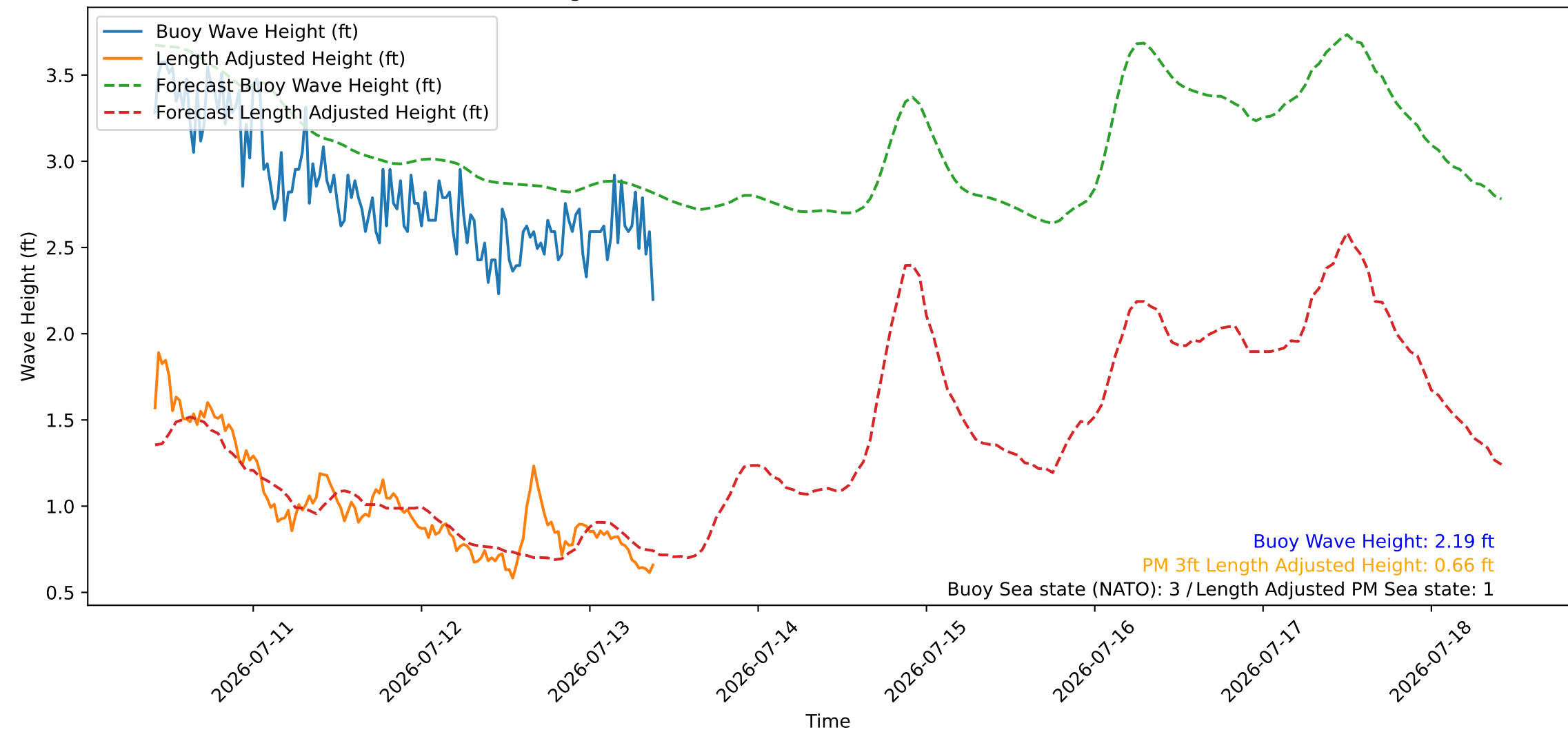
Wave Heights over Time for Green Beach at 2026-07-13 10:01:07
