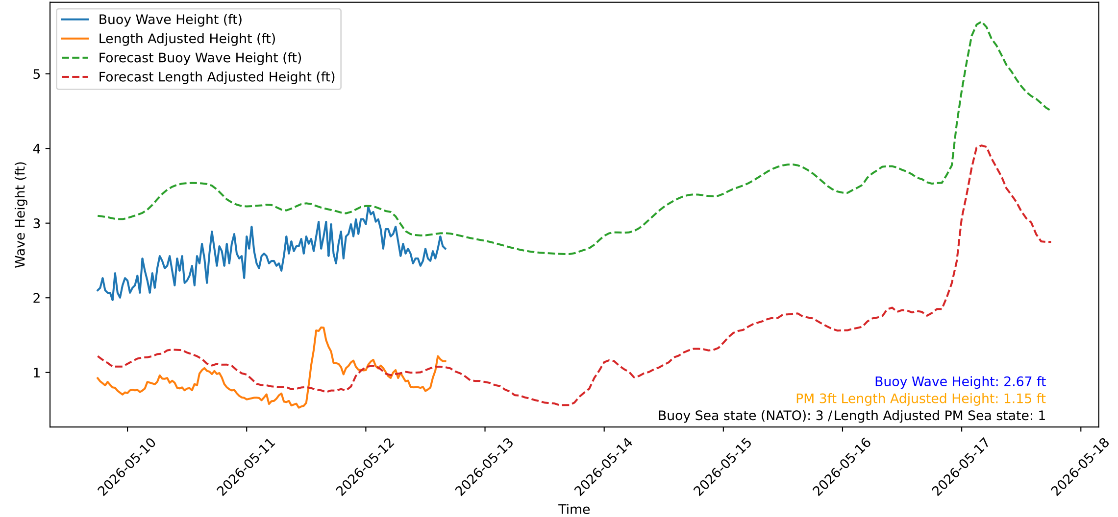
Wave Heights over Time for Red Beach at 2026-05-12 17:30:51
