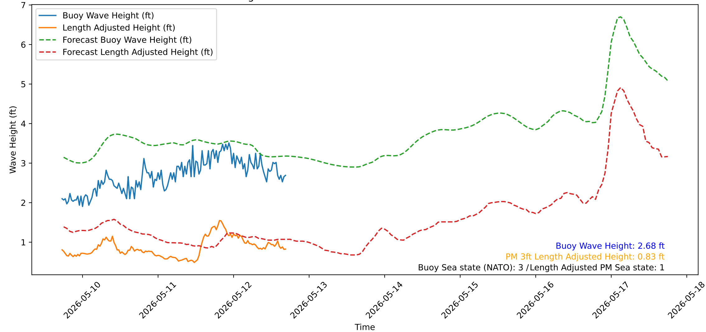
Wave Heights over Time for Green Beach at 2026-05-12 17:31:14
