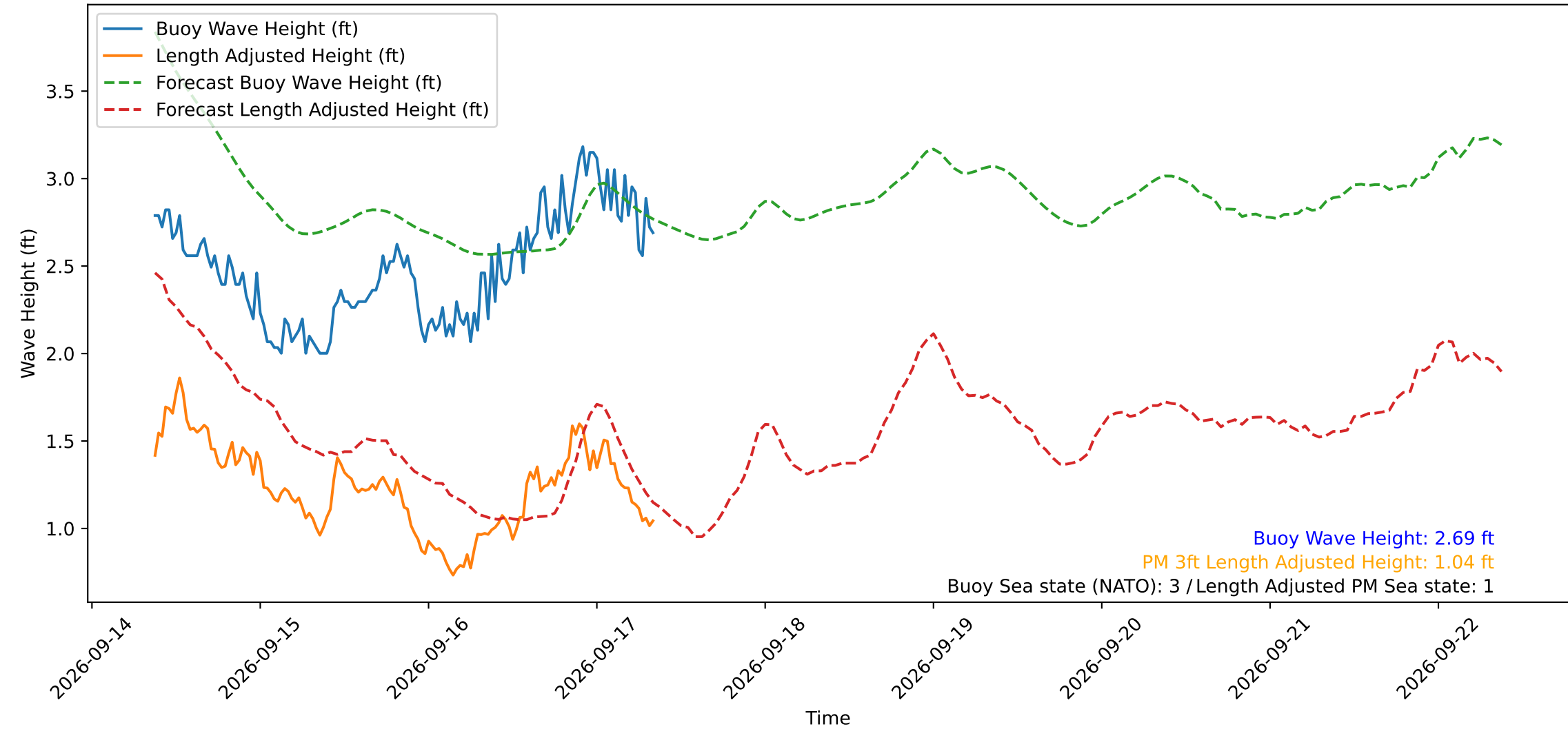
Wave Heights over Time for Red Beach at 2026-09-17 08:50:51
