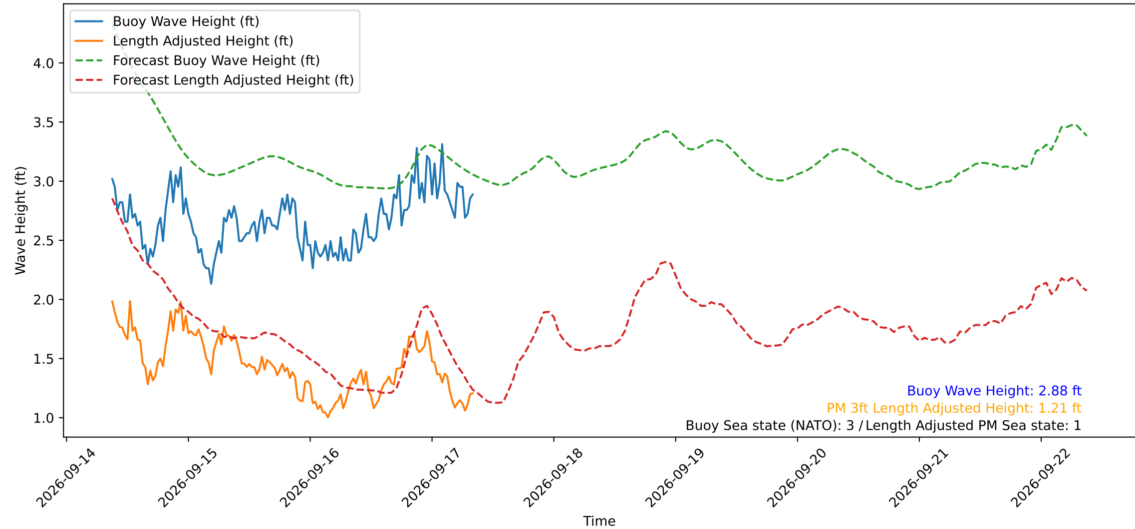
Wave Heights over Time for Green Beach at 2026-09-17 08:51:15
