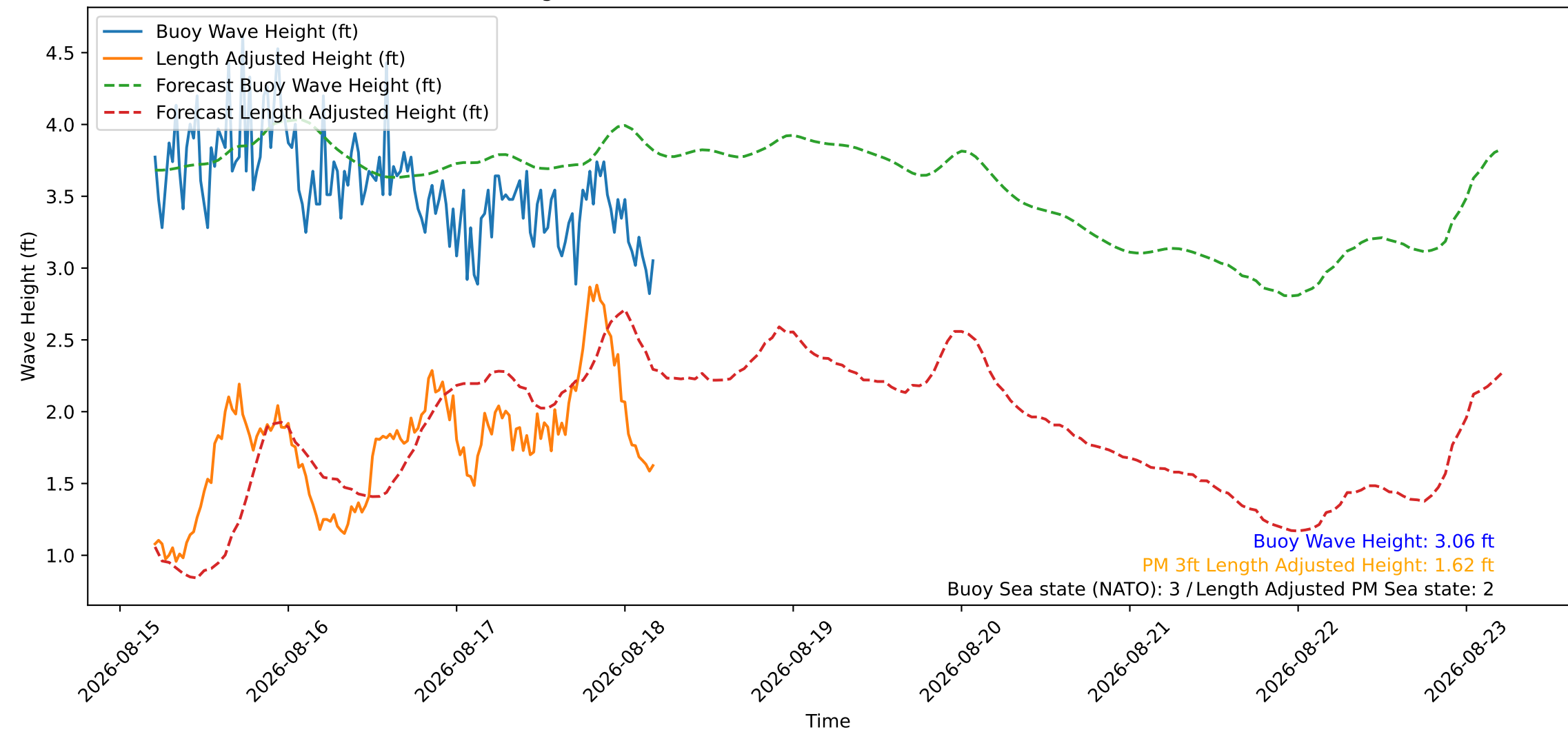
Wave Heights over Time for Oceanside Harbor at 2026-08-18 04:50:27
