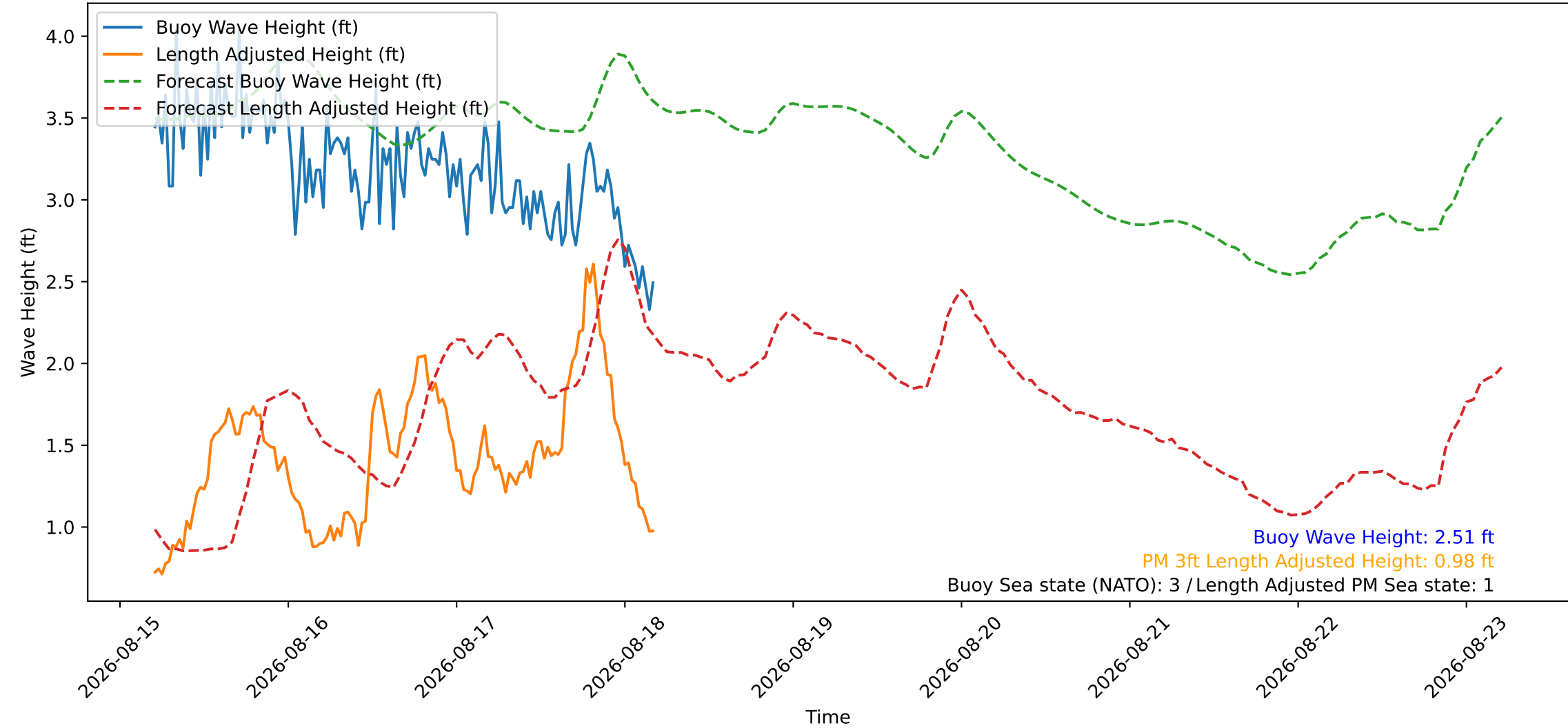
Wave Heights over Time for Red Beach at 2026-08-18 04:50:47
