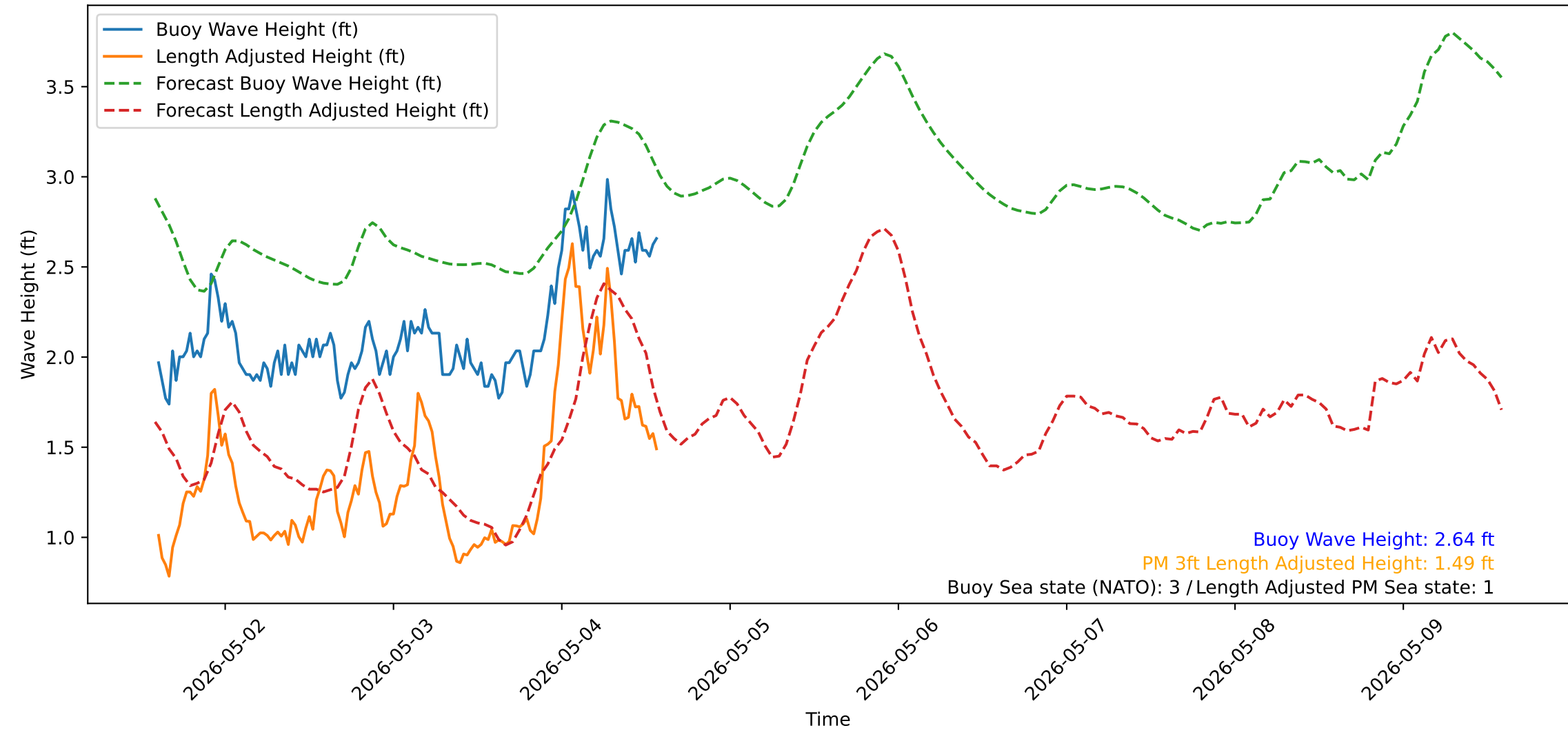
Wave Heights over Time for Green Beach at 2026-05-04 14:21:14
