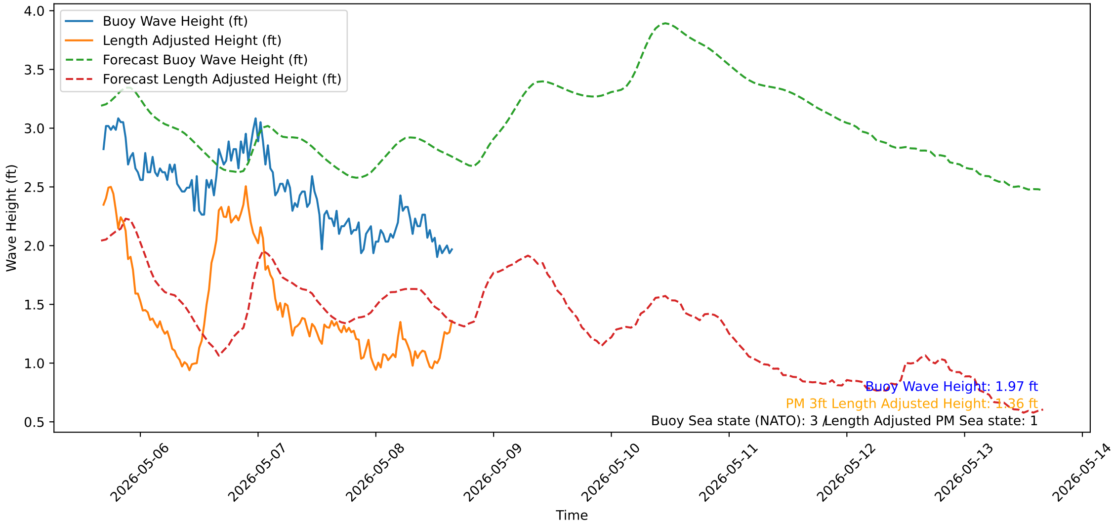
Wave Heights over Time for Red Beach at 2026-05-08 16:20:52
