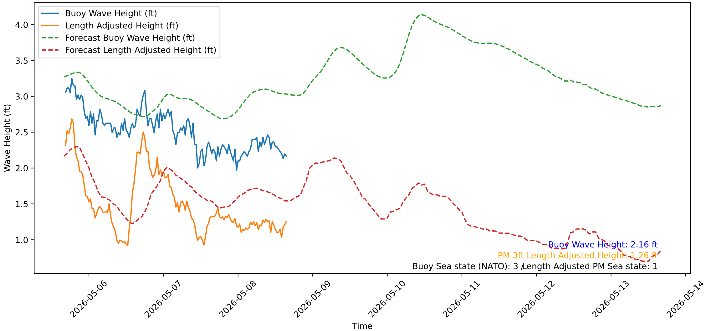
Wave Heights over Time for Oceanside Harbor at 2026-05-08 16:20:31
