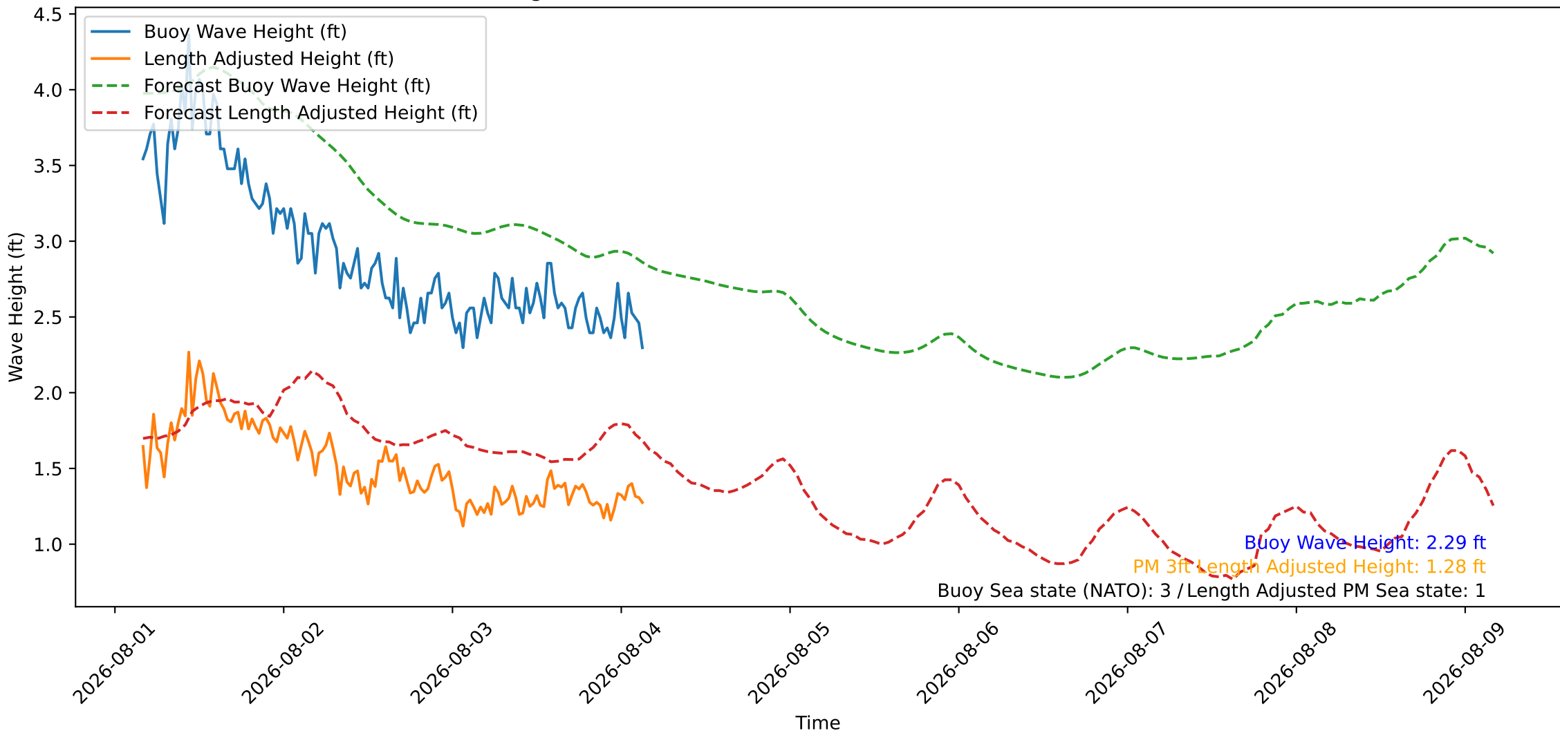
Wave Heights over Time for Oceanside Harbor at 2026-08-04 03:50:26
