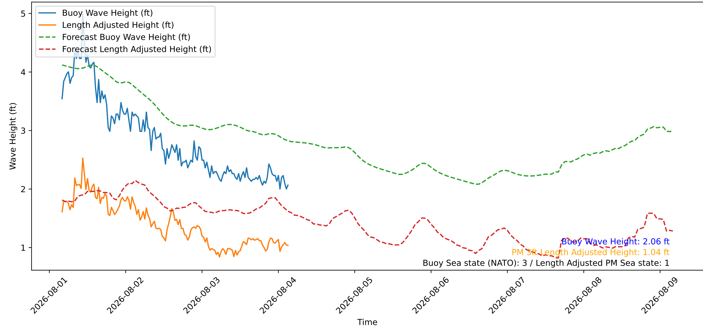
Wave Heights over Time for Green Beach at 2026-08-04 03:51:09
