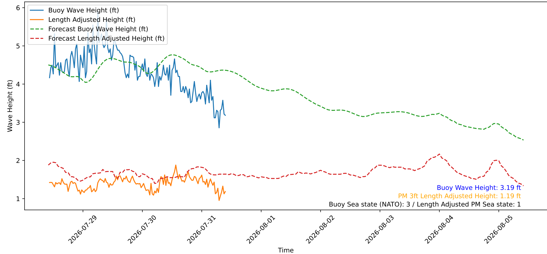
Wave Heights over Time for Oceanside Harbor at 2026-07-31 10:20:27
