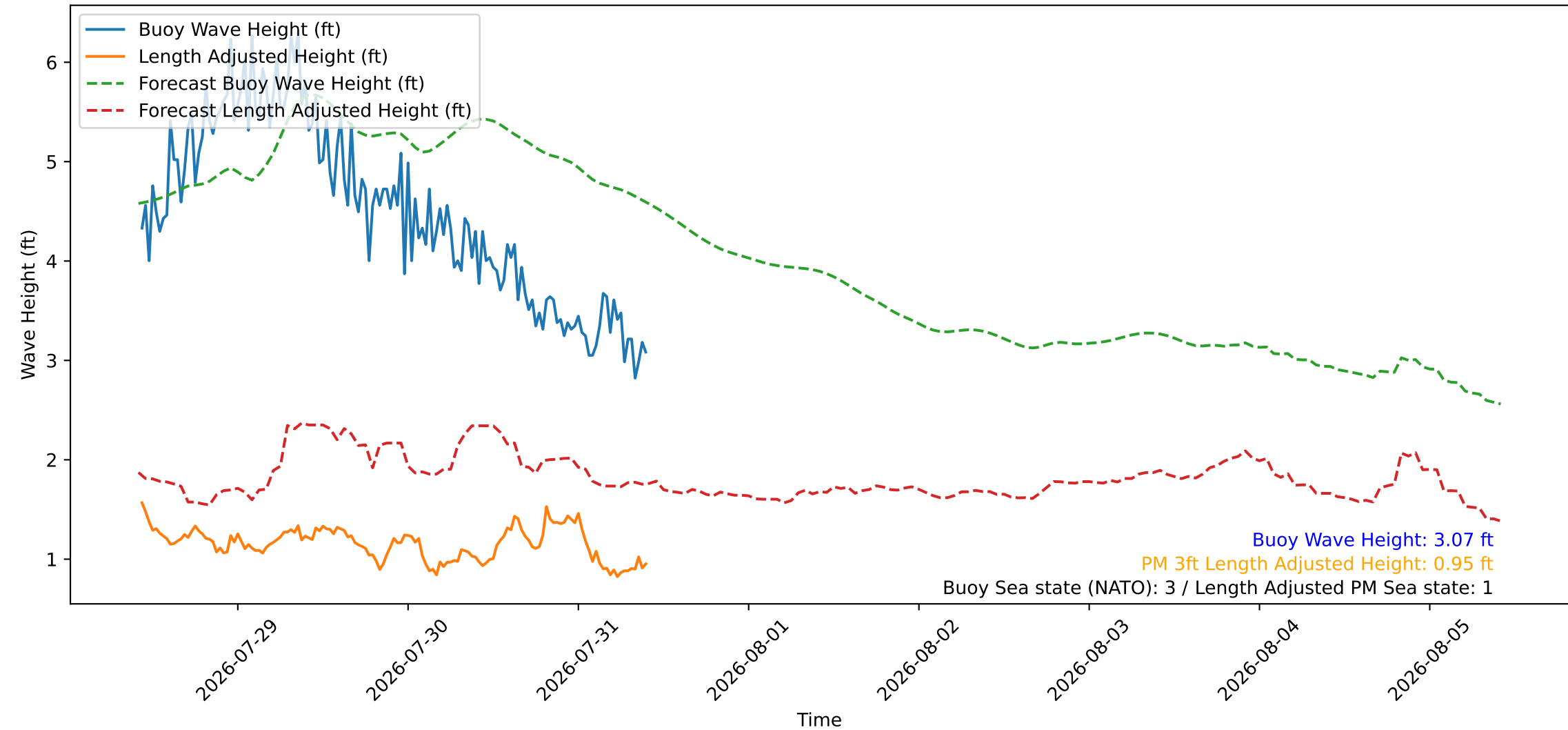
Wave Heights over Time for Green Beach at 2026-07-31 10:21:11
