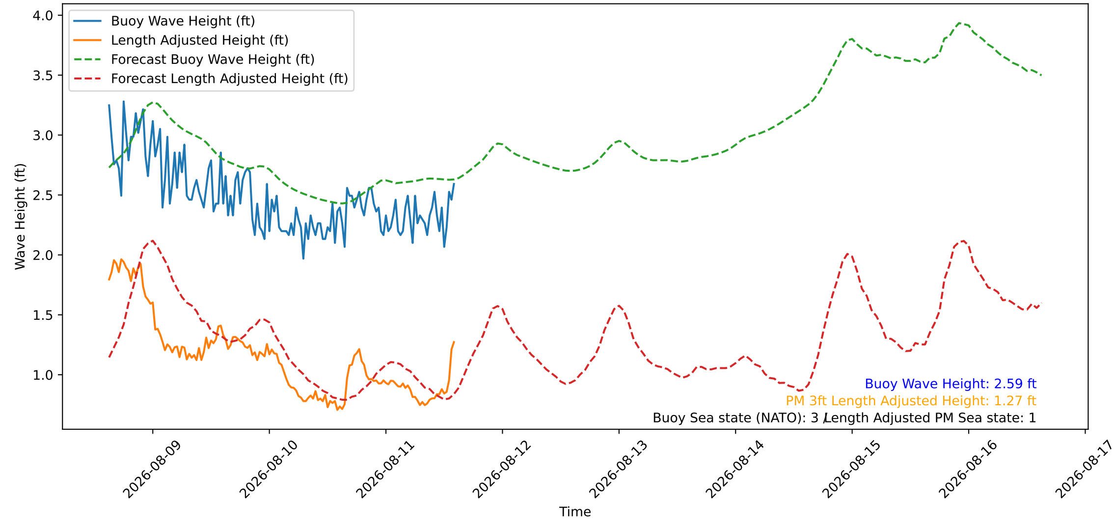
Wave Heights over Time for Oceanside Harbor at 2026-08-11 15:00:26
