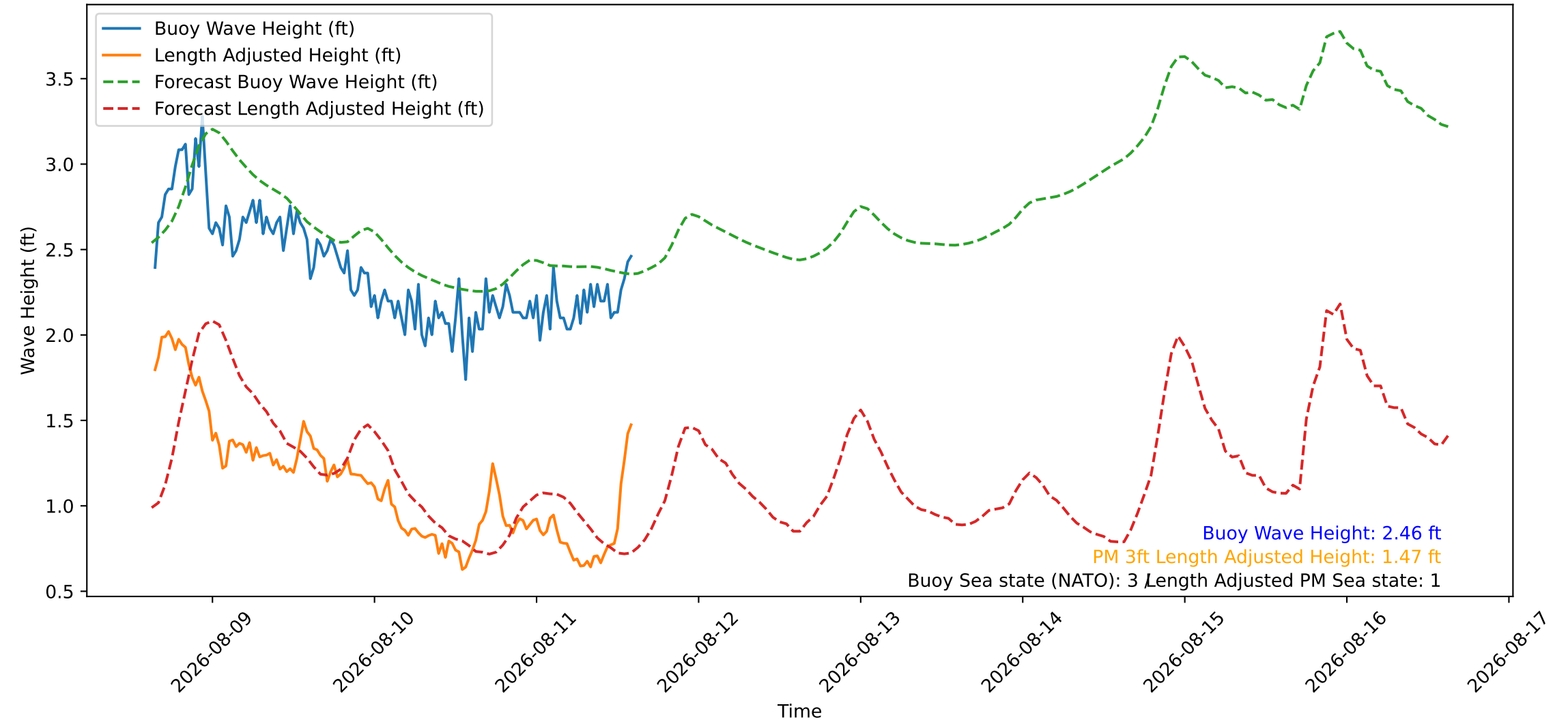
Wave Heights over Time for Red Beach at 2026-08-11 15:00:47
