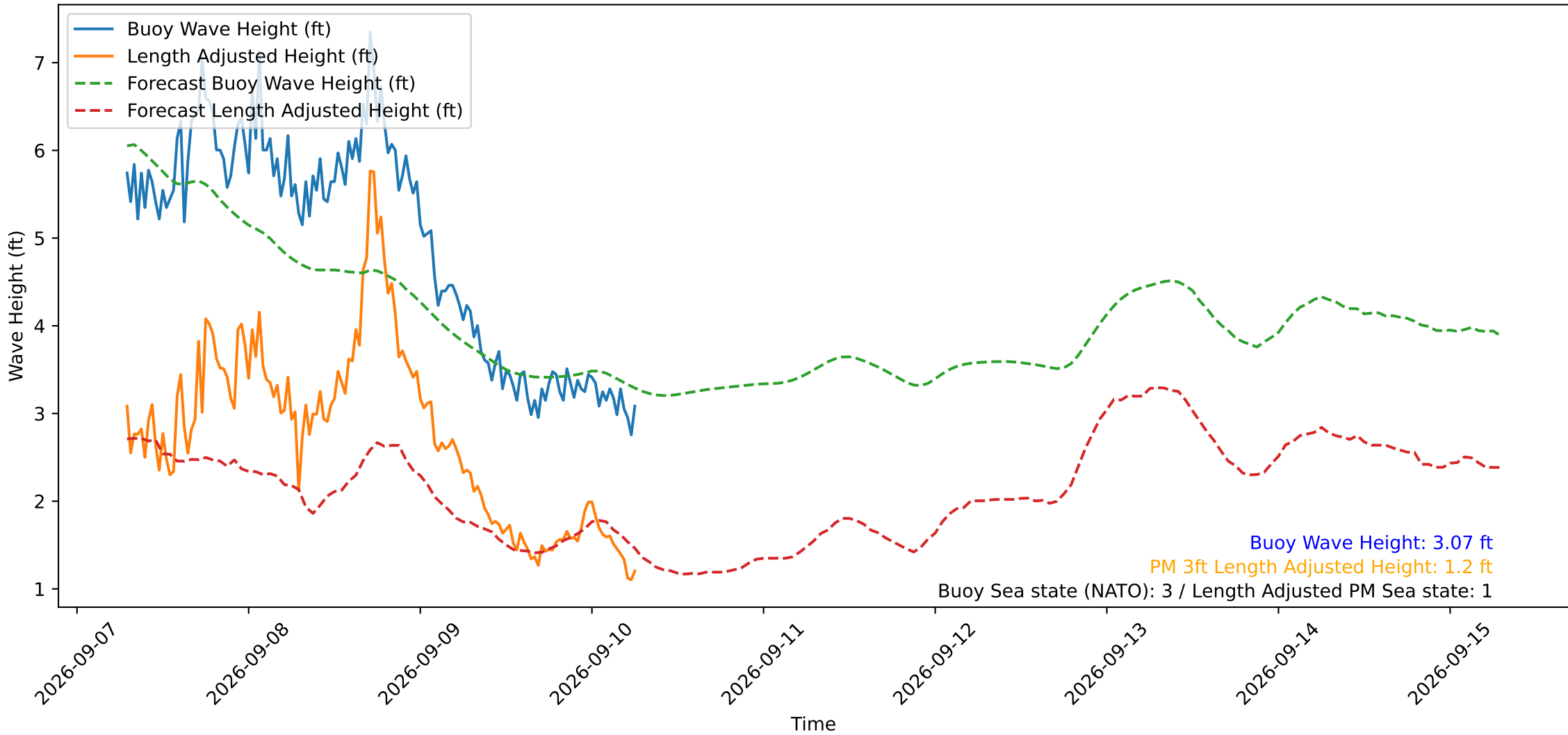
Wave Heights over Time for Oceanside Harbor at 2026-09-10 06:50:29
