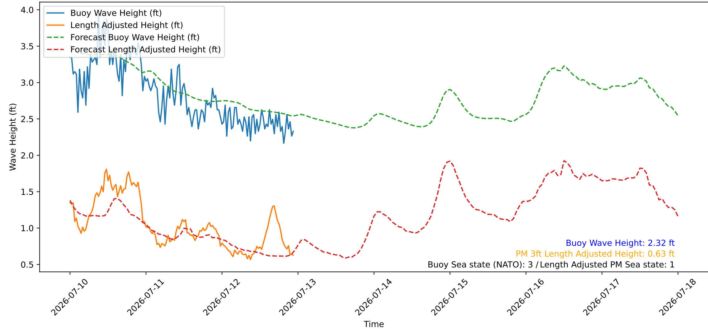
Wave Heights over Time for Red Beach at 2026-07-12 23:30:45
