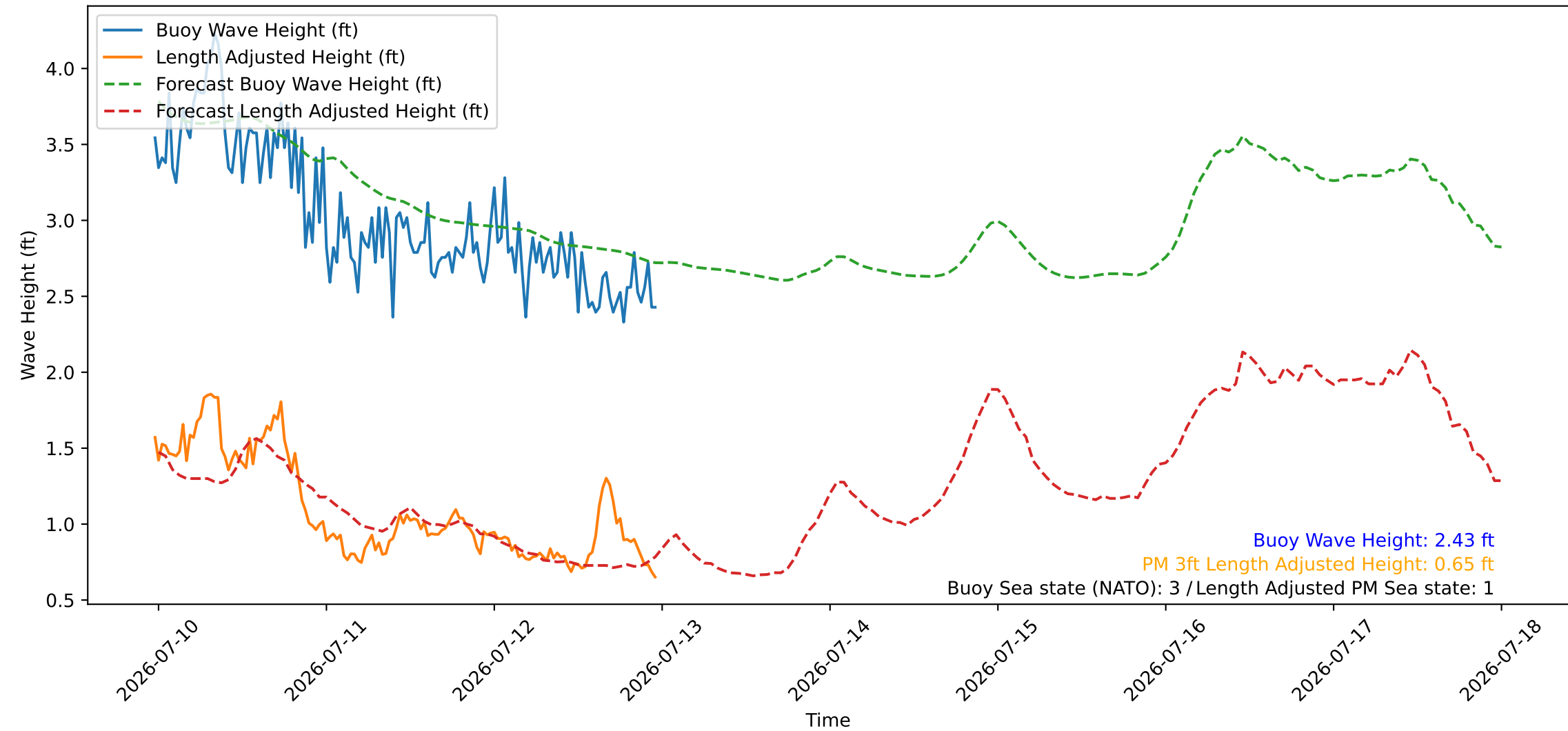
Wave Heights over Time for Oceanside Harbor at 2026-07-12 23:30:26
